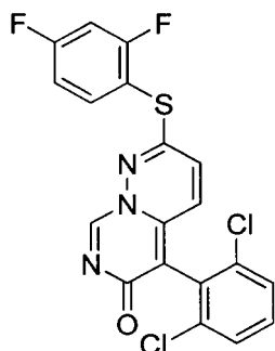
5-(2,6-dichlorophenyl)-2-(2,4-difluorophenylthio)-6H-pyrimido[1,6-b]pyridazin-6-one
