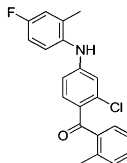
(2-chloro-4-(4-fluoro-2-methylphenylamino)phenyl)(o-tolyl)methanone
