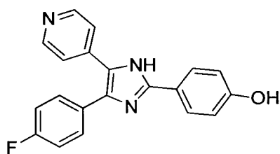
SB 202190
