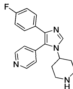
4-(4-(4-fluorophenyl)-1-(piperidin-4-yl)-1H-imidazol-5-yl)pyridine
