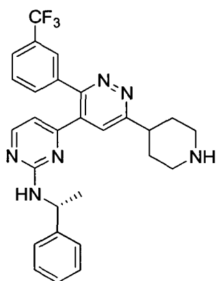
(R)-N-(1-phenylethyl)-4-(6-(piperidin-4-yl)-3-(3-(trifluoromethyl)phenyl)pyridazin-4-yl)pyrimidin-2-amine
