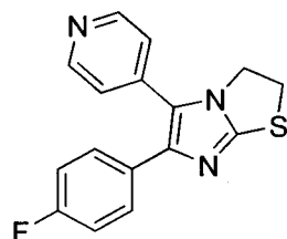
SKF 86002
