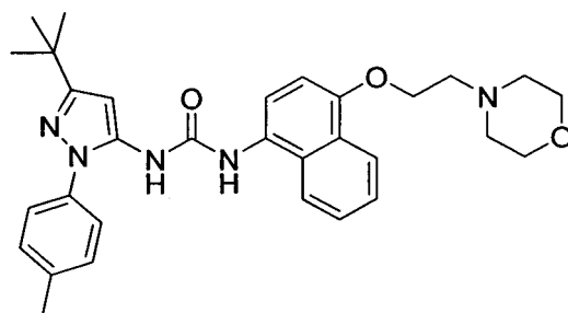
BIRB 796 (Doramapimod)
