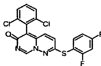
VX-745
