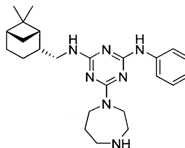
6-(1,4-diazepan-1-yl)-N²-(((1S,2R,5S)-6,6-dimethylbicyclo[3.1.1]heptan-2-yl)methyl)-N⁴-phenyl-1,3,5-triazine-2,4-diamine
