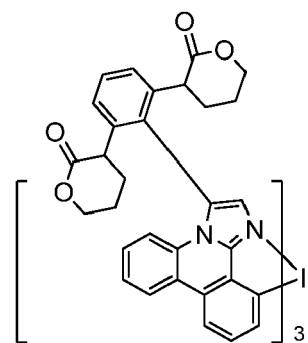
Compound 23
