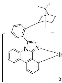
Compound 15
