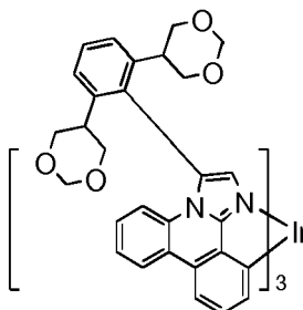
Compound 35
