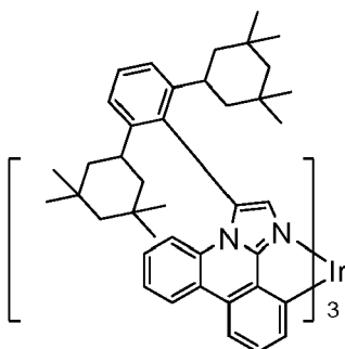
Compound 7
