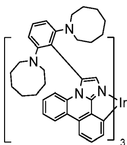
Compound 30
