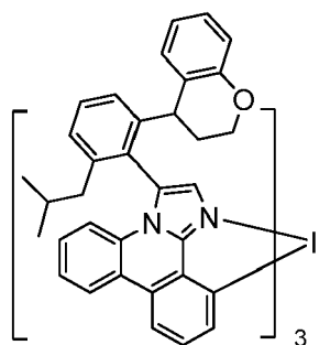
Compound 20
