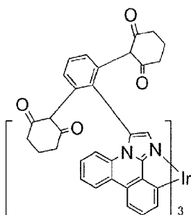
Compound 21
