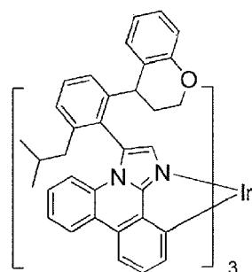
Compound 20
