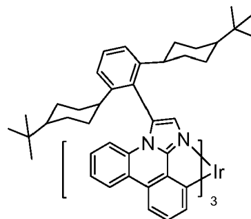
Compound 5
