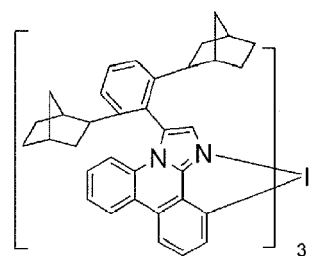
Compound 14
