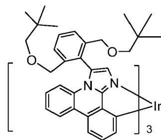
Compound 17
