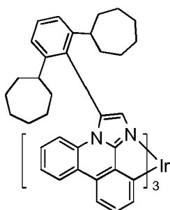
Compound 3
