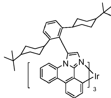
Compound 5
