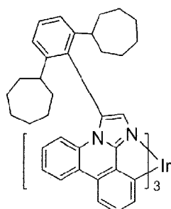
Compound 3
