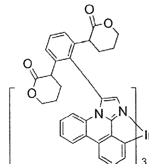
Compound 23
