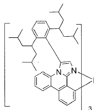
Compound 11
