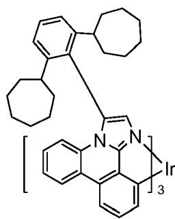
Compound 3
