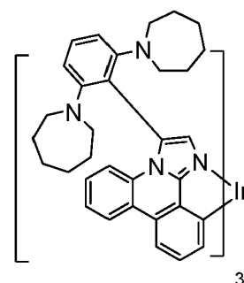
Compound 29
