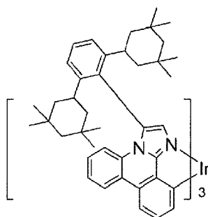
Compound 7
