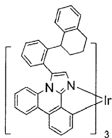
Compound 12
