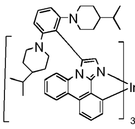
Compound 31
