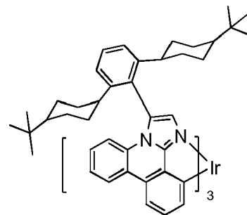
Compound 5
