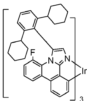
Compound 9
