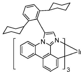
Compound 2
