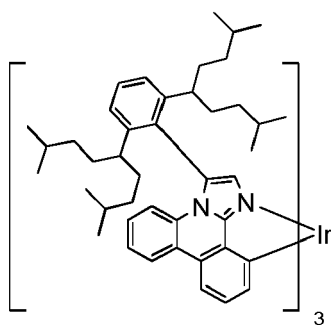
Compound 13
