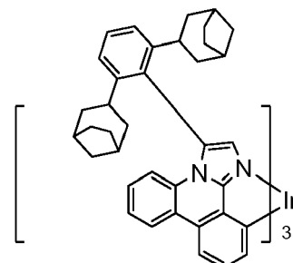
Compound 8
