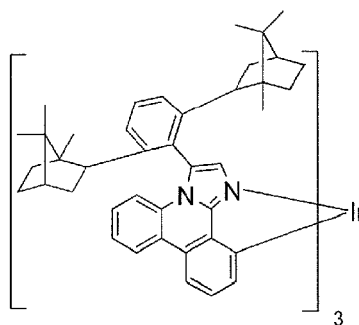
Compound 10
