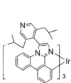
Compound 6
