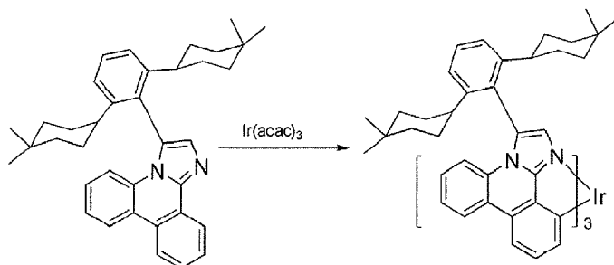
Compound 4
