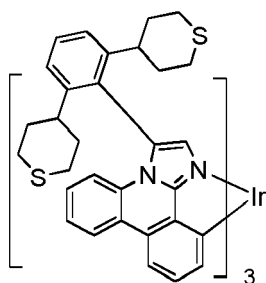
Compound 18
