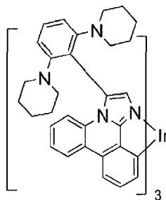
Compound 28
