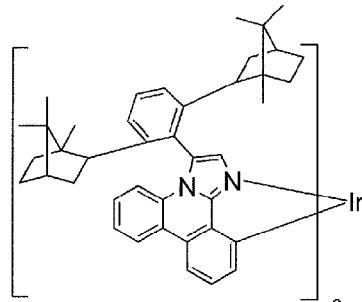
Compound 10
