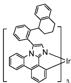
Compound 12
