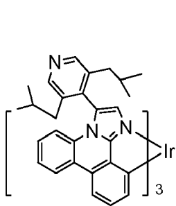
Compound 6
