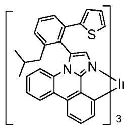
Compound 25
