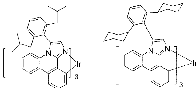
Compound 2
