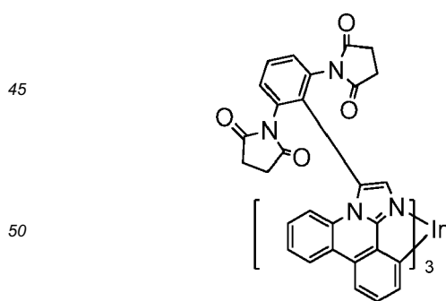
Compound 34
