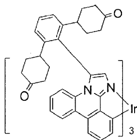
Compound 22
