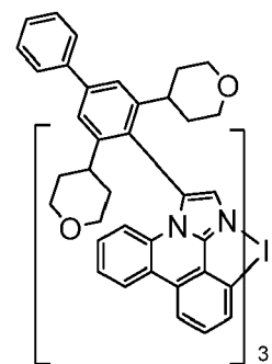
Compound 33
