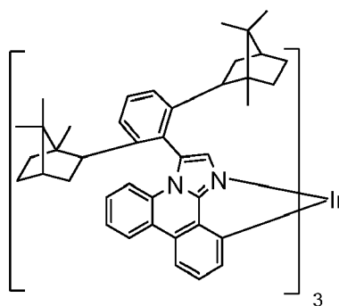
Compound 10
