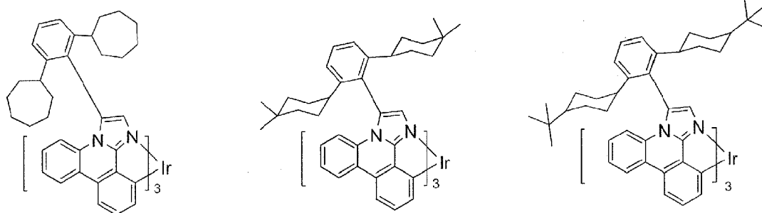
Compound 4
