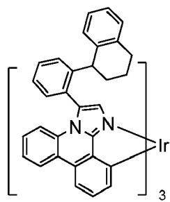
Compound 12
