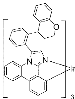
Compound 19
