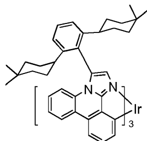
Compound 4
