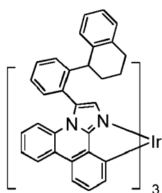
Compound 12
