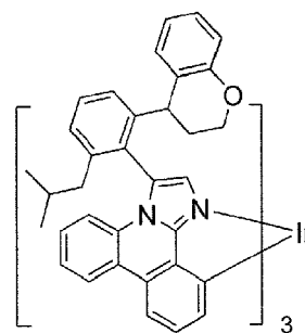
Compound 20
