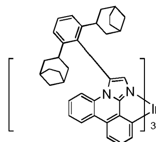
Compound 8
