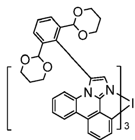
Compound 36
