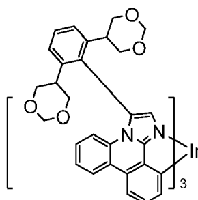
Compound 35
