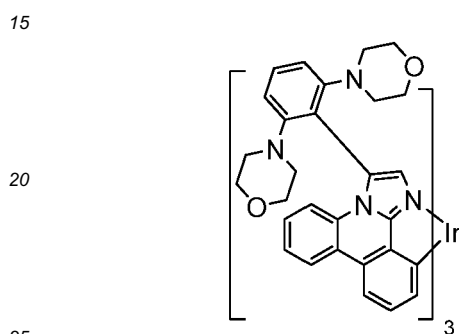
Compound 27
