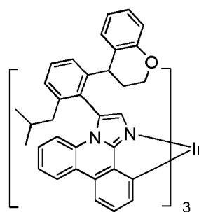
Compound 20
