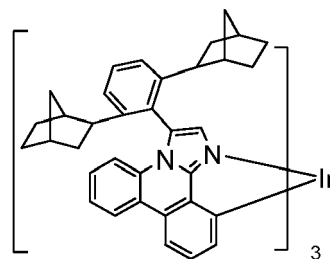
Compound 14
