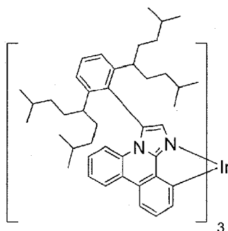
Compound 13
