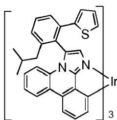
Compound 25
