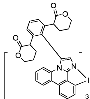
Compound 23
