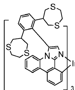
Compound 32
