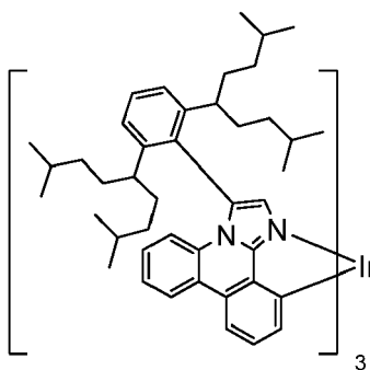
Compound 13
