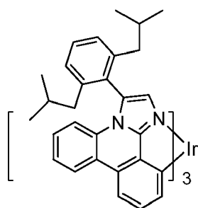
Compound 1
