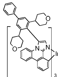
Compound 33
