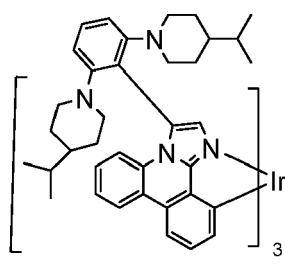
Compound 31
