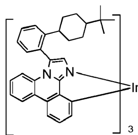
Compound 16
