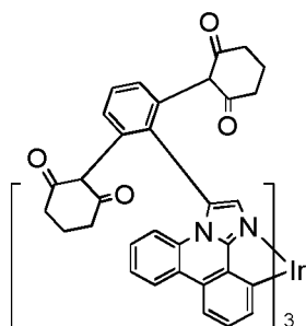
Compound 21
