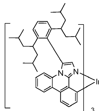
Compound 11
