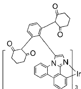
Compound 21
