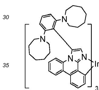
Compound 30
