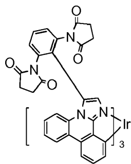
Compound 34
