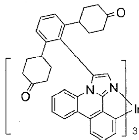
Compound 22
