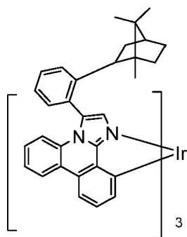
Compound 15
