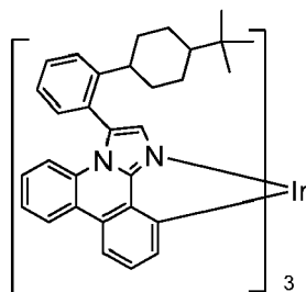
Compound 16
