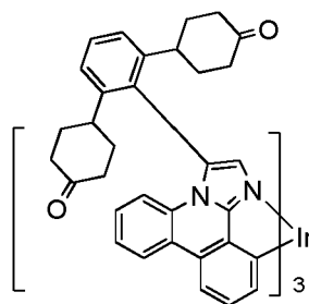
Compound 22
