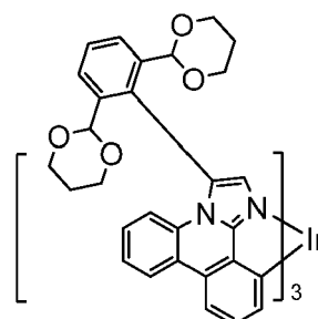
Compound 36
