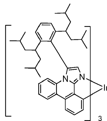
Compound 11
