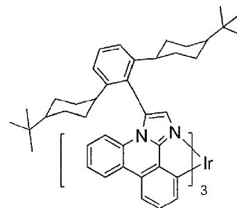
Compound 5
