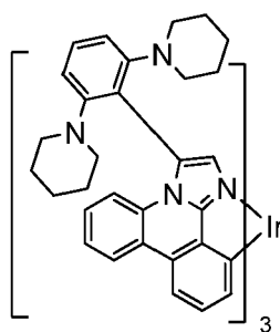
Compound 28
