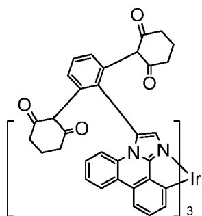
Compound 21
