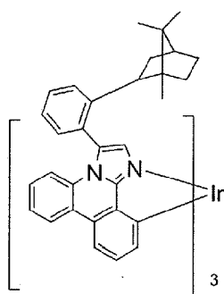
Compound 15
