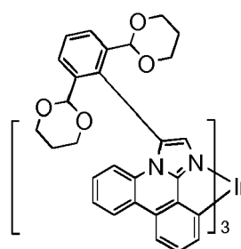
Compound 36
