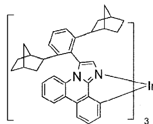
Compound 14
