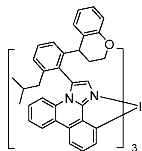
Compound 20
