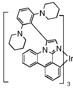
Compound 28
