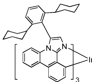
Compound 2
