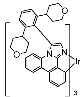
Compound 26
