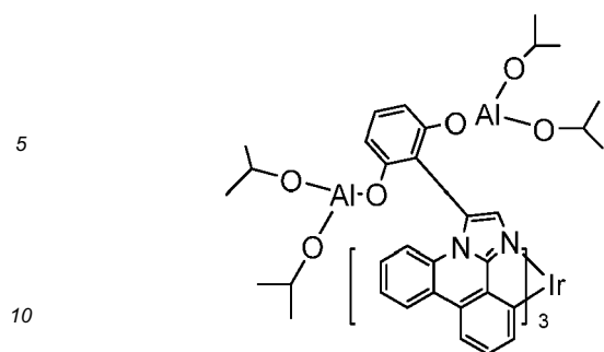
Compound 24
