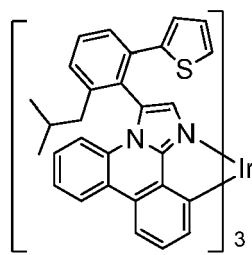
Compound 25
