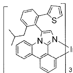
Compound 25
