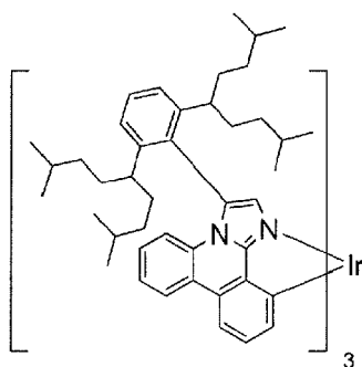
Compound 13
