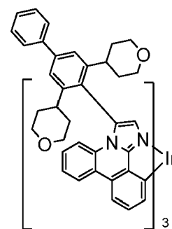
Compound 33
