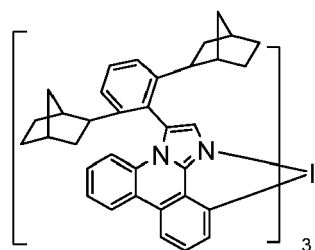
Compound 14
