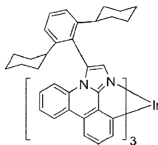
Compound 2
