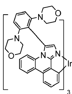
Compound 27
