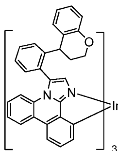
Compound 19
