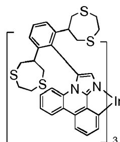
Compound 32
