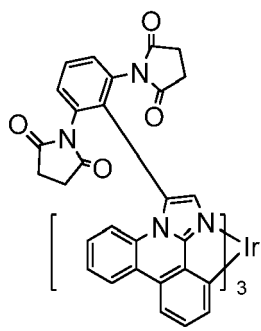
Compound 34
