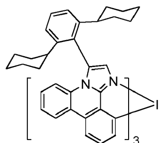
Compound 2
