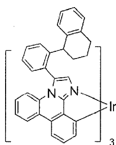
Compound 12
