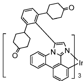
Compound 22
