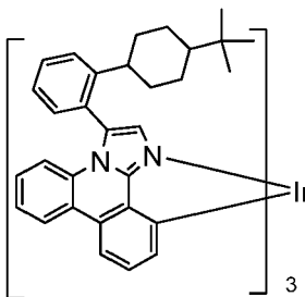
Compound 16
