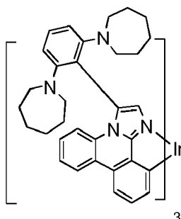
Compound 29
