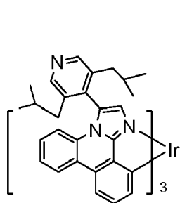
Compound 6
