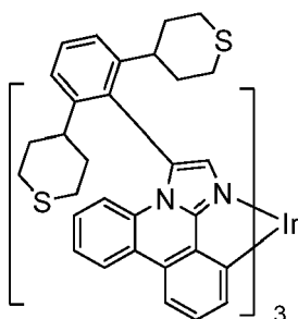
Compound 18
