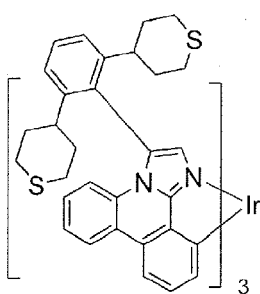
Compound 18
