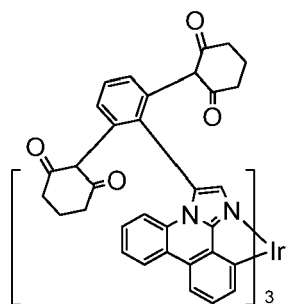
Compound 21
