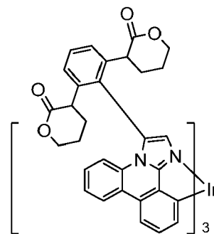
Compound 23
