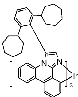
Compound 3
