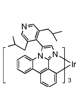
Compound 6
