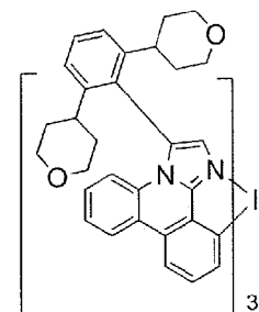
Compound 26
