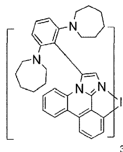
Compound 29
