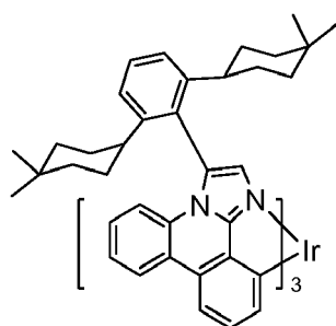
Compound 4
