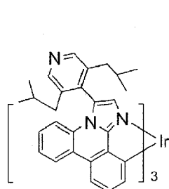
Compound 6
