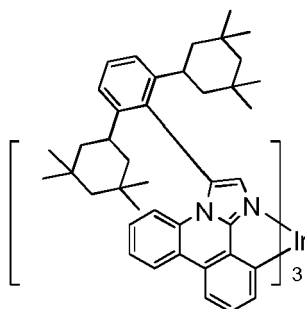
Compound 7
