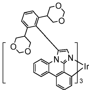
Compound 35
