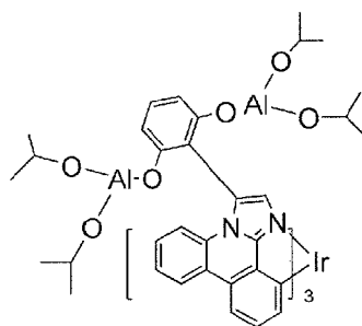
Compound 24
