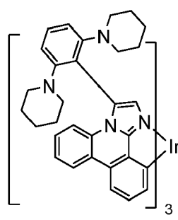
Compound 28
