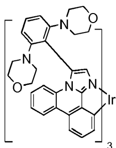
Compound 27
