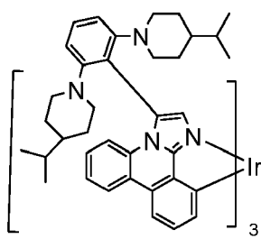
Compound 31
