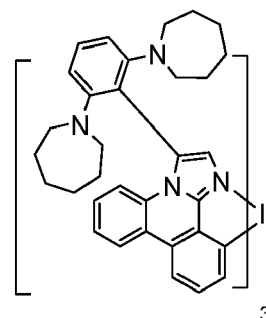
Compound 29
