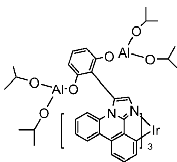
Compound 24
