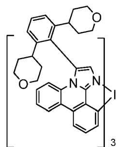
Compound 26
