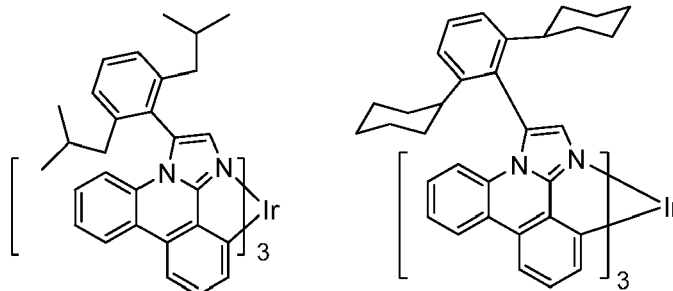
Compound 1
