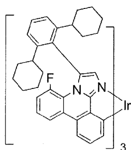
Compound 9
