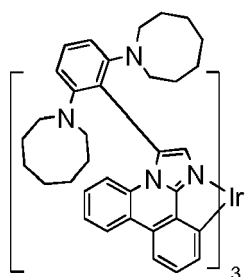
Compound 30
