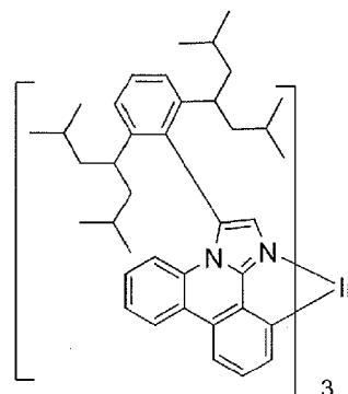
Compound 11
