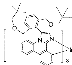
Compound 17
