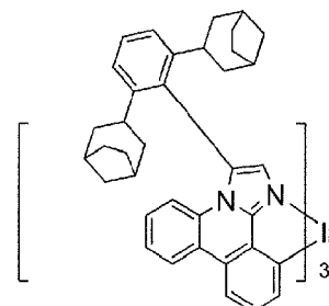
Compound 8
