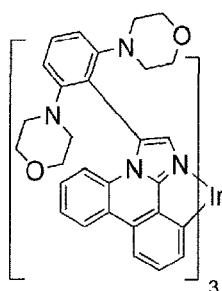
Compound 27
