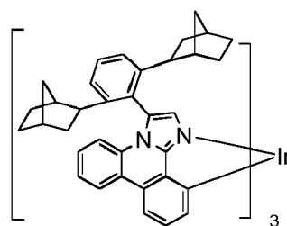
Compound 14
