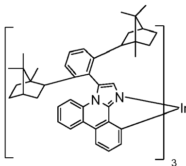
Compound 10
