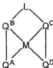
Formula (VIII)
