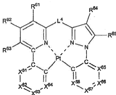
Formula (IV)
