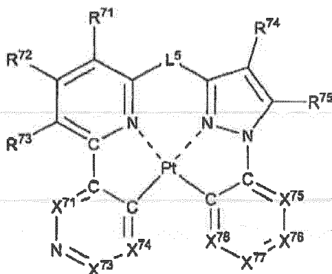
Formula (V)
