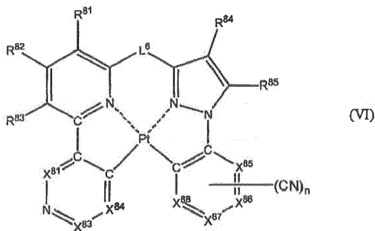
Formula (VI)
