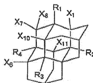
Triamantane structure
