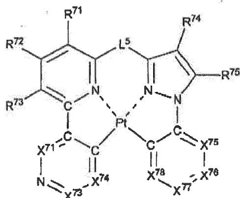
Formula (V)
