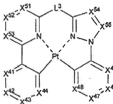
Formula (III)
