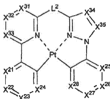
Formula (II)
