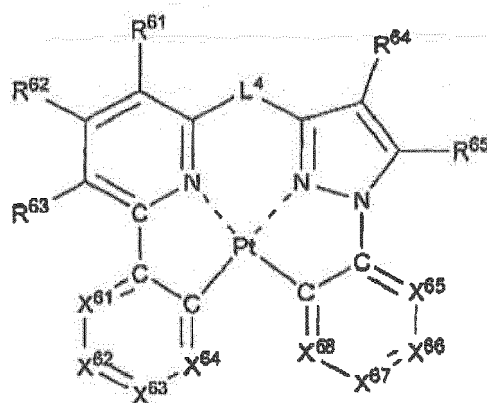
Formula (IV)
