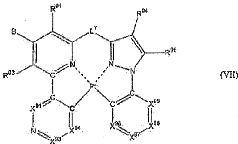
Formula (VII)
