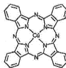
Copper phthalocyanine
