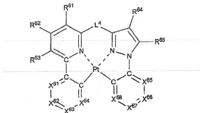
Formula (IV)
