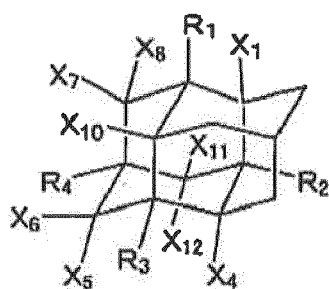
Diamantane structure
