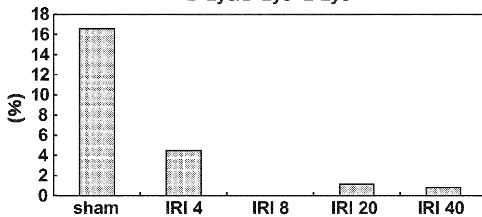
FIG. 4-L D-Lys/D-Lys+L-Lys
