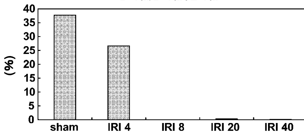
FIG. 4-I D-Val/D-Val+L-Val
