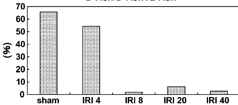
FIG. 4-B D-Asn/D-Asn+L-Asn
