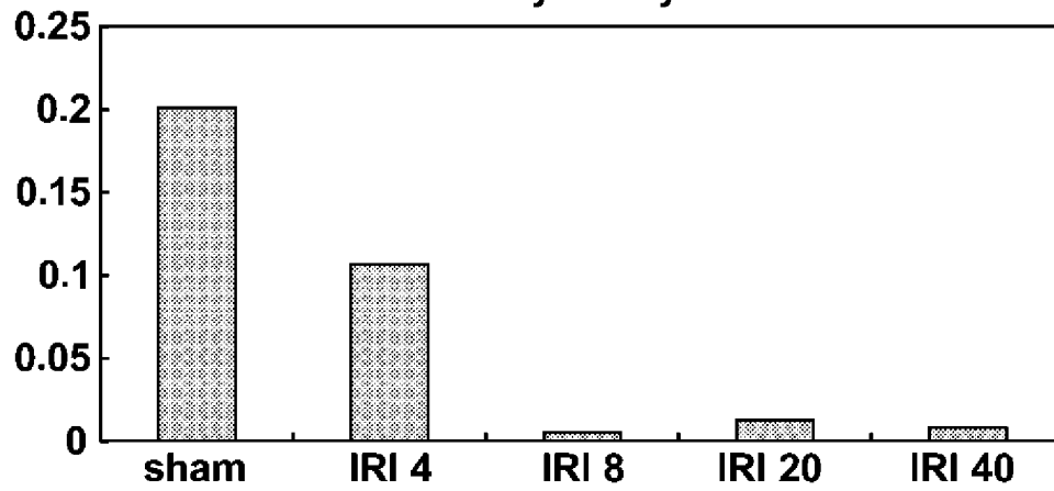
FIG. 3-L D-Lys/L-Lys
