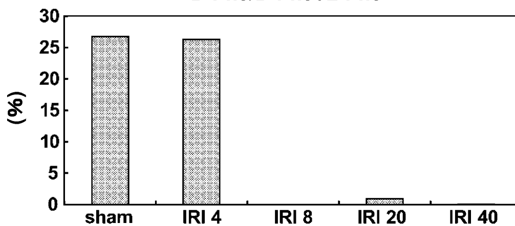
FIG. 4-K D-Phe/D-Phe+L-Phe
