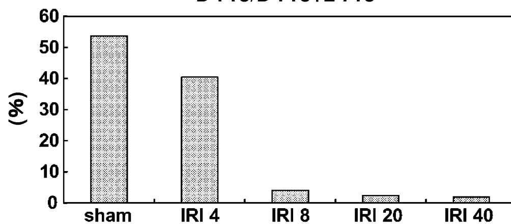
FIG. 4-H D-Pro/D-Pro+L-Pro
