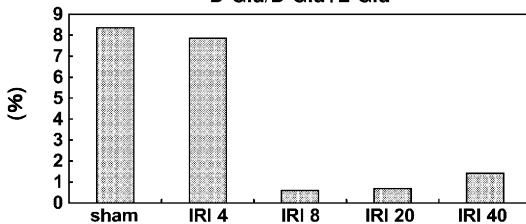
FIG. 4-F D-Glu/D-Glu+L-Glu
