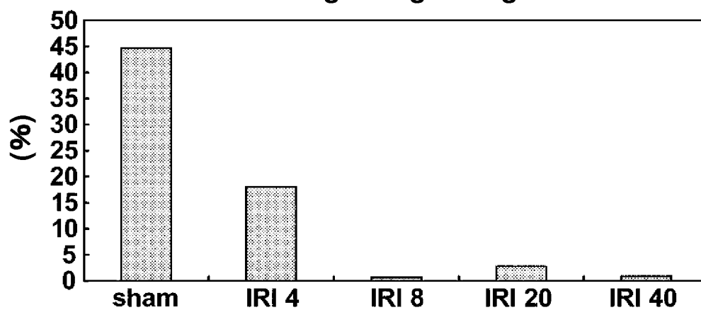
FIG. 4-D D-Arg/D-Arg+L-Arg
