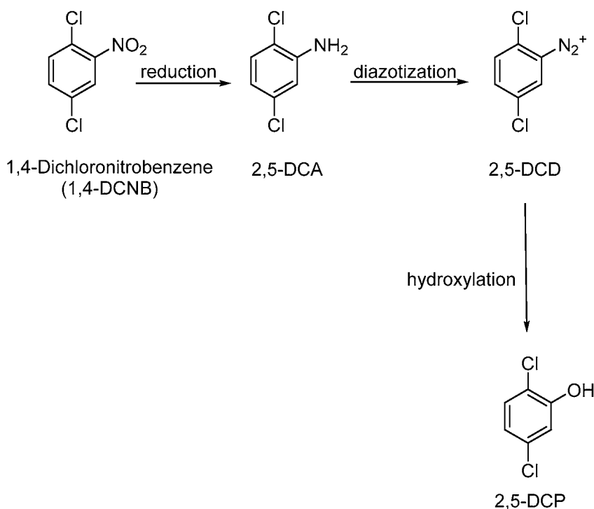
Scheme 5
