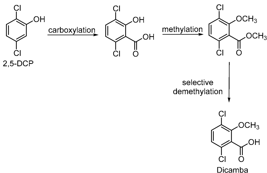
Scheme 6
