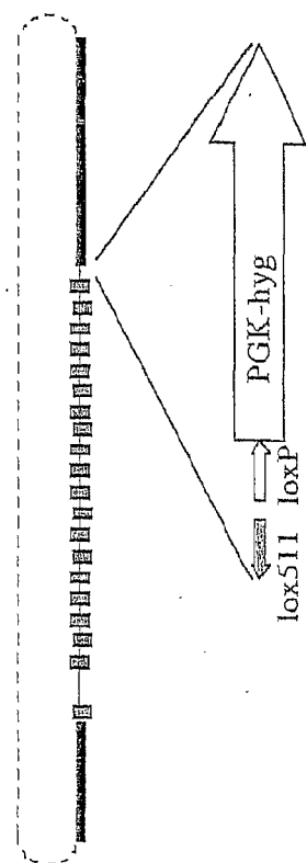
Figure 4C LTVEC2:
