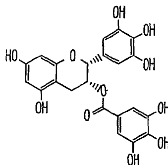
EGCG: (-)-EPIGALLOCATECHIN-3-O-GALLATE
