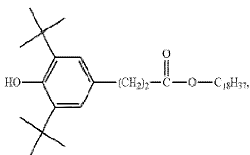
Ciba® Irganox® 1076;
