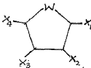
Structure II
