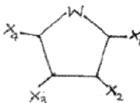
Structure II
