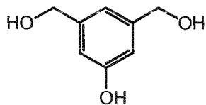
3,5-Di(hydroxymethyl)phenol
