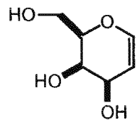
D-Galactal
