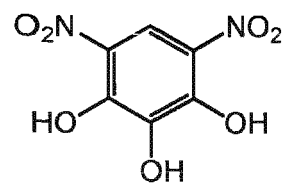
4,6-Nitropyrogallol
