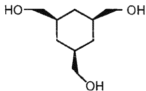
cis-1,3,5-Tri(hydroxymethyl)cyclohexane
