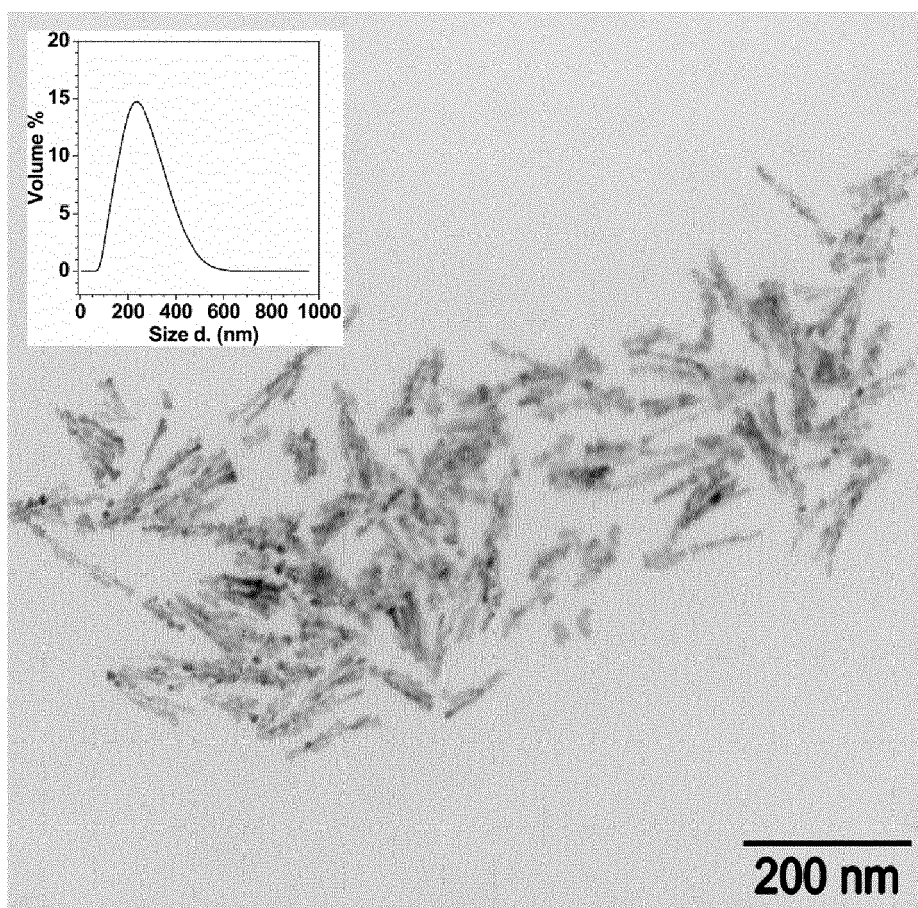
Figure 1: TEM image of ZnO nanoparticles prepared in oil medium; nano dispersion made in example 2. Particle size distribution of ZnO nanoparticles in the range 100-400 nm within oil medium (In set).
