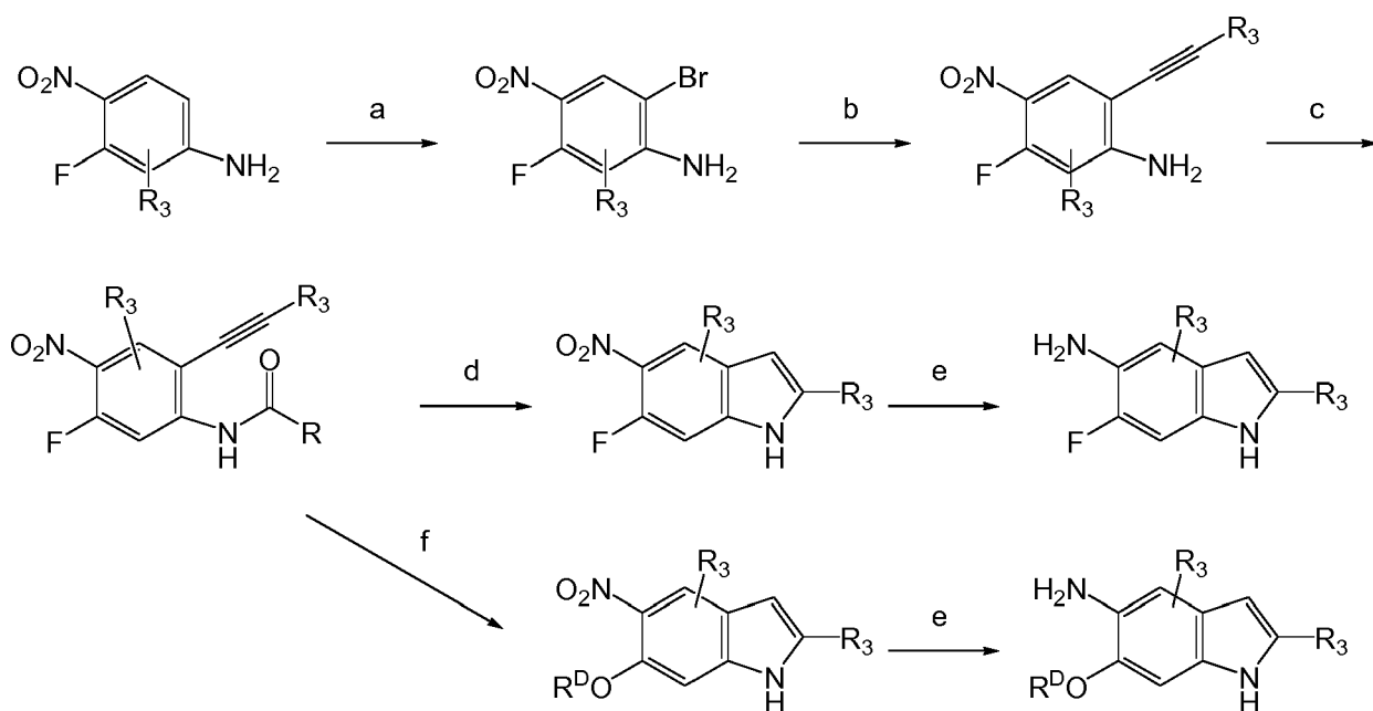
Scheme 18
