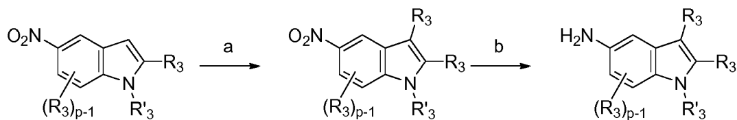
Scheme 28
