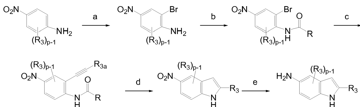
Scheme 17
