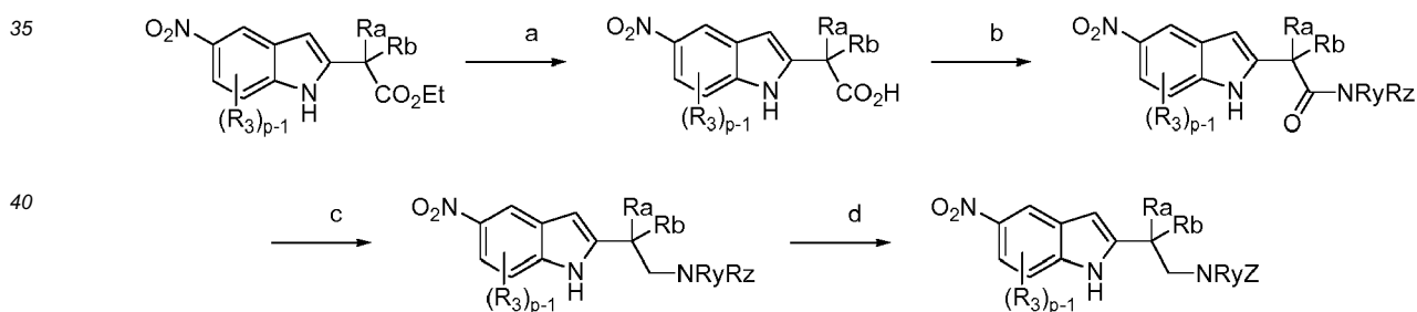
Scheme 26
