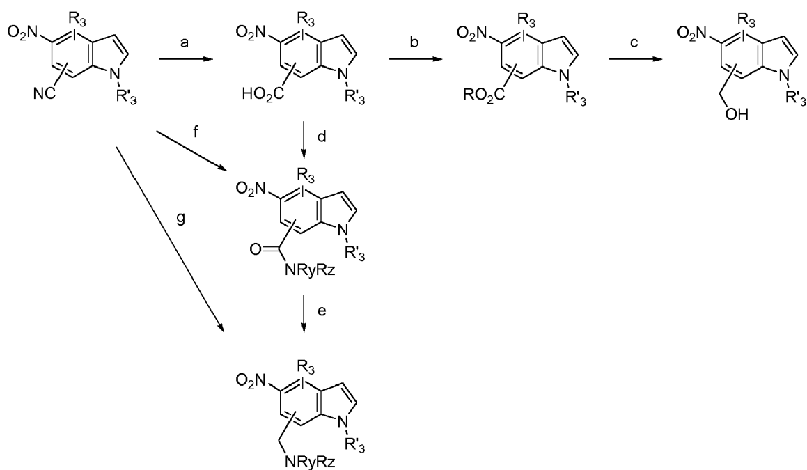
Scheme 30
