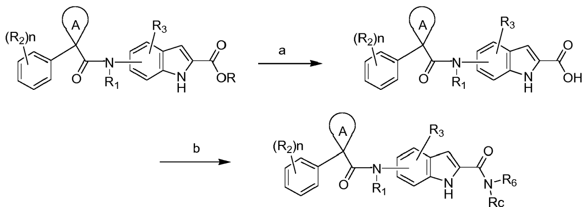
Scheme 32
