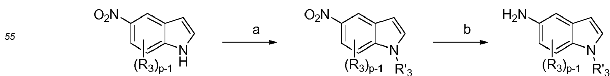
Scheme 27
