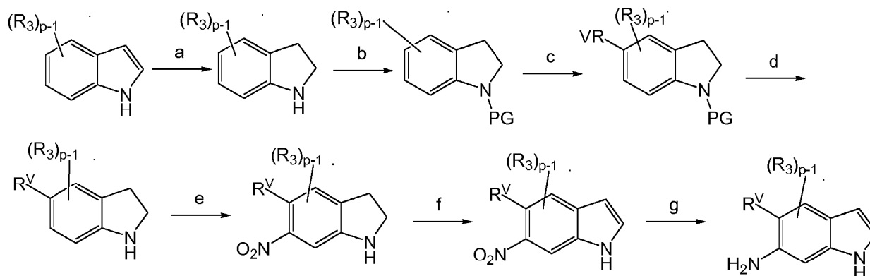
Scheme 13
