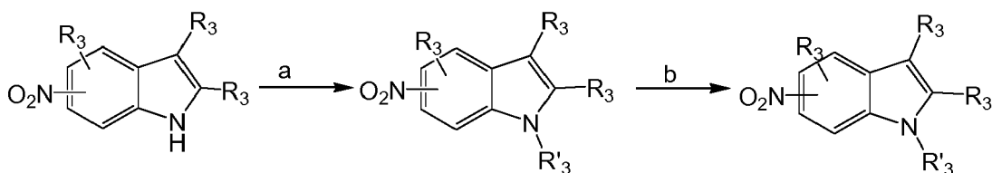
Scheme 16
