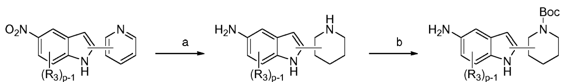
Scheme 29
