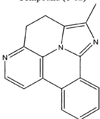
Compound (1-62)
