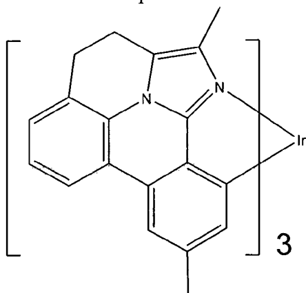
Compound 89
