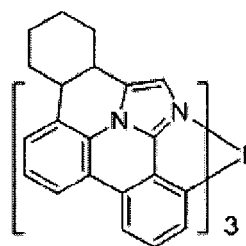
Compound 8
