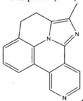
Compound (1-66)
