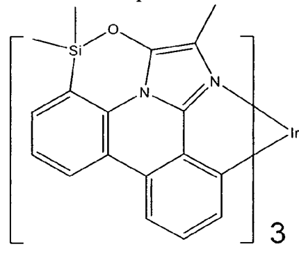
Compound 64
