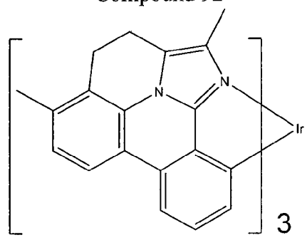
Compound 92
