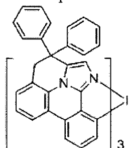
Compound 6
