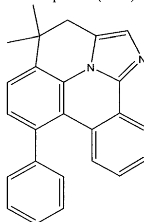
Compound (1-36)
