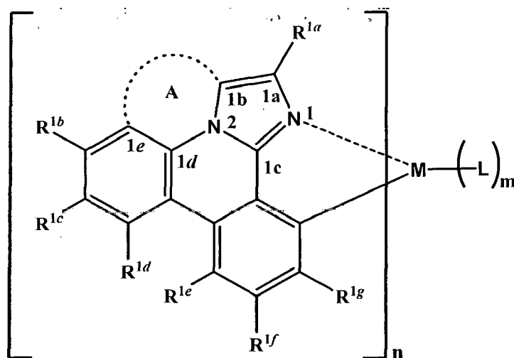
, Formula 1;
