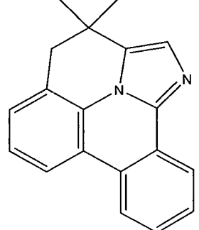
Compound (1-36)
