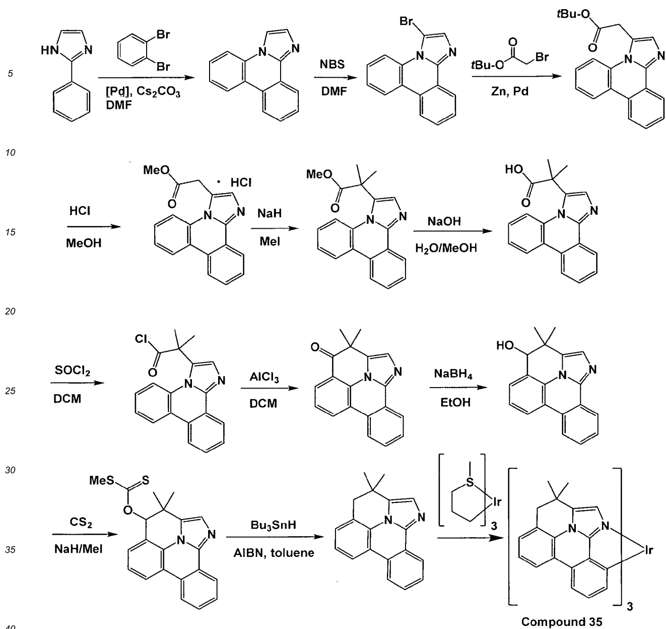
Scheme 5
