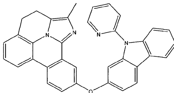
Compound (3-4)
