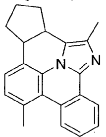
Compound (1-154)
