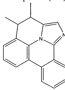
Compound (1-4)
