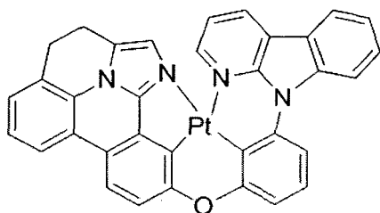
Compound 103
