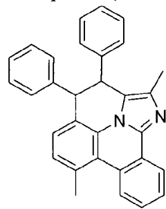
Compound (1-151)
