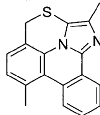
Compound (1-163)
