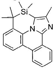
Compound (1-88)
