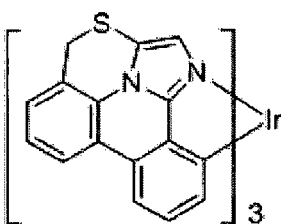
Compound 19
