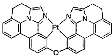
Compound 99
