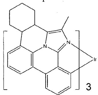
Compound 58
