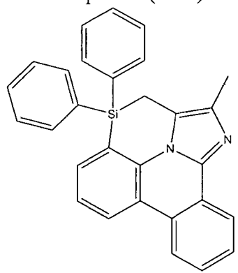
Compound (1-59)
