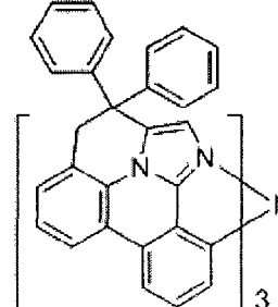
Compound 6
