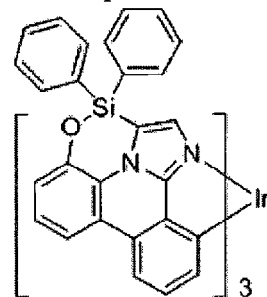
Compound 12
