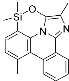
Compound (1-159)
