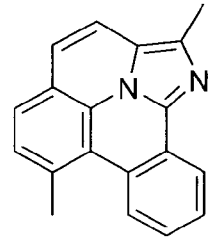
Compound (1-166)
