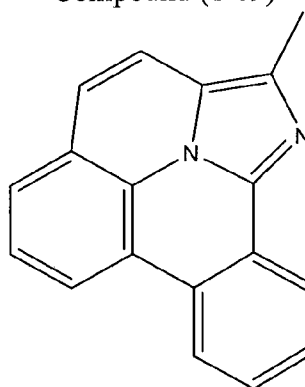
Compound (1-69)
