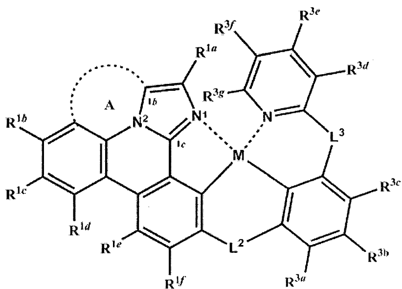
, Formula 3;
