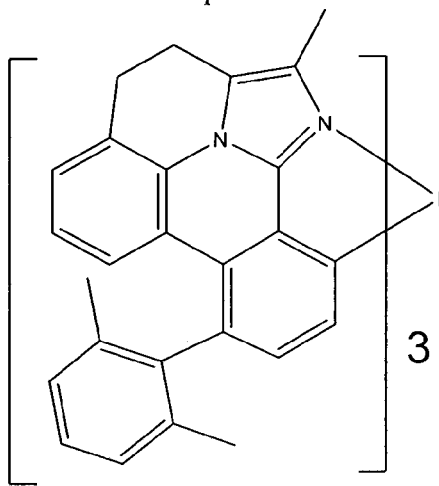
Compound 94
