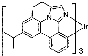
Compound 11
