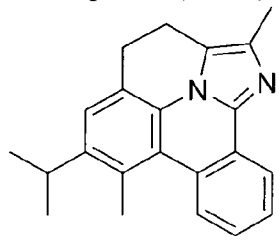
Compound (1-156)
