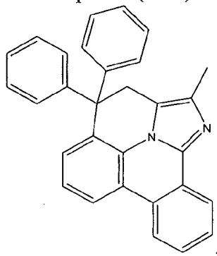
Compound (1-43)
