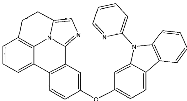
Compound (3-1)
