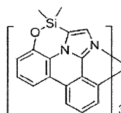
Compound 14
