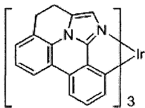
Compound 1
