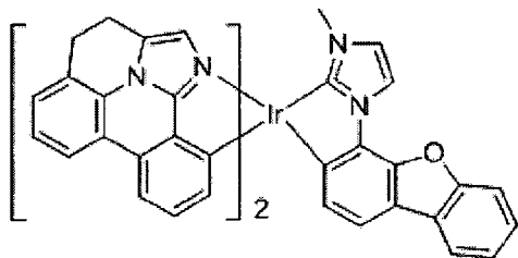
Compound 23
