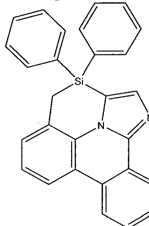
Compound (1-26)
