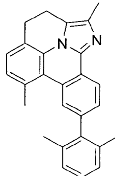
Compound (1-165)
