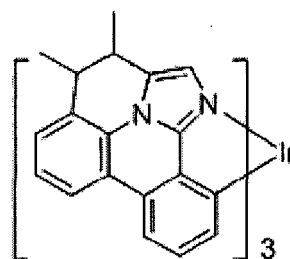
Compound 4
