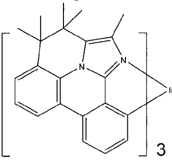
Compound 53
