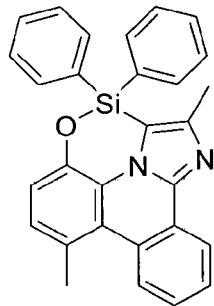
Compound (1-158)
