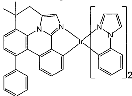
Compound 52
