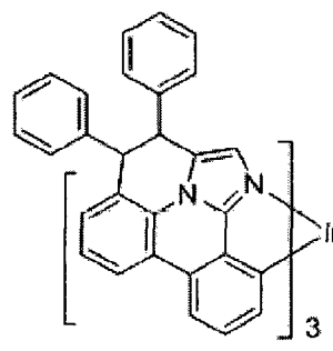
Compound 6
