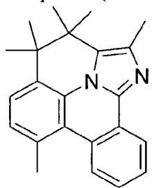
Compound (1-148)
