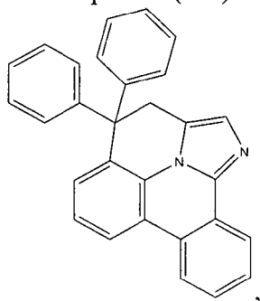
Compound (1-5)
