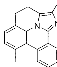
Compound (1-155)
