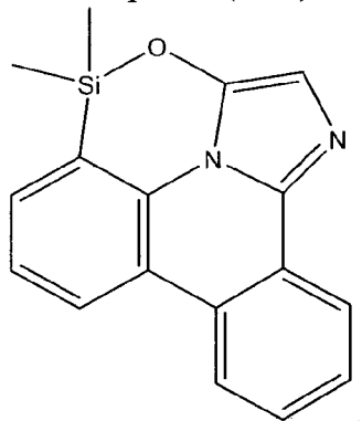
Compound (1-15)
