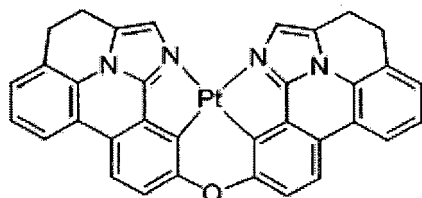
Compound 99
