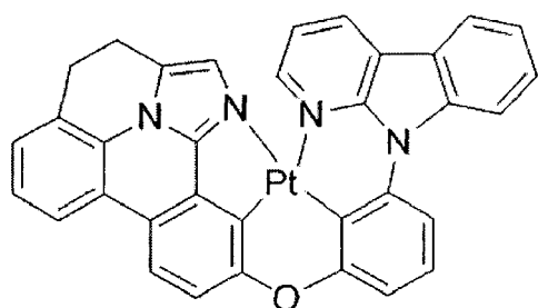
Compound 103
