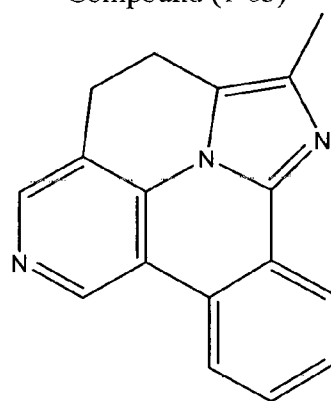
Compound (1-63)
