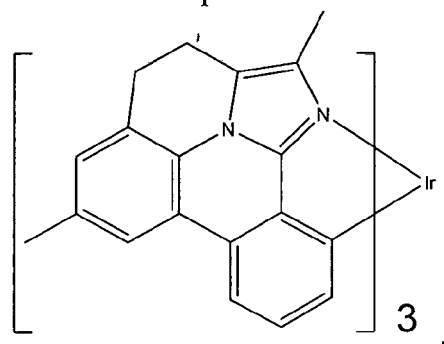
Compound 93
