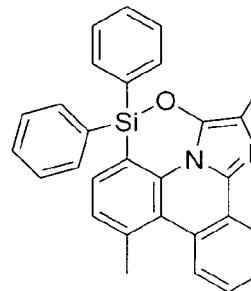
Compound (1-157)
