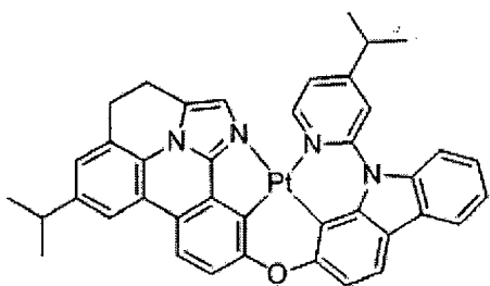
Compound 105
