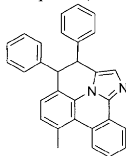
Compound (1-105)
