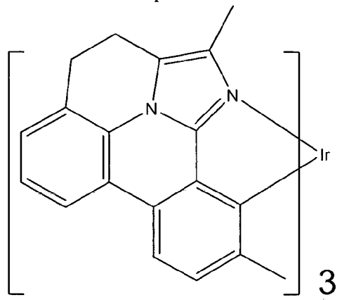
Compound 90
