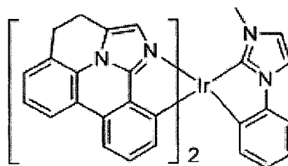
Compound 20
