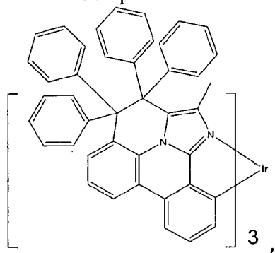
Compound 57
