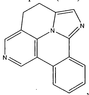
Compound (1-31)
