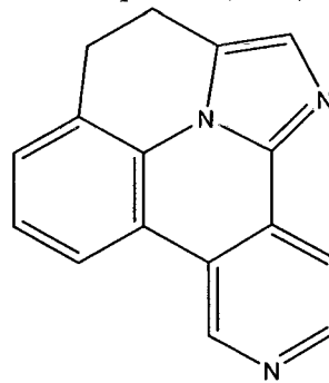
Compound (1-34)
