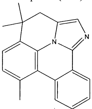
Compound (1-35)
