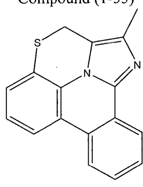
Compound (1-55)
