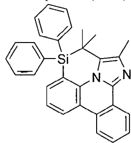
Compound (1-89)
