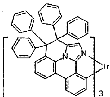
Compound 9
