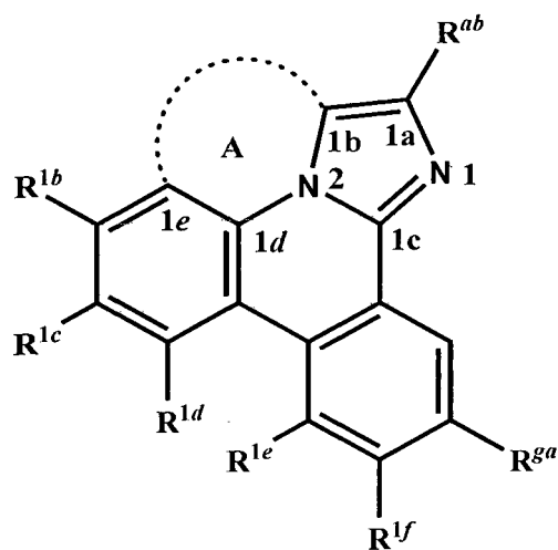
, Formula (1a).
