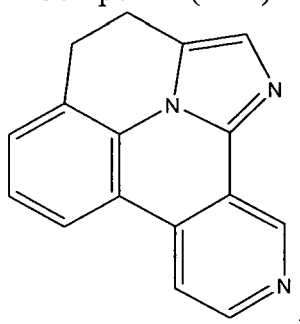
Compound (1-33)
