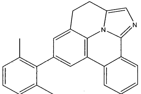
Compound (1-25)
