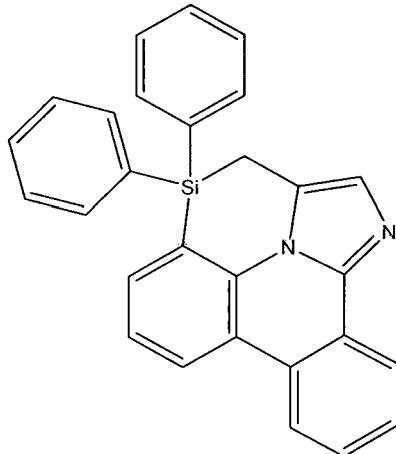
Compound (1-27)
