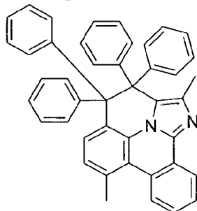
Compound (1-154)
