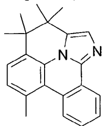
Compound (1-102)
