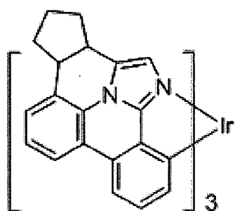
Compound 9
