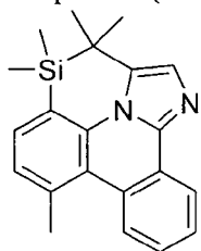
Compound (1-96)
