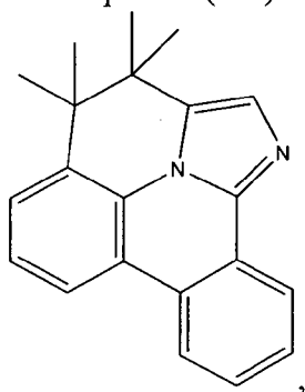
Compound (1-3)
