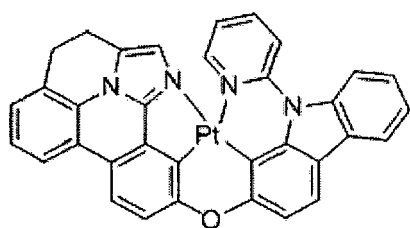
Compound 101
