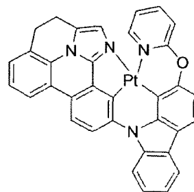
Compound 104
