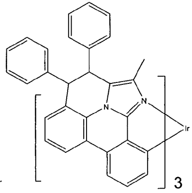
Compound 56
