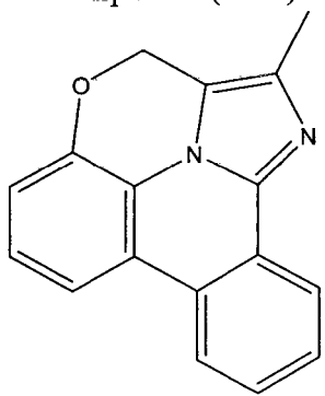
Compound (1-56)
