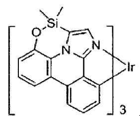
Compound 14
