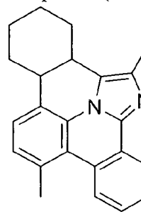
Compound (1-155)
