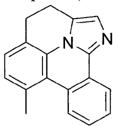
Compound (1-100)
