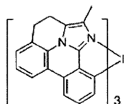
Compound 10
