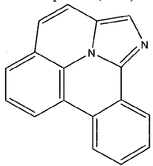
Compound (1-20)
