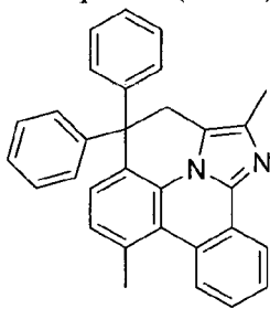
Compound (1-152)
