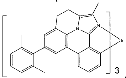
Compound 81
