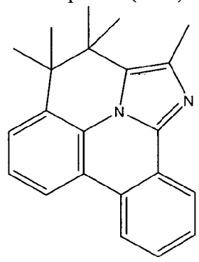
Compound (1-41)
