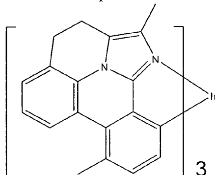
Compound 88
