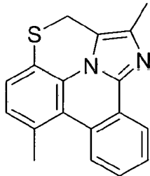
Compound (1-162)
