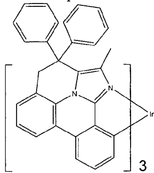
Compound 56
