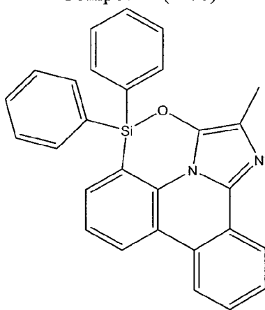
Compound (1-68)
