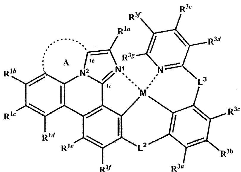
, Formula 3;
