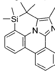
Compound (1-87)
