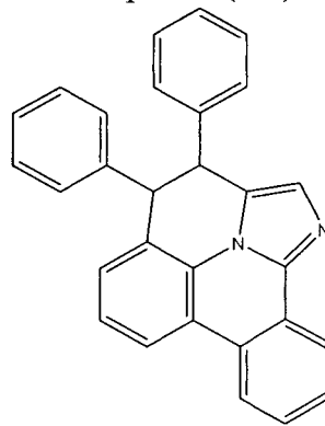
Compound (1-6)
