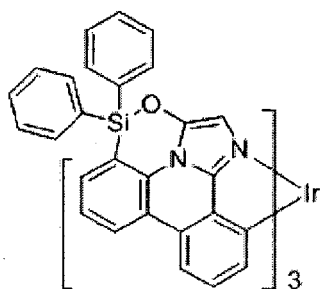
Compound 13
