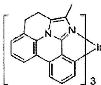
Compound 10
