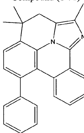
Compound (1-71)
