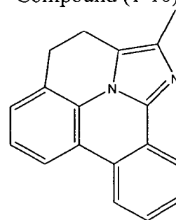
Compound (1-12)
