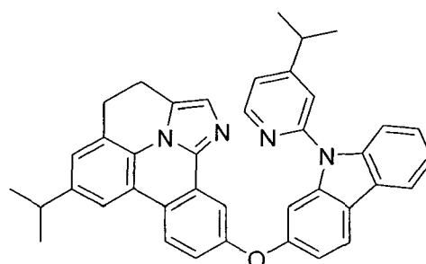
Compound (3-6)
