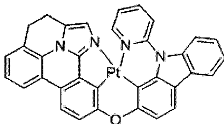
Compound 101
