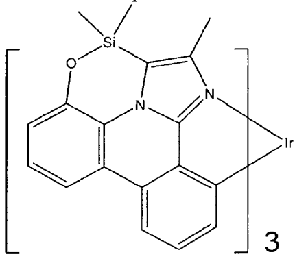
Compound 63
