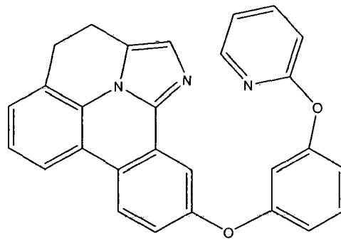
Compound (3-2)
