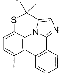
Compound (1-94)
