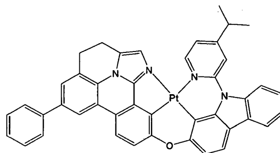
Compound 106
