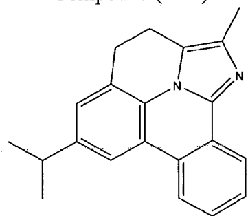
Compound (1-47)
