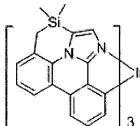
Compound 24
