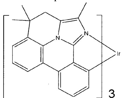
Compound 85
