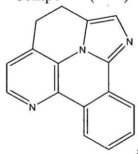
Compound (1-32)
