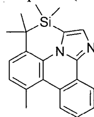
Compound (1-99)
