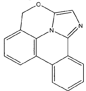
Compound (1-22)
