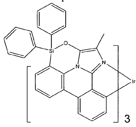
Compound 64
