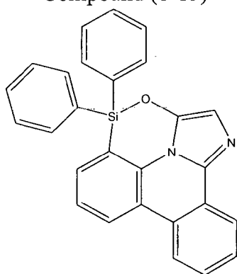
Compound (1-13)
