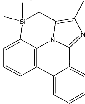
Compound (1-59)
