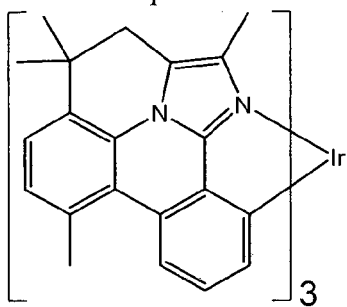
Compound 49
