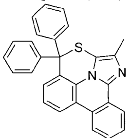
Compound (1-86)
