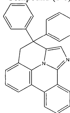
Compound (1-6)
