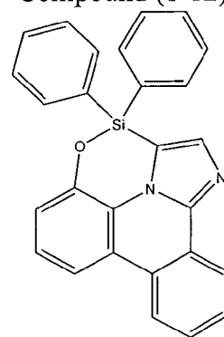
Compound (1-14)
