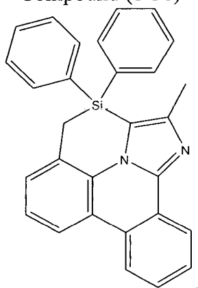
Compound (1-58)
