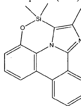
Compound (1-49)
