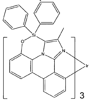
Compound 63
