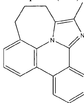
Compound (1-51)
