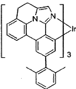
Compound 21
