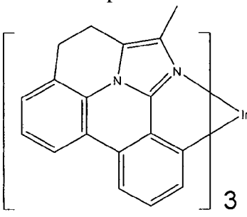
Compound 51
