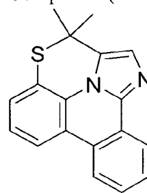
Compound (1-75)
