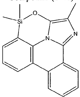
Compound (1-50)
