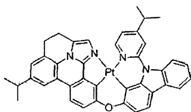
Compound 105
