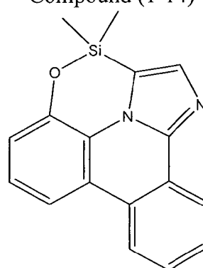
Compound (1-14)
