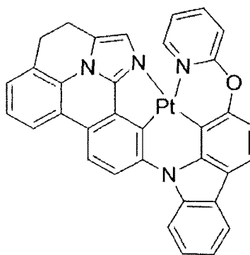
Compound 106
