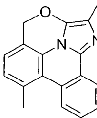
Compound (1-167)
