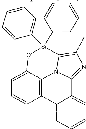
Compound (1-50)
