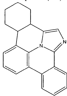
Compound (1-10)
