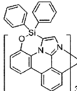
Compound 12
