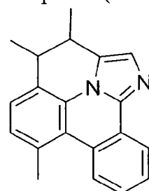
Compound (1-103)
