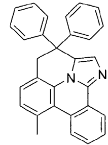
Compound (1-105)
