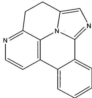
Compound (1-28)
