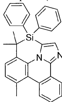
Compound (1-99)
