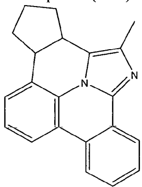
Compound (1-48)
