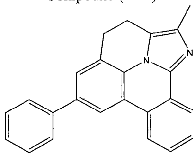
Compound (1-45)
