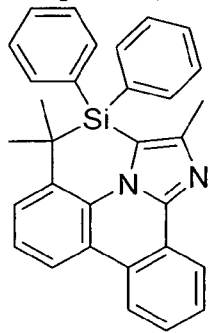
Compound (1-92)
