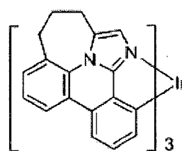
Compound 16
