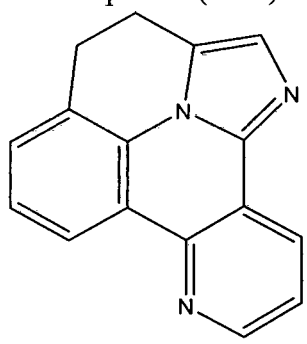
Compound (1-33)
