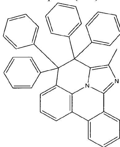
Compound (1-43)
