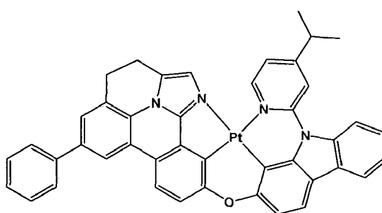
Compound 106
