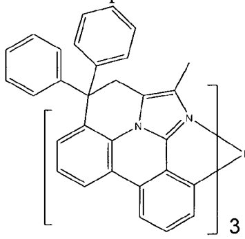
Compound 55
