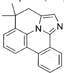
Compound (1-72)
