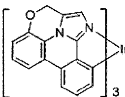
Compound 24
