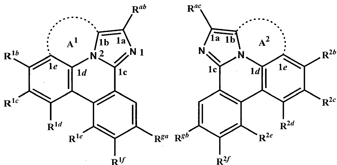
Formula (2a)
