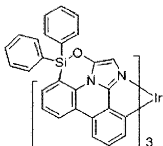
Compound 13
