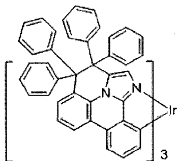
Compound 7
