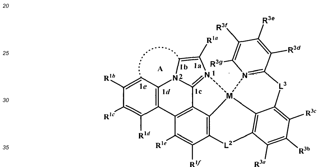
Formula 3
