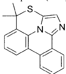
Compound (1-74)
