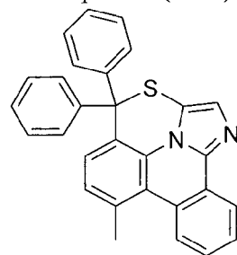
Compound (1-95)
