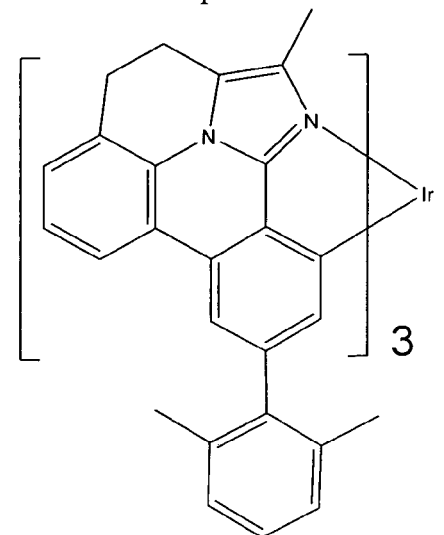
Compound 93
