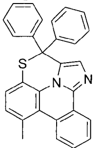
Compound (1-94)
