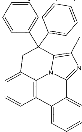
Compound (1-42)
