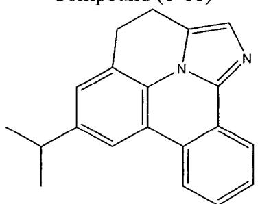
Compound (1-11)
