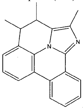
Compound (1-40)
