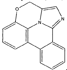
Compound (1-21)
