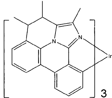
Compound 54
