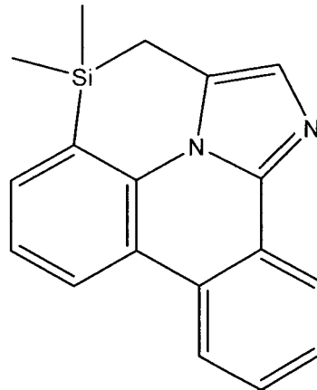
Compound (1-24)
