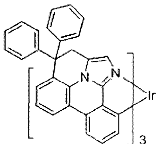
Compound 5
