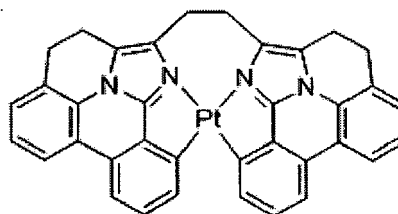
Compound 100
