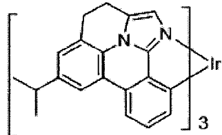
Compound 11
