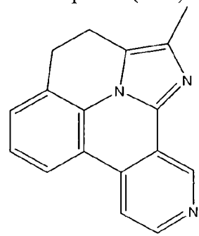
Compound (1-67)
