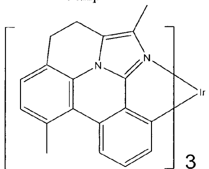
Compound 87
