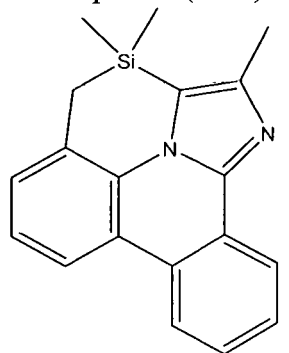
Compound (1-58)
