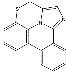
Compound (1-18)
