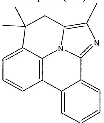
Compound (1-70)
