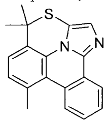
Compound (1-95)
