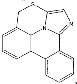
Compound (1-19)
