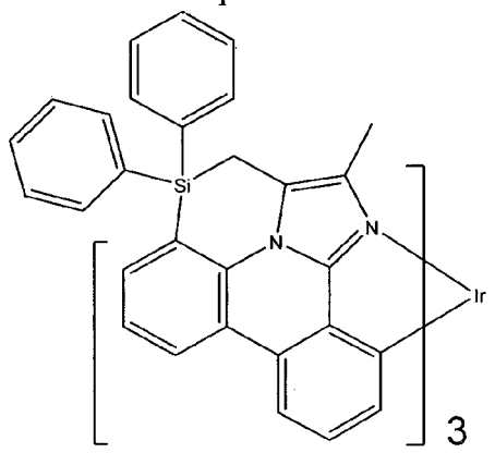
Compound 85
