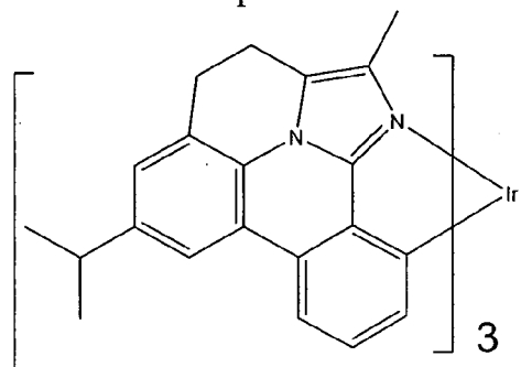
Compound 60
