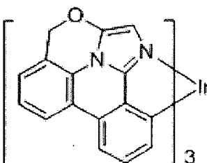
Compound 23
