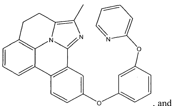
Compound (3-5)
