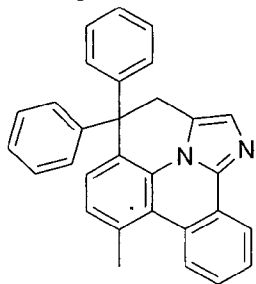
Compound (1-104)
