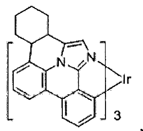
Compound 8
