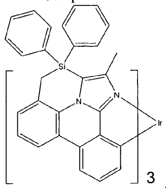
Compound 84
