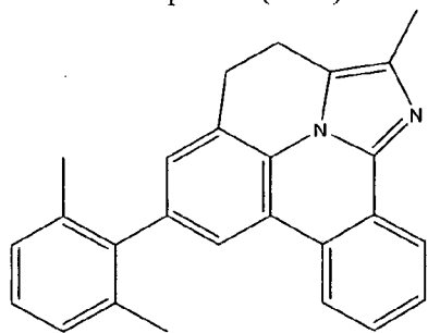
Compound (1-60)
