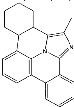
Compound (1-46)
