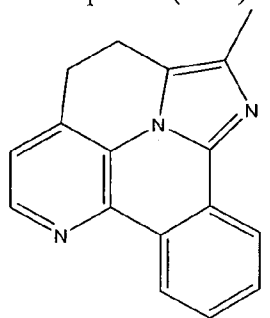
Compound (1-66)
