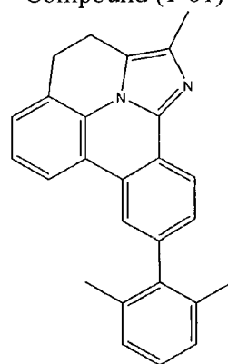
Compound (1-61)
