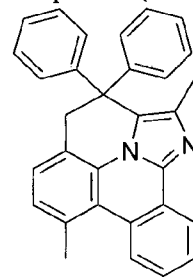
Compound (1-153)
