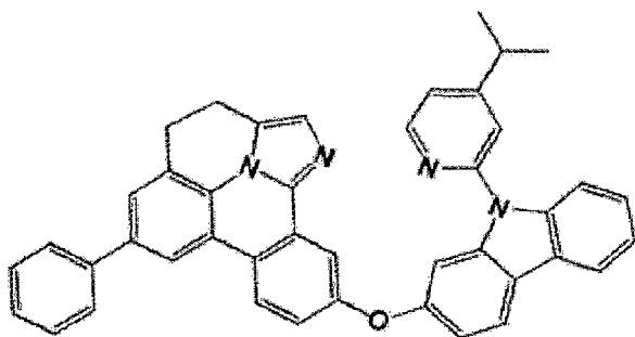
Compound (3-5)
