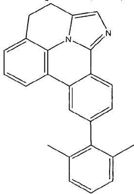
Compound (1-21)
