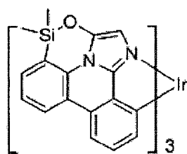
Compound 15
