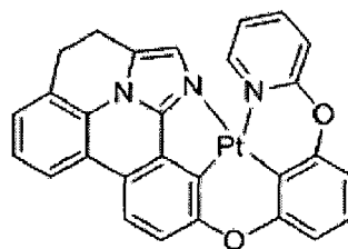
Compound 102
