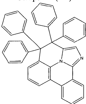
Compound (1-9)
