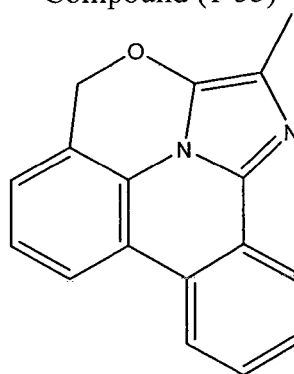
Compound (1-57)
