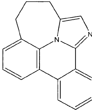
Compound (1-16)
