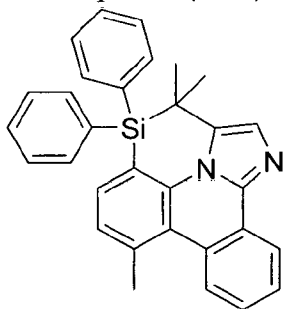
Compound (1-98)
