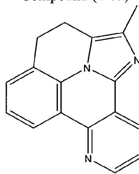
Compound (1-67)
