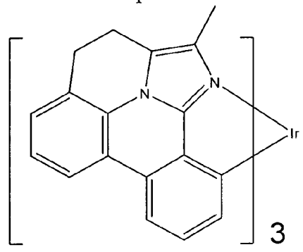
Compound 88
