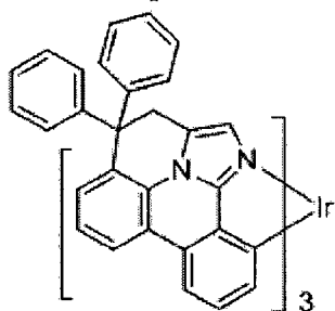
Compound 7
