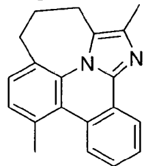
Compound (1-160)
