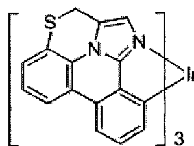
Compound 18
