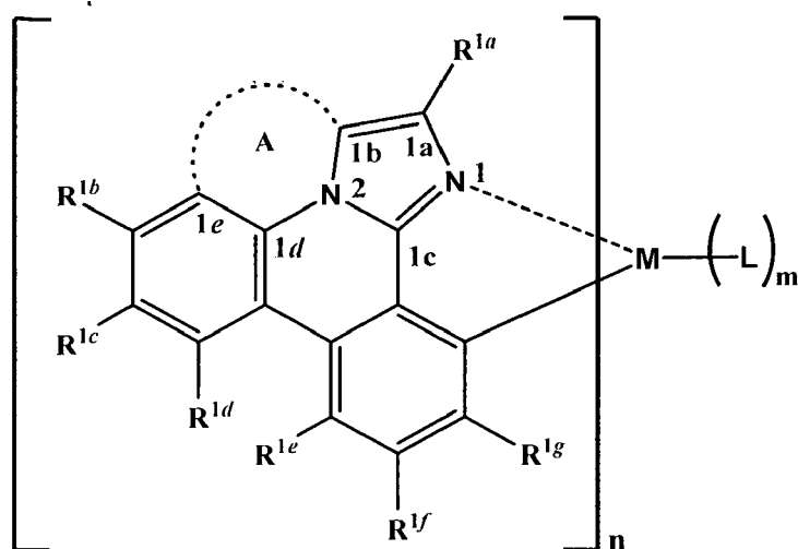
, Formula 1.
