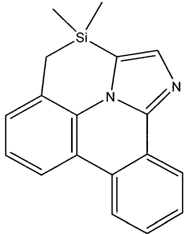
Compound (1-23)
