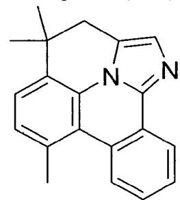
Compound (1-91)
