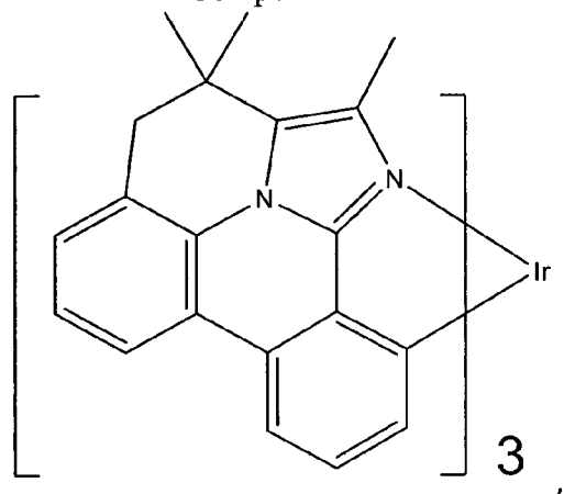
Compound 86
