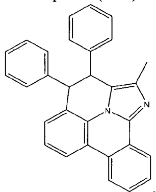
Compound (1-42)
