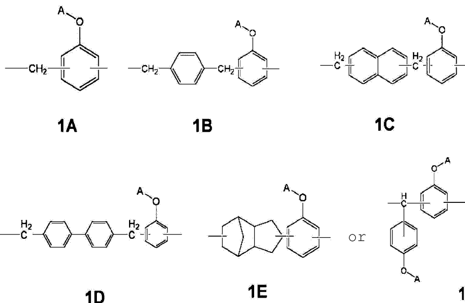
[Formula I-2]
