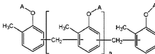
[Formula I-2]
