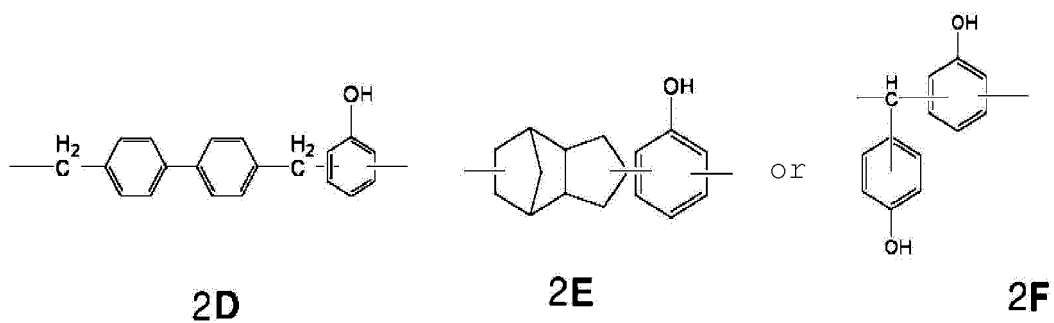
[Formula IA-2]
