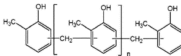
[Formula IA-2]
