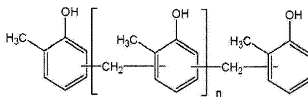
[Formula IA-3]
