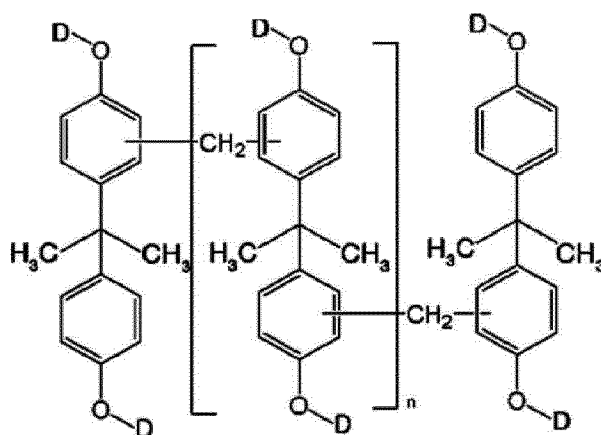
[Formula IB-4]
