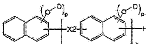
[Formula IB-4]
