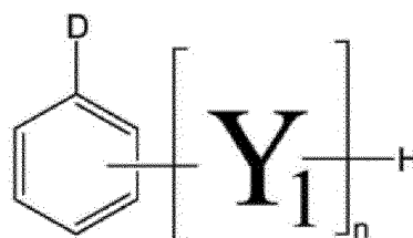
[Formula IB-1]
