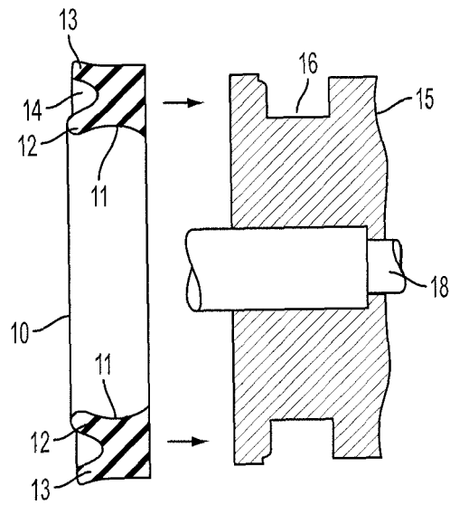
FIG. 2 PRIOR ART
