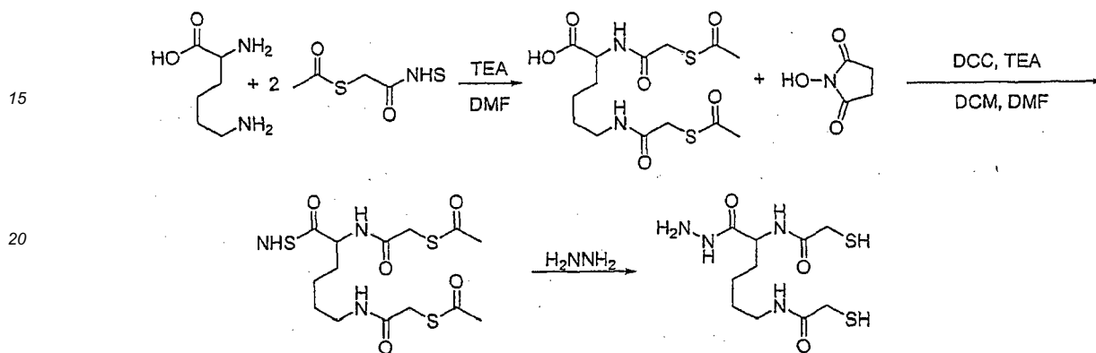
Scheme 17b
