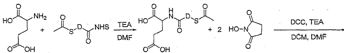
Scheme 4b
