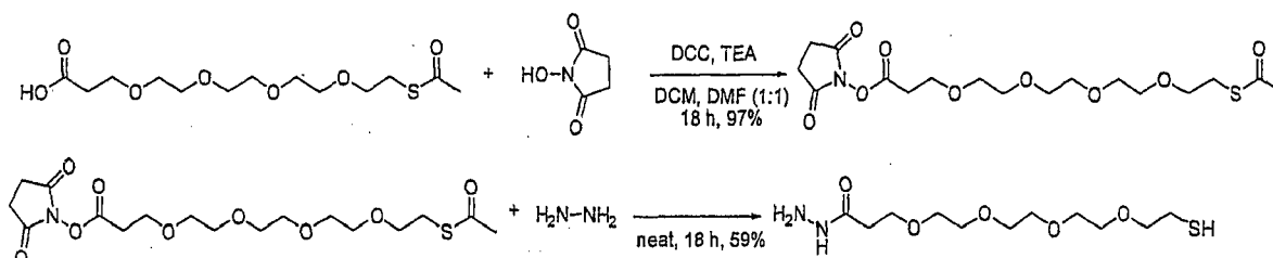
Scheme 10
