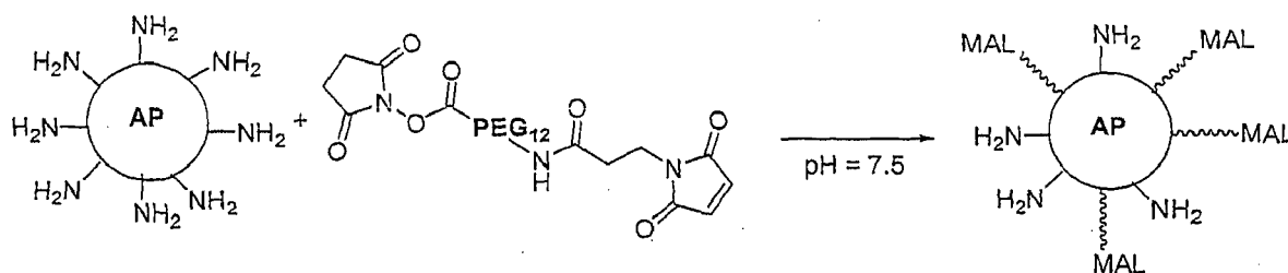
Scheme 12
