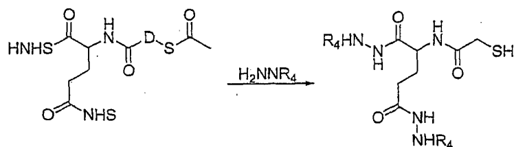
Scheme 4c
