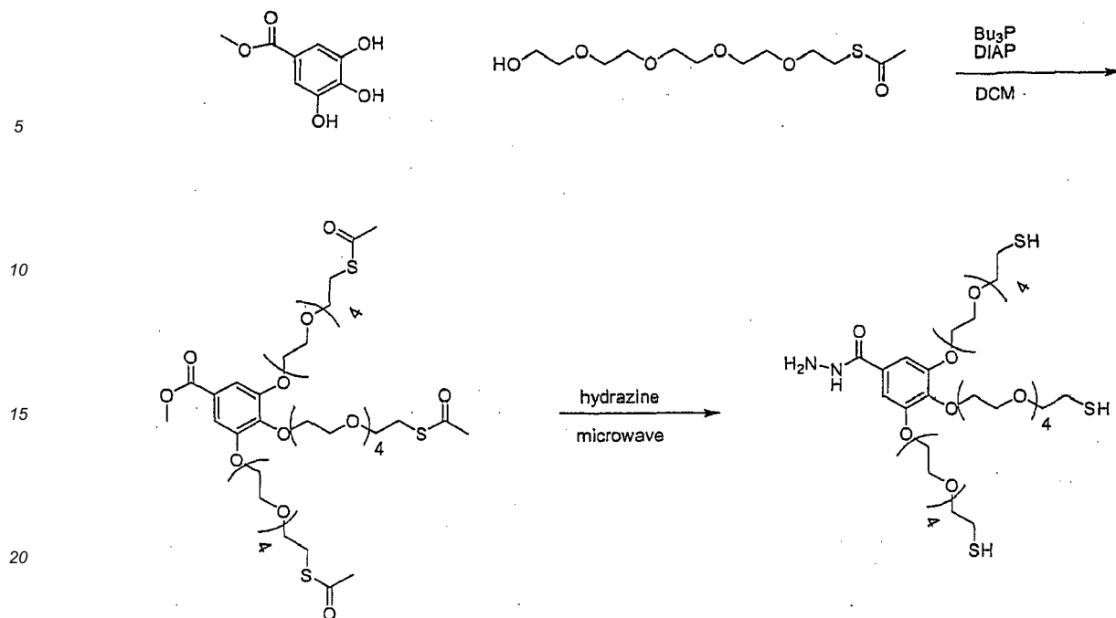
Scheme 18b
