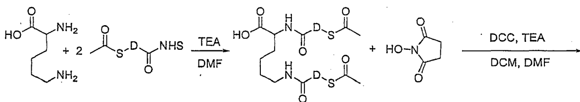
Scheme 4a
