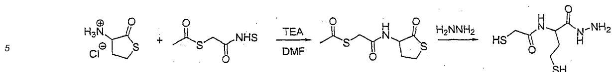
Scheme 17a
