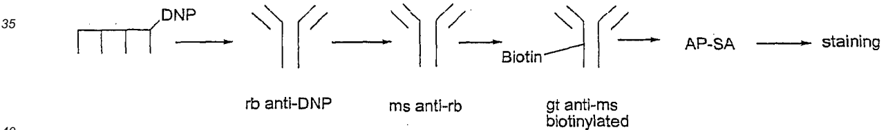
Scheme 14
