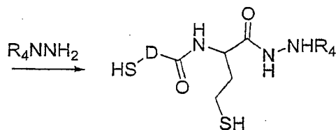
Scheme 4a
