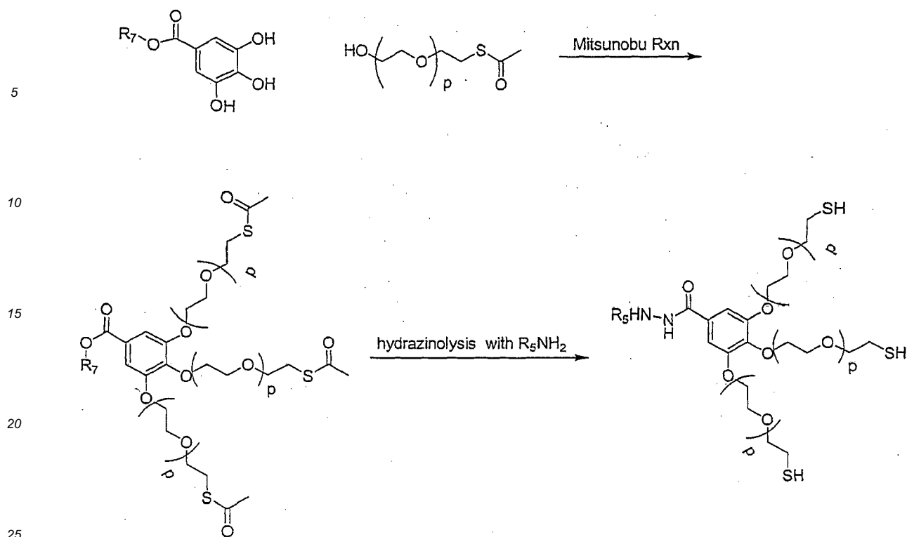
Scheme 5c
