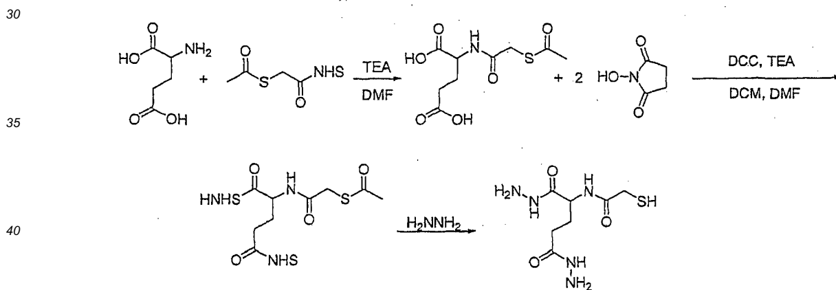
Scheme 17c
