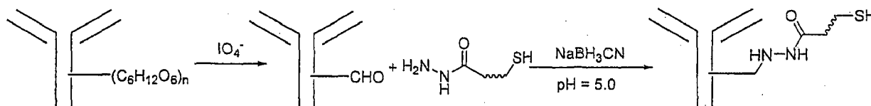
Scheme 11
