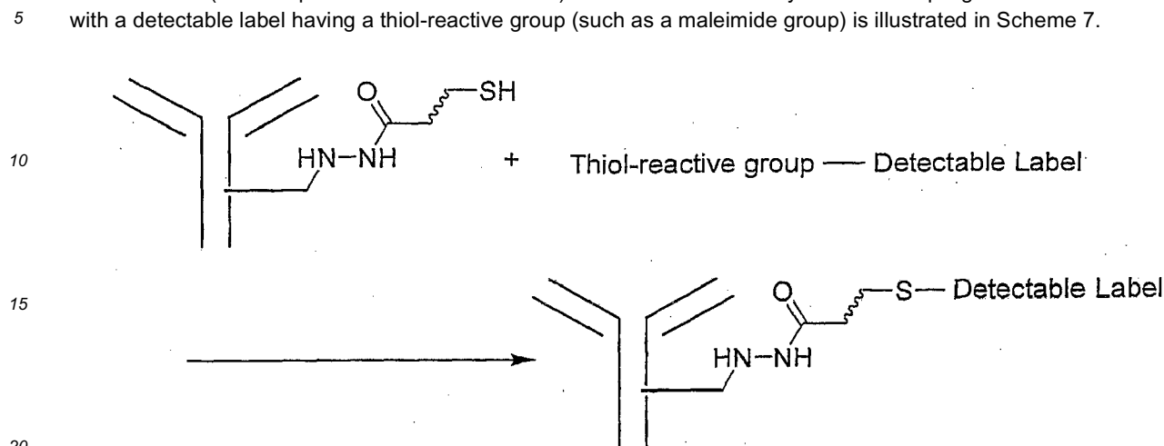
Scheme 7
