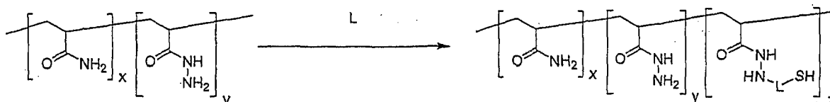
Scheme 19
