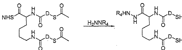
Scheme 4b
