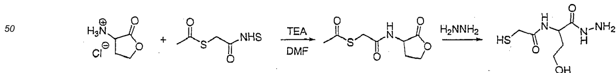
Scheme 17d
