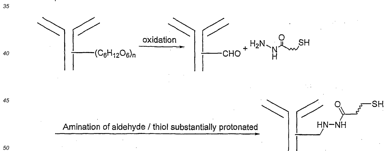
Scheme 6
