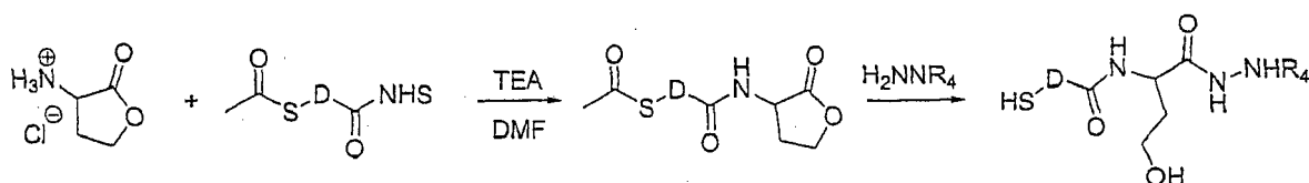
Scheme 4d
