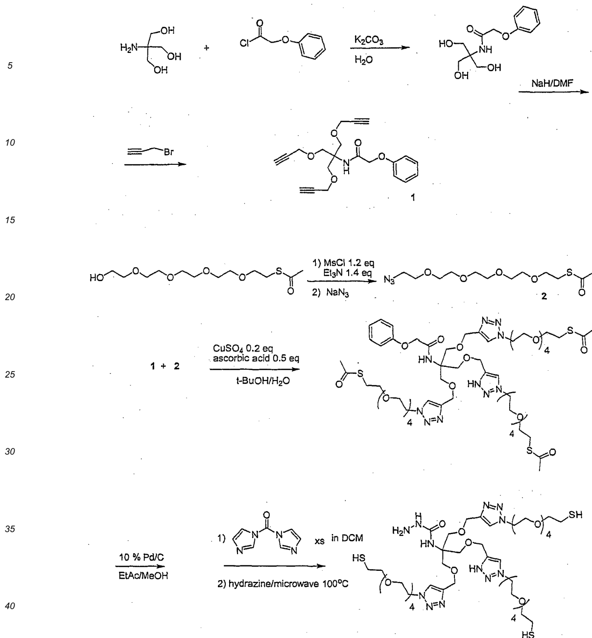
Scheme 18c
