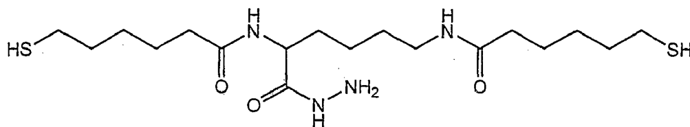
Bisthiohexanamidohydrazidolysine (BTHL)
