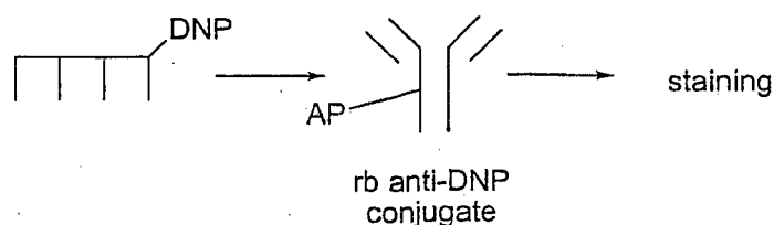
Scheme 16
