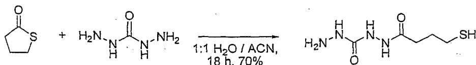
Scheme 9
