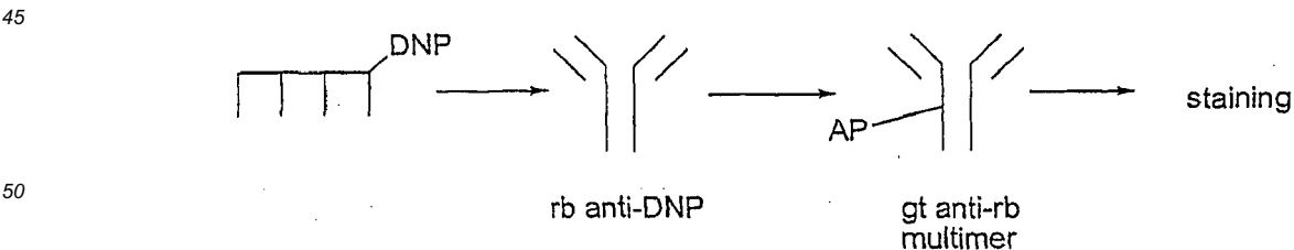
Scheme 14
