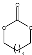
10. pentamethylene carbonate
