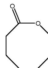
8. \xi -enthrolactone
