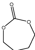
9. tetramethylene carbonate
