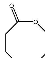
8. ξ-enantholactone
