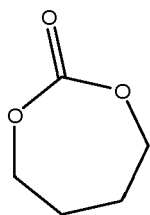
9. tetramethylene carbonate
