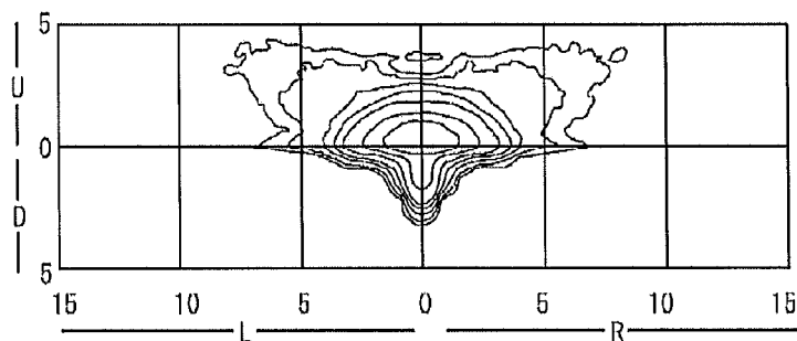
First exemplary light distribution pattern
