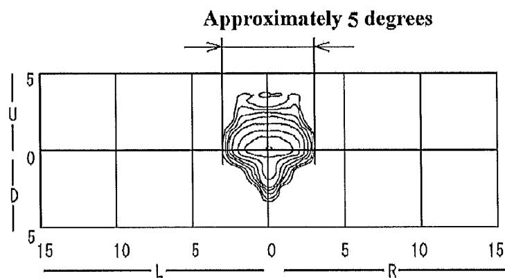
Second exemplary light distribution pattern
