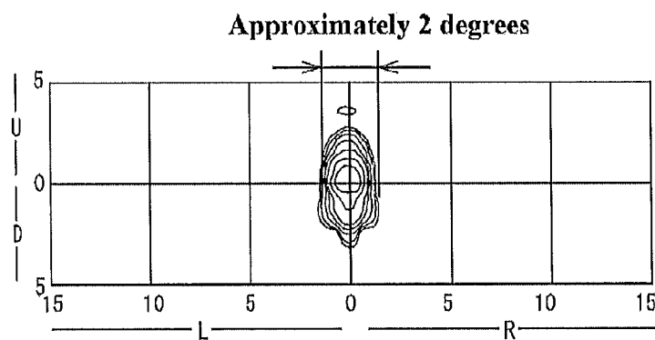
Third exemplary light distribution pattern
