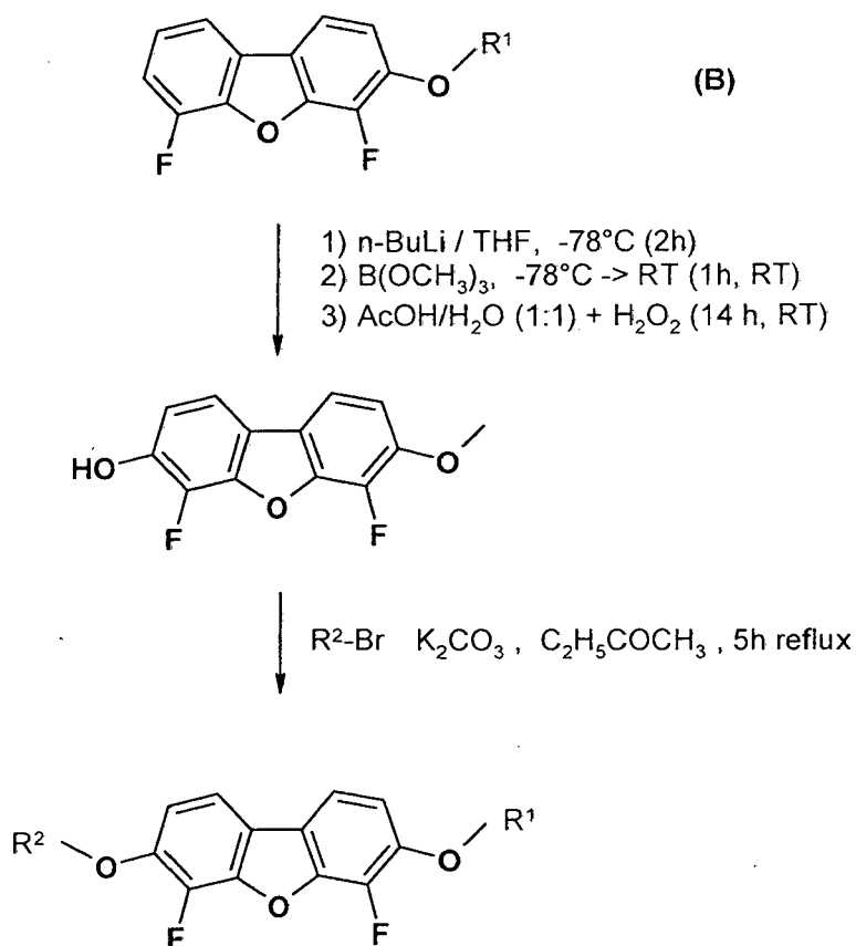
Scheme 1. Synthesis of the compounds of the formula I-1 with two alkoxy groups
