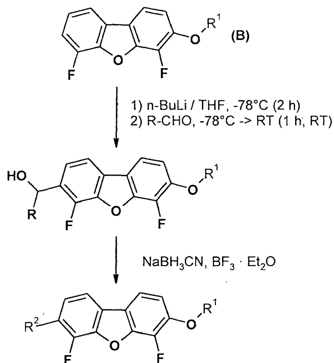
Scheme 2. Synthesis of the compounds of the formula I-1 with one alkyl and one alkoxy end group. The radical R corresponds to a radical such as R 2 correspondingly shortened by one carbon atom.
