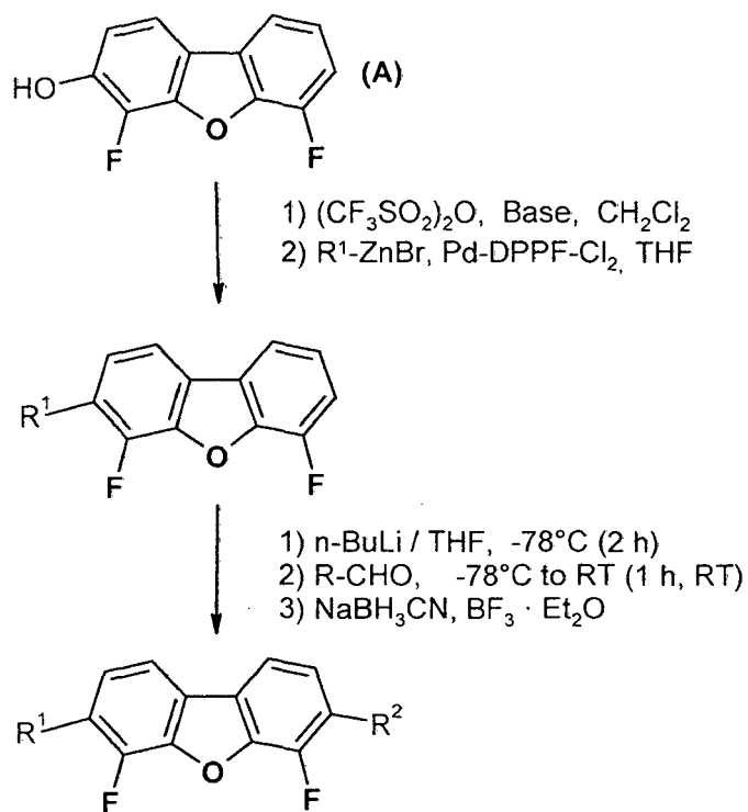
Scheme 3. Synthesis of the compounds of the formula I-1. The radical R of the aldehyde employed corresponds to a radical such as \text{R}^2 correspondingly shortened by one carbon atom.
