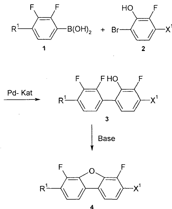
Scheme 4. Synthesis of the compounds of formula I-2.
