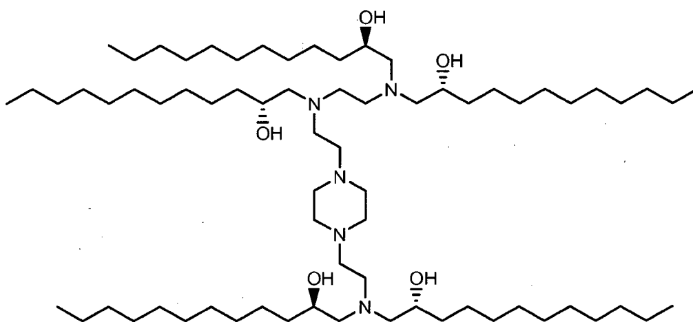
Major product, (R)-6
