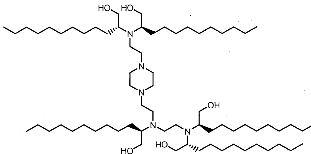
Minor product (one of 17 isomers)
