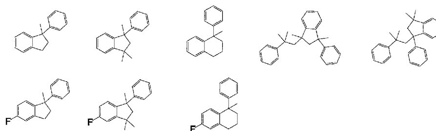
[Chem. 36]
