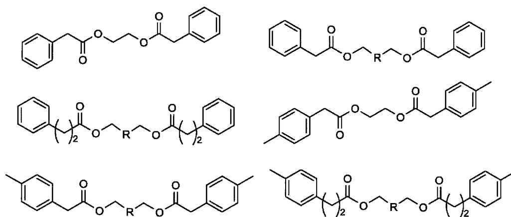
[Chem. 19]
