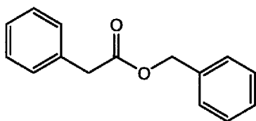
(Compound 2-1)
