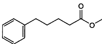
(Compound 1-3)
