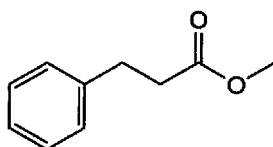
(Compound 1-2)
