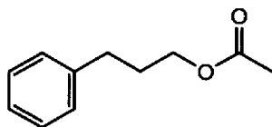
3-Phenylpropyl acetate
