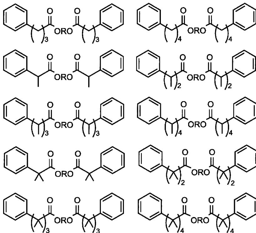
[Chem. 14]
