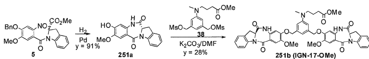
Figure 35. Synthetic scheme of dimer 251b (IGN-17-OMe).
