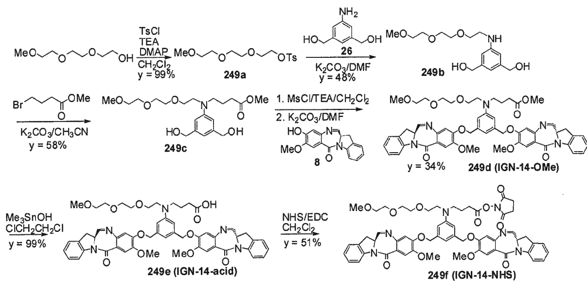
Figure 33. Synthetic scheme for indolinobenzodiazepine (IBD) dimers
