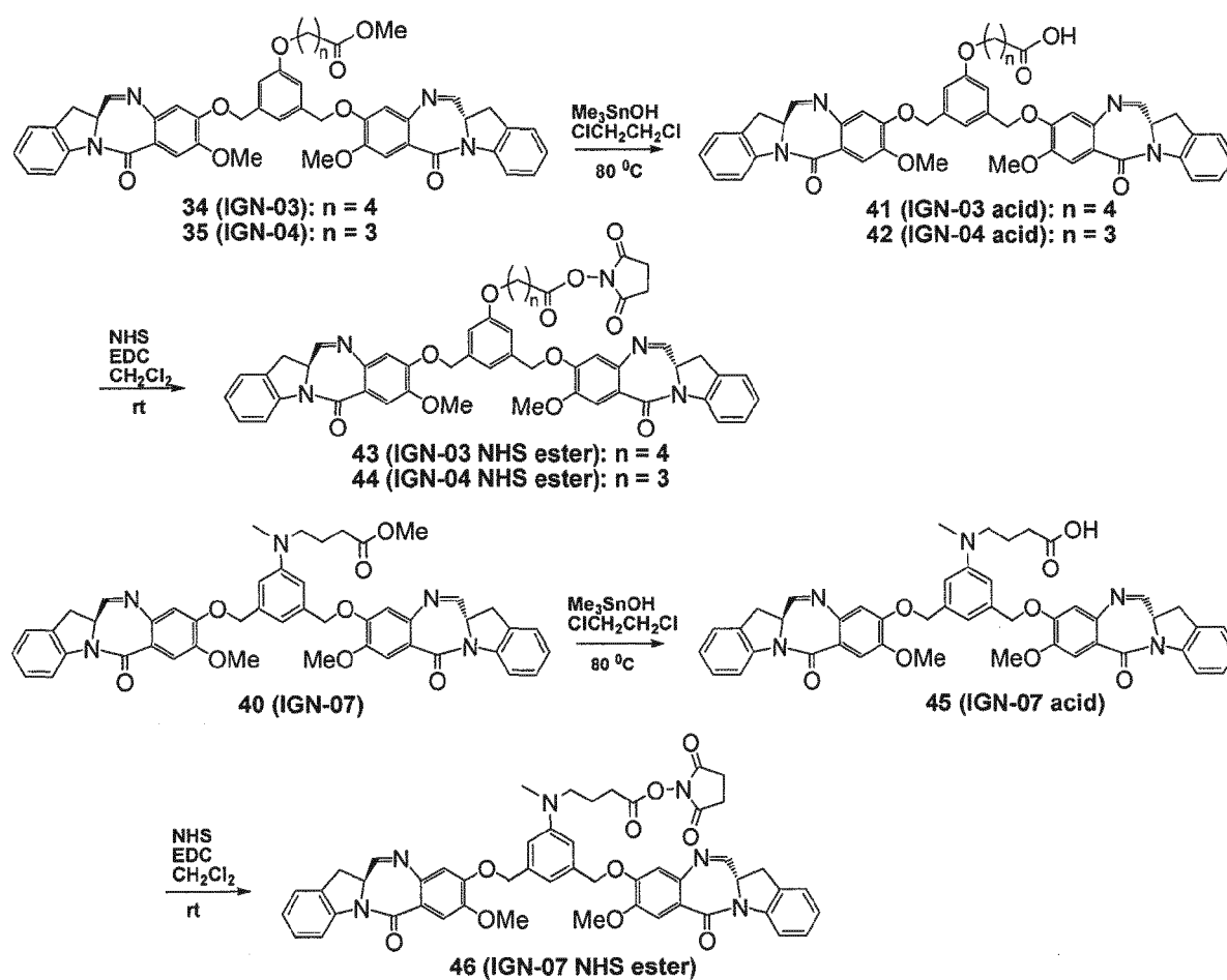
Figure 8. Synthetic scheme of the NHS esters 43 , 44 and 46
