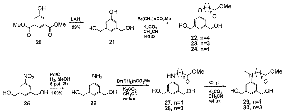
Figure 6. Synthetic scheme of the linkers
