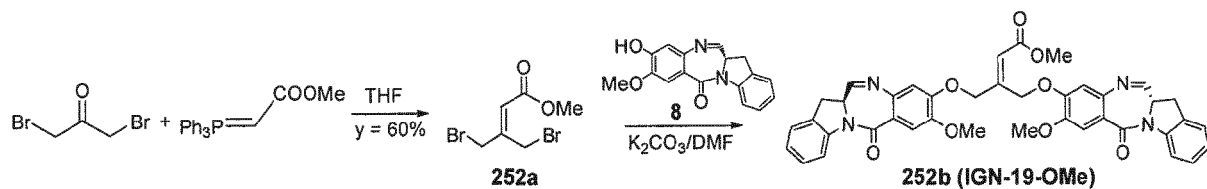
Figure 36. Synthetic scheme for dimer 252b (IGN-19-OMe).
