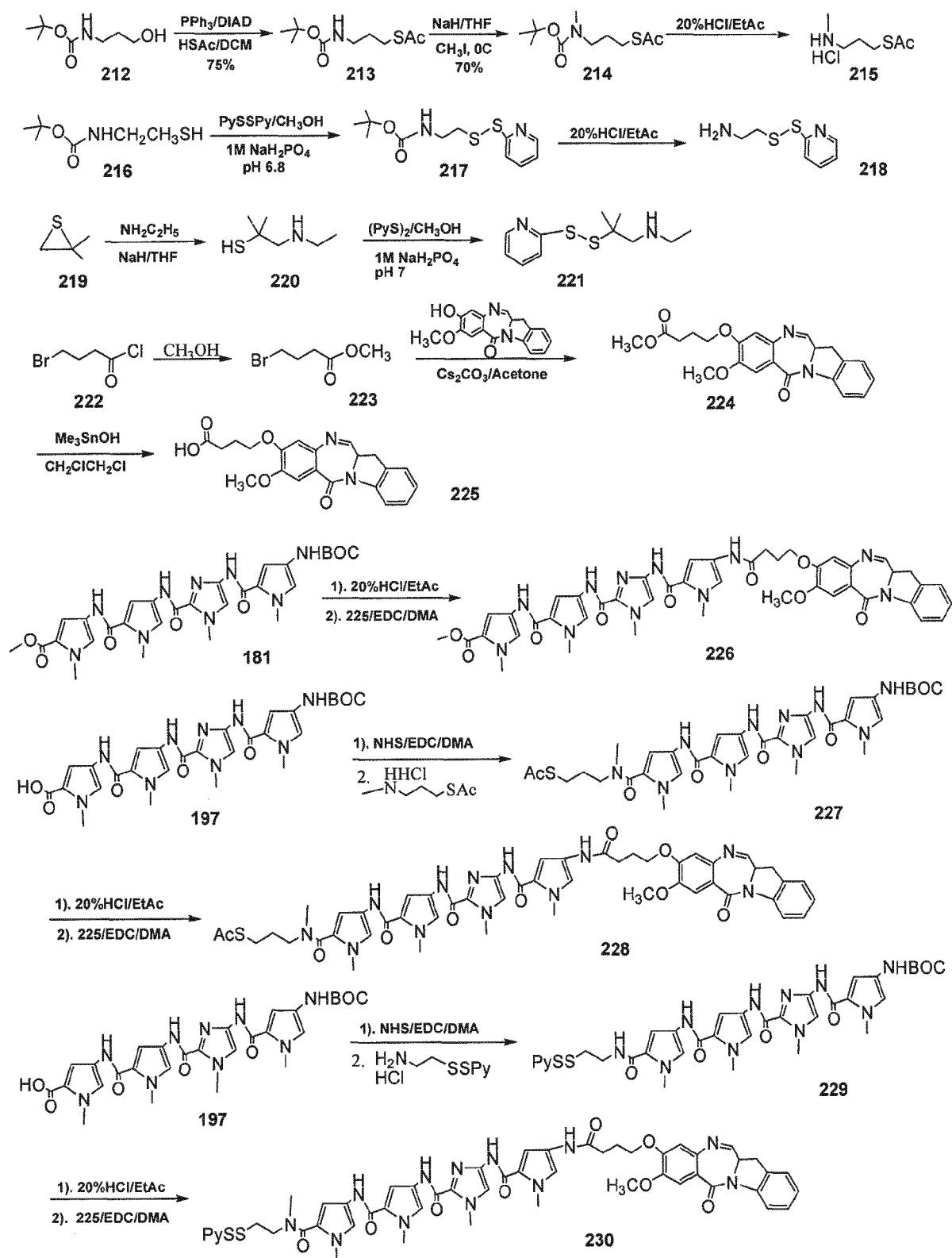
Figure 19. The synthesis of IBD-polypyrrole-imidazole analogs
