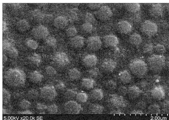
SEM photograph of the adhesive from Example 1
