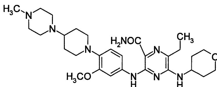
[Chem. 1]
