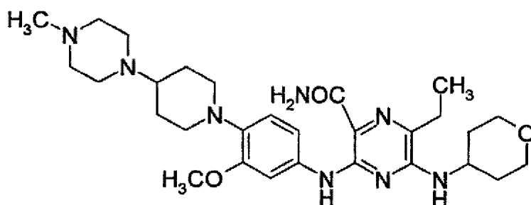
[Chem. 1]
