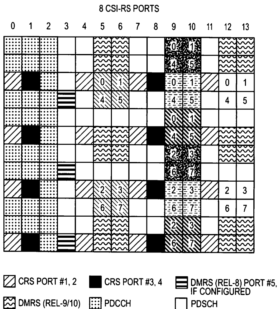
FIG. 8C (PRIOR ART)
