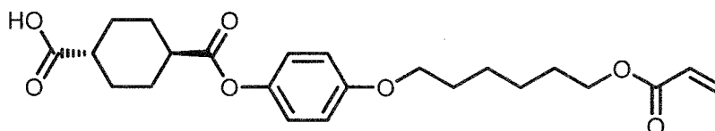
Intermediate C
