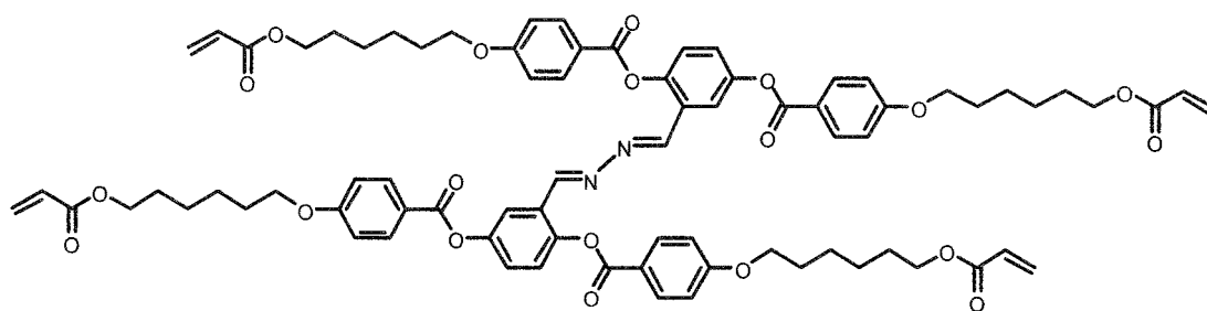
Compound \alpha
