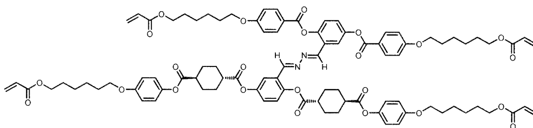
Compound 1
