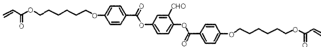
Intermediate E
