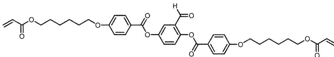
Intermediate B
