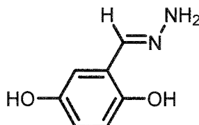
Intermediate A
