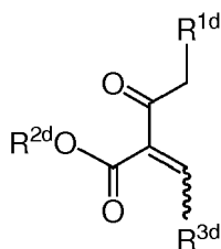
[Chemical formula 1]
