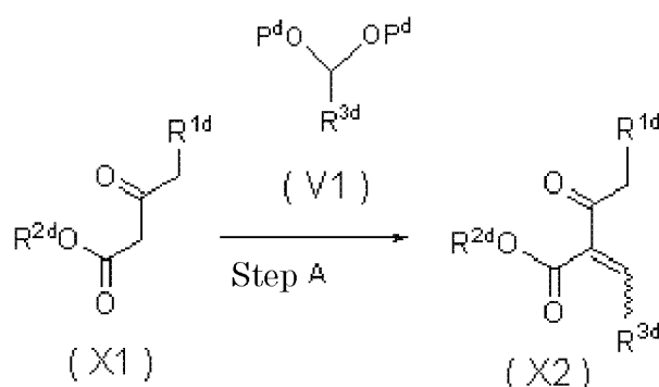
[Chemical formula 41]
