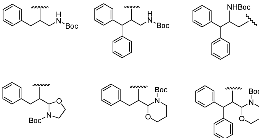
[Chemical formula 47]
