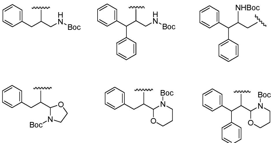
[Chemical formula 52]
