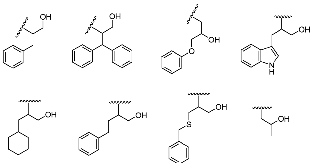
[Chemical formula 53]
