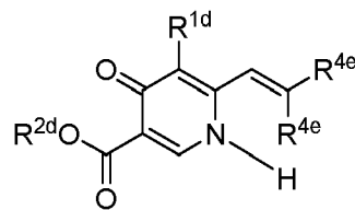
( XA4' )
