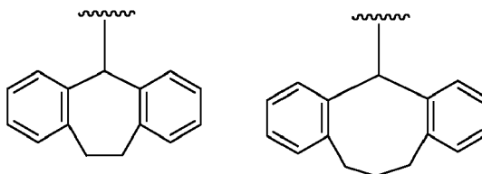
[Chemical formula 35]
