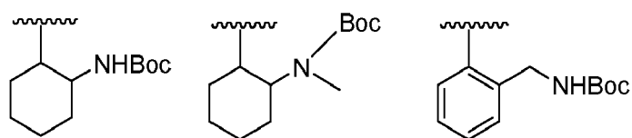
[Chemical formula 48]
