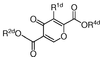
( X3 )
