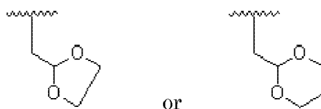
[Chemical formula 46]
