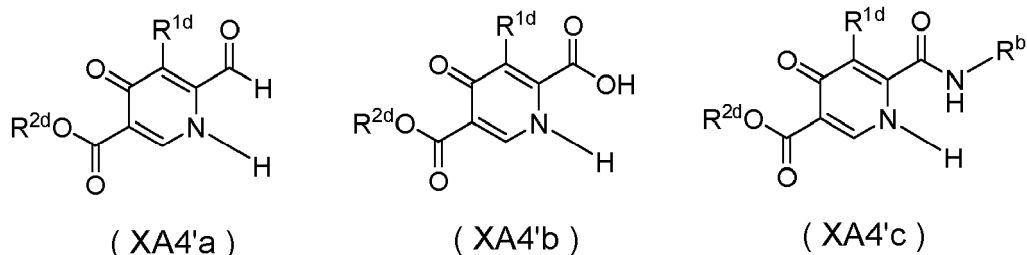
[Chemical formula 40]
