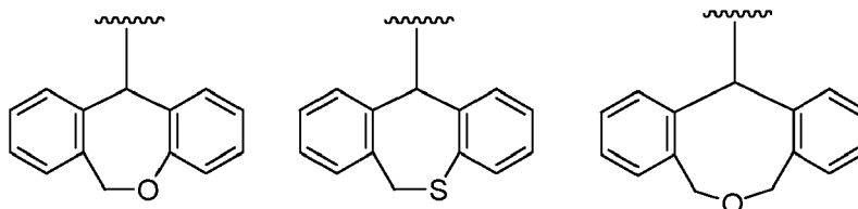
[Chemical formula 36]
