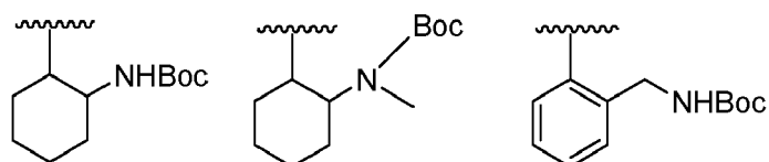
[Chemical formula 54]
