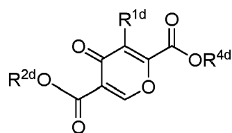
( X3 )
