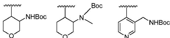
[Chemical formula 49]
