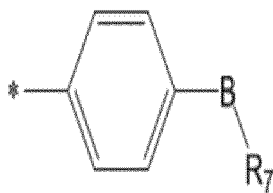
[Chemical Formula 3]
