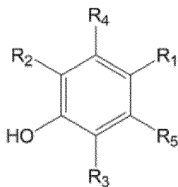
[Chemical Formula 1]
