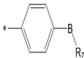
[Chemical Formula 3]
