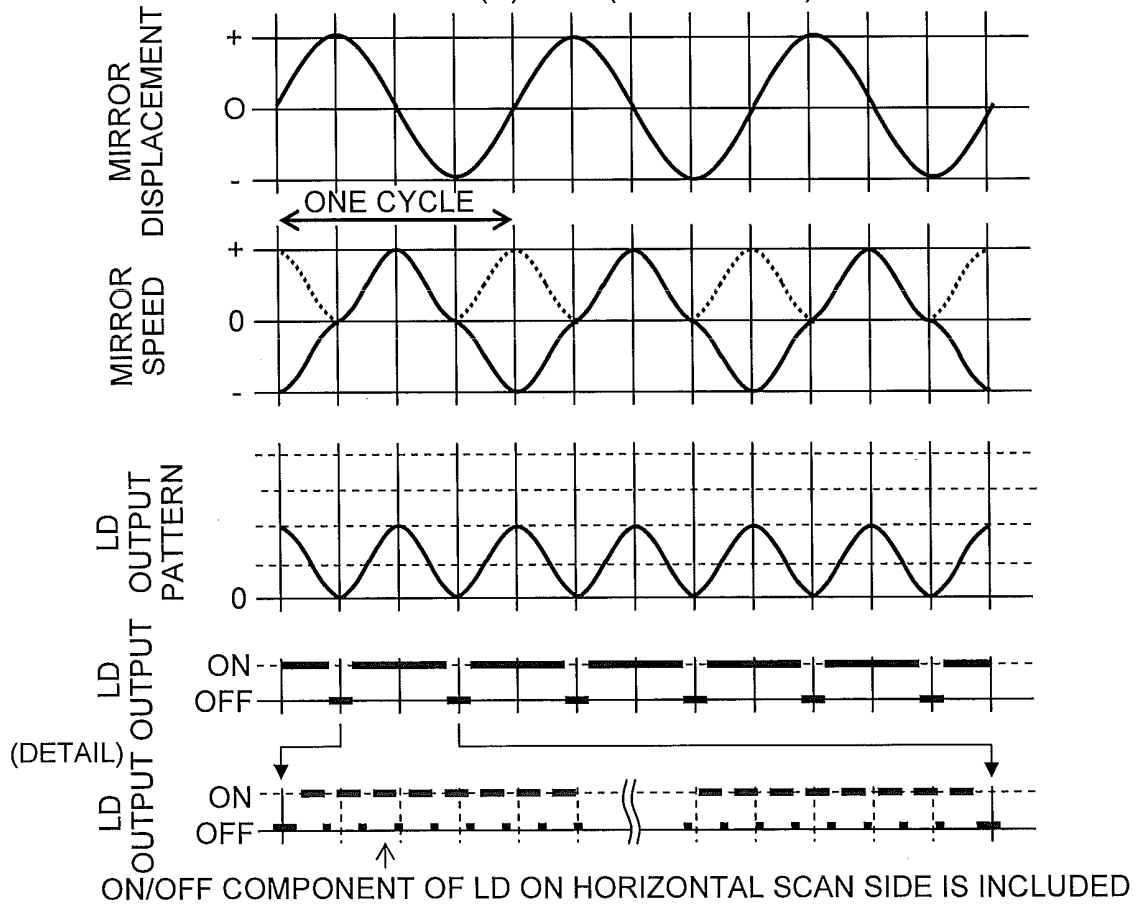
■ VERTICAL SCAN FREQUENCY ( f_v ): 12Hz(RESONANCE) FIG.18B
