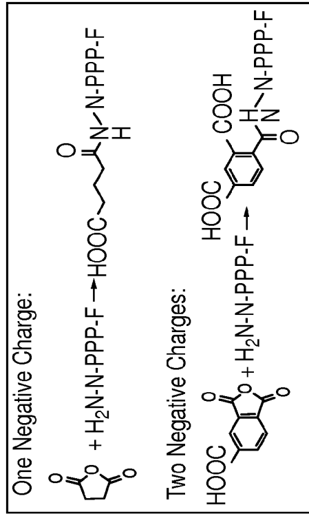
Scheme 9 - Add carboxylate to aminoallyl-dUTP
