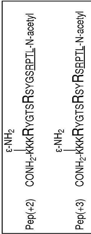
Scheme 7 - Peptide linkers (shown in C-to-N direction)
