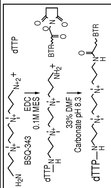
Scheme 6 - Coupling nucleotide, linker and dye
