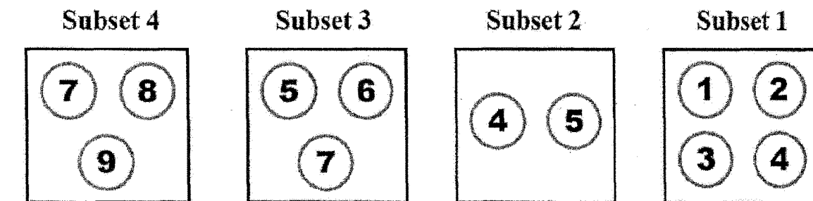
Caption Figure 6: Schematic of separating of 9 particle groups j = 1 \dots 9 with group average particle volumes V_j^{avg} into subsets according to volume ranges spanning four orders of magnitude (factor of 10,000). In this case, the super-set \{i\} of all subsets contains 4 subsets, \{1,2,3,4\}_1 , \{4,5\}_2 , \{5,6,7\}_3 , and \{7,8,9\}_4 .
