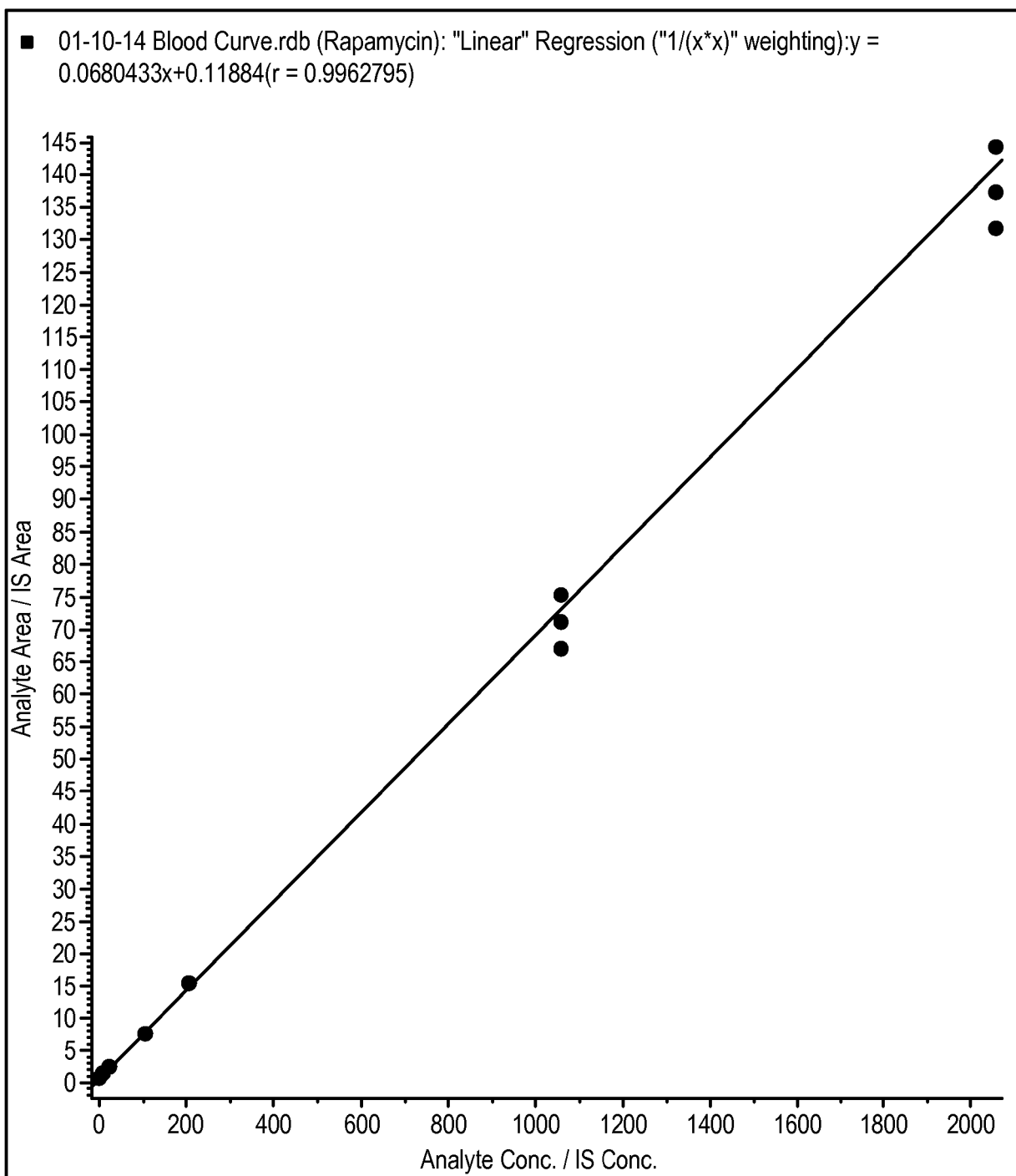
Calibration Curve for Rapamycin in Mouse Blood
