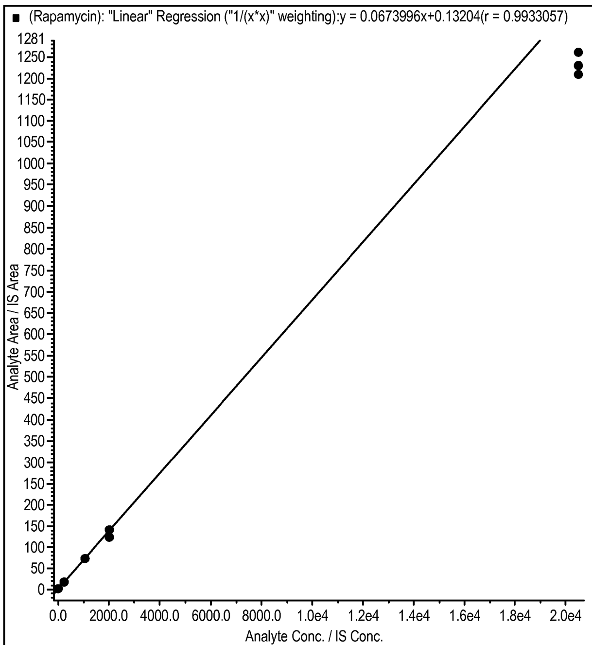
Calibration Curve for Rapamycin in Mouse Lung Homogenate
