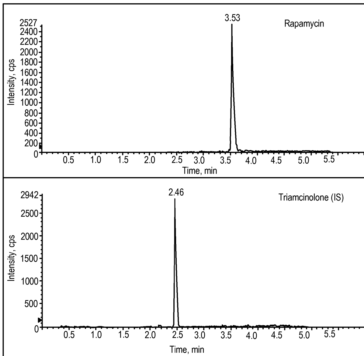
LC-MS/MS Chromatogram of 10.6 ng/mL Rapamycin (top) and Internal Standard (bottom) in Mouse Blood
