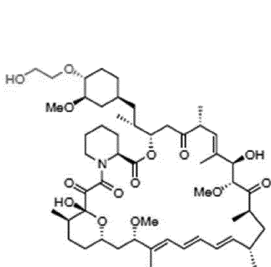
Everolimus (Affinitor)
