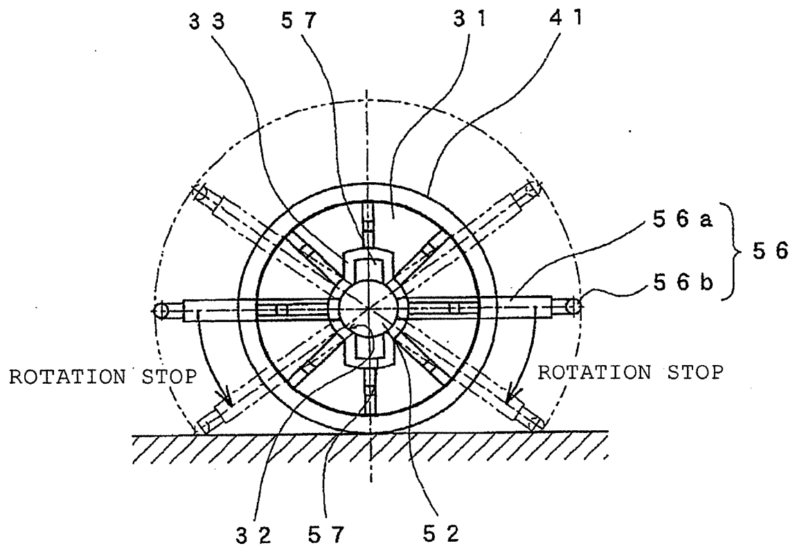
ROTATION STOP STATE REFERENCE DIAGRAM
