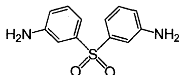
3,3'-diaminodiphenylsulfone
