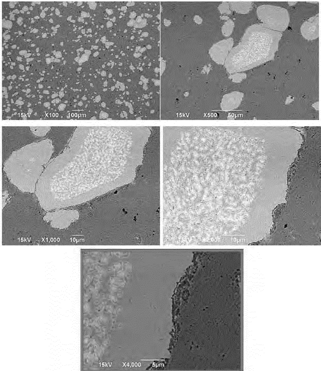
Field of View of SEM-EDX Analysis
