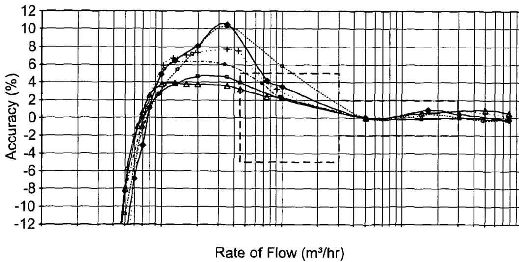
Meter Performance versus Ring Diameter
