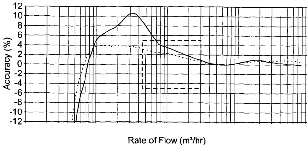
Meter Performance - Ring versus No Ring
