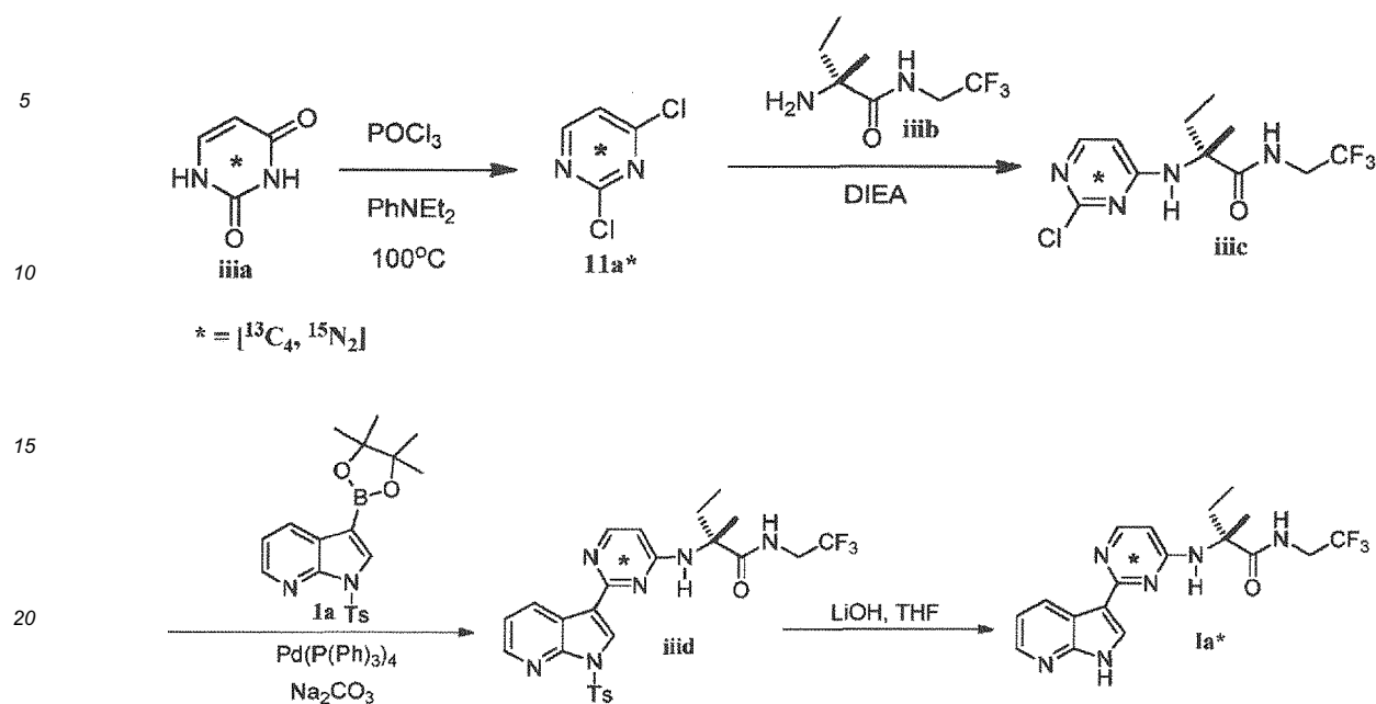
Scheme III
