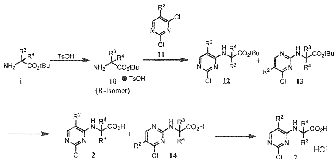
Scheme Ib:
