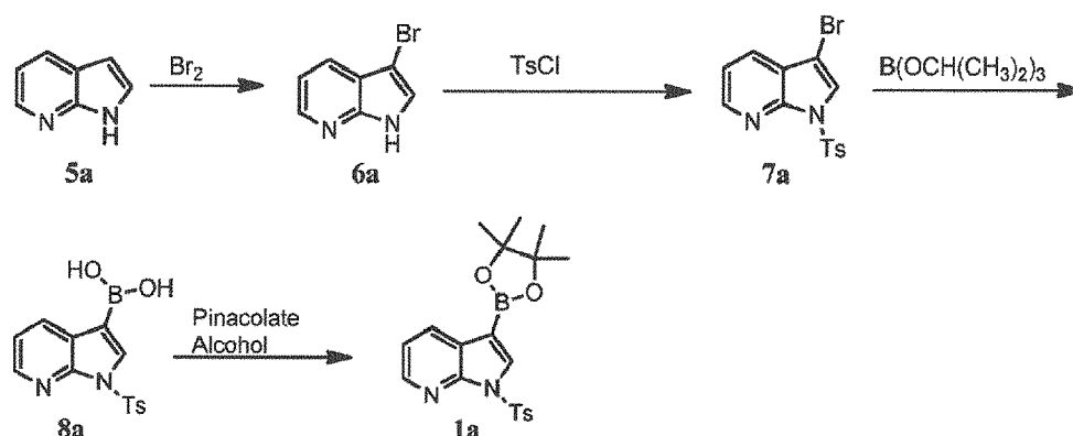
Scheme IIa:
