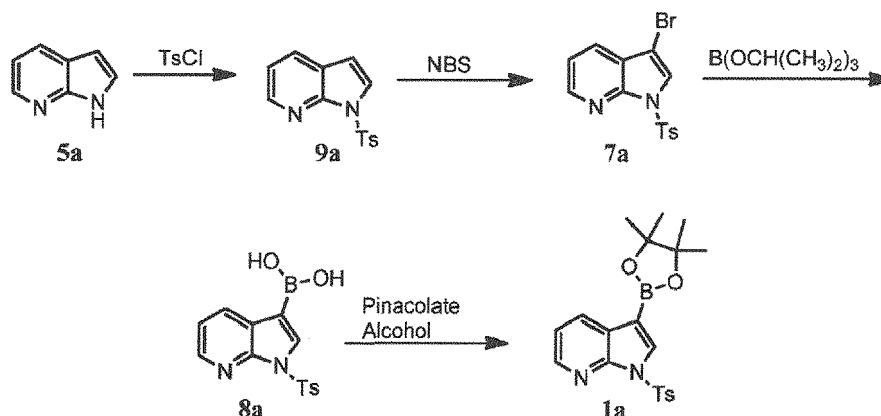
Scheme IIb:
