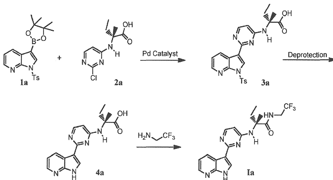
Scheme IIc:
