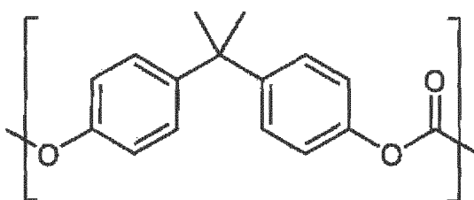
[Chemical Formula 4-1]
