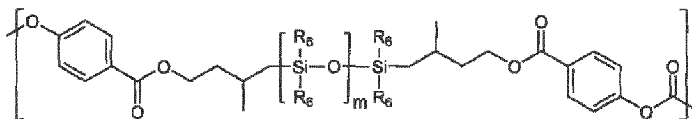
[Chemical Formula 3-2]
