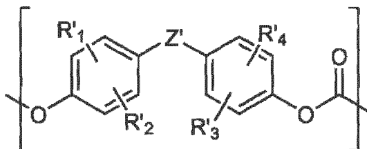
[Chemical Formula 4]
