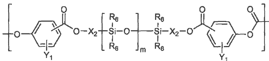
[Chemical Formula 3]
