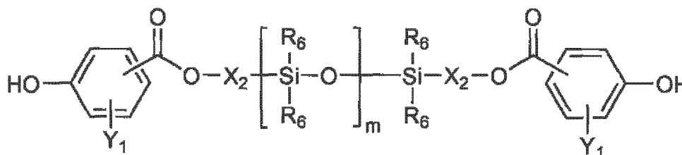
[Chemical Formula 3-1]
