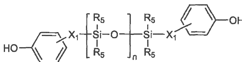
[Chemical Formula 2-1]
