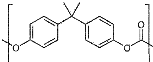
[Chemical Formula 1-1]
