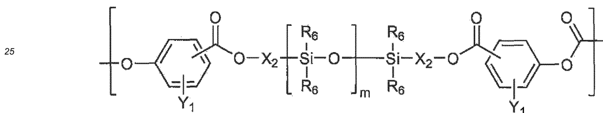
[Chemical Formula 3]
