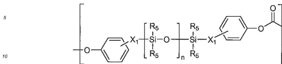
[Chemical Formula 2]
