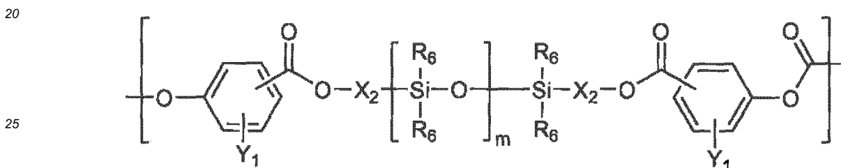
[Chemical Formula 3]
