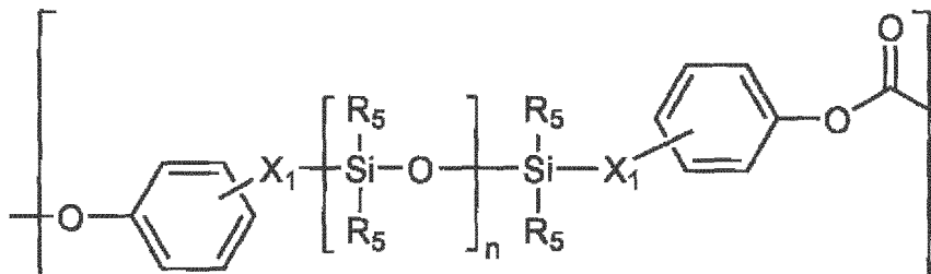
[Chemical Formula 2]
