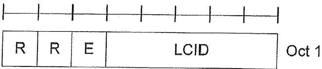
R/R/E/LCID sub-header
