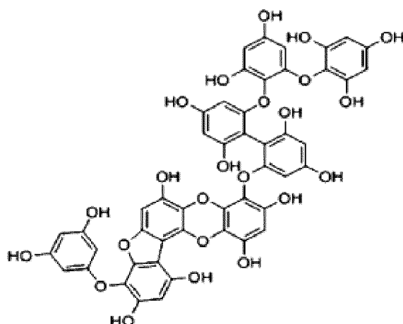
[Chemical Formula 5]
