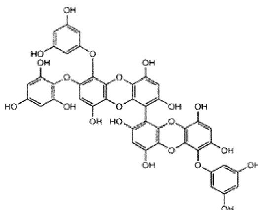
[Chemical Formula 1]
