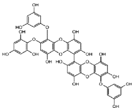
[Chemical Formula 1]
