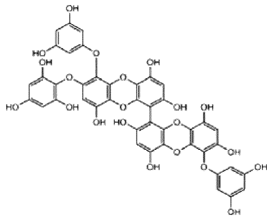
[Chemical Formula 2]
