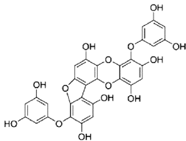
[Chemical Formula 4]
