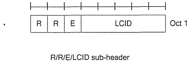
FIG. 15 (PRIOR ART)
