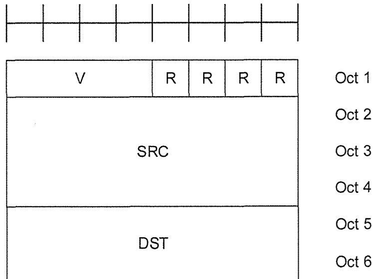
FIG. 16 (PRIOR ART)
