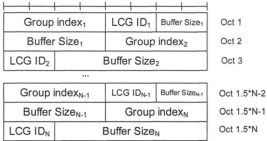
FIG. 12 (PRIOR ART)
