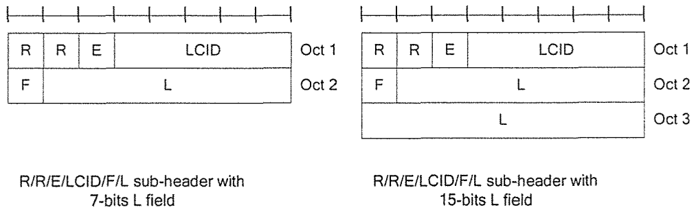
FIG. 14 (PRIOR ART)
