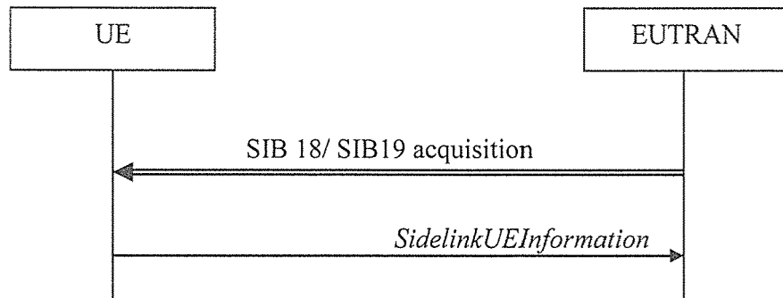
FIG. 11 (PRIOR ART)
