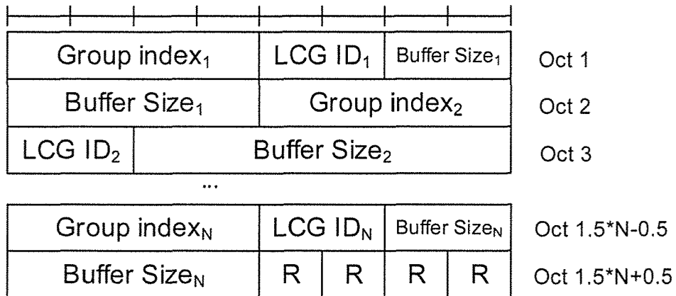
FIG. 13 (PRIOR ART)
