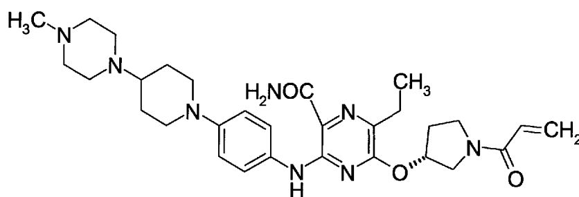
[Chem. 1]
