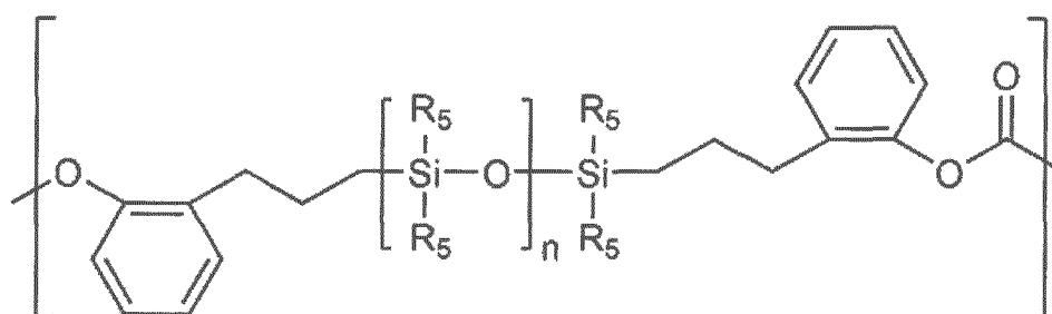
[Chemical Formula 2-2]
