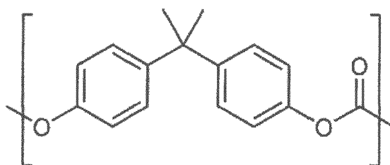
[Chemical Formula 4-1]
