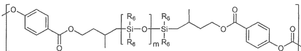
[Chemical Formula 3-2]
