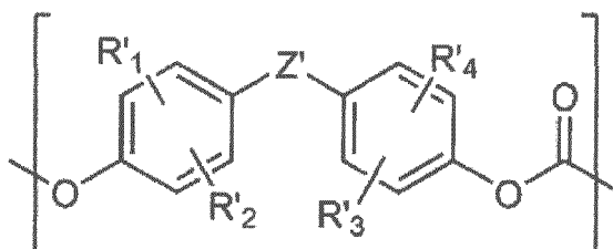
[Chemical Formula 4]
