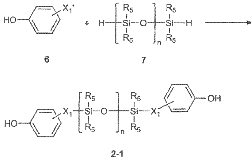
[Reaction Scheme 1]
