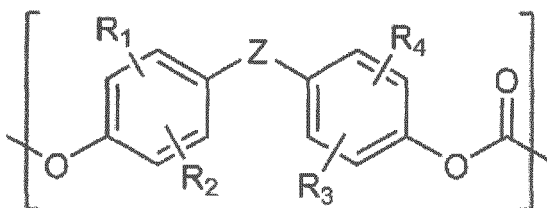
[Chemical Formula 1]
