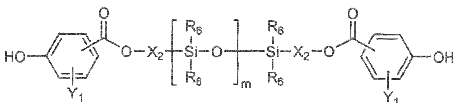
[Chemical Formula 3-1]
