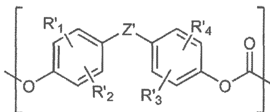
[Chemical Formula 4]
