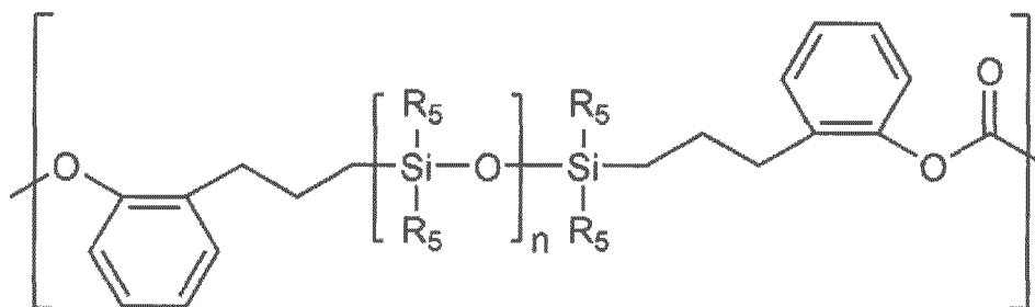
[Chemical Formula 2-2]
