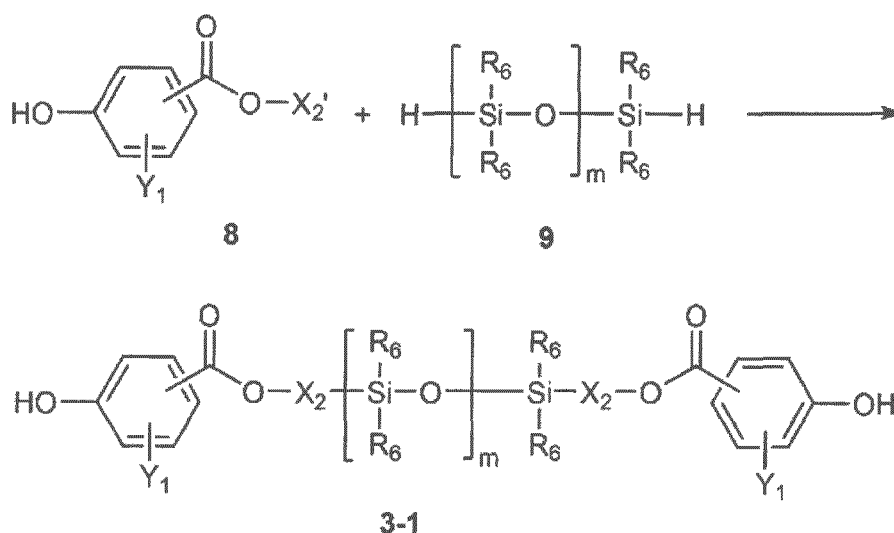
[Reaction Scheme 2]
