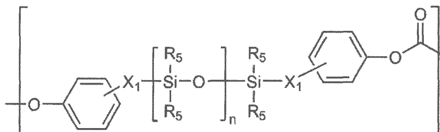
[Chemical Formula 2]
