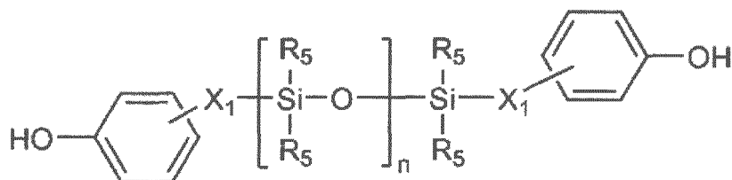
[Chemical Formula 2-1]
