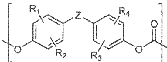
[Chemical Formula 1]
