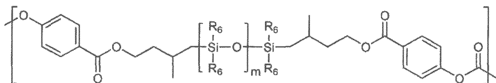
[Chemical Formula 3-2]
