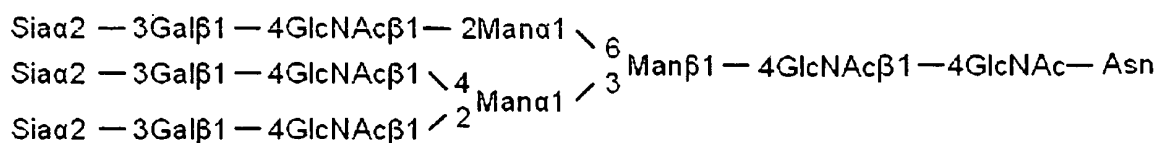
structural formula 1
