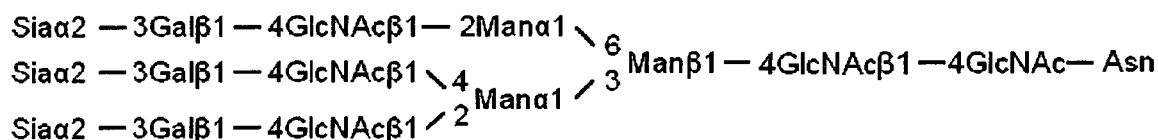
structural formula 1
