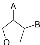
TRANS- single stereoisomer a
