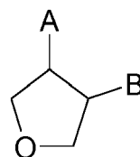
TRANS- single stereoisomer b
