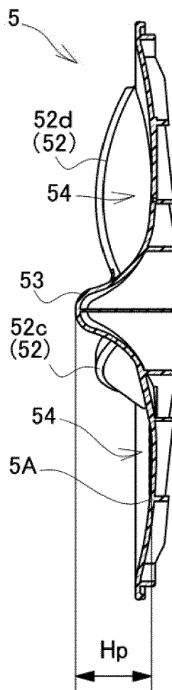
(b) B-B section
