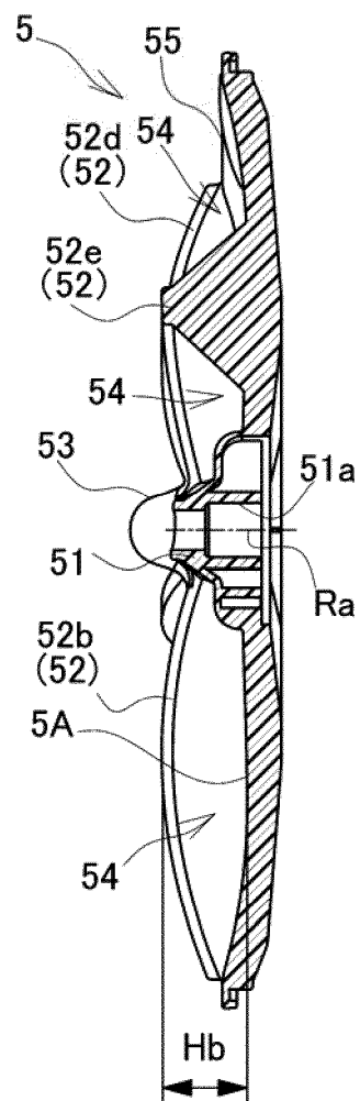
(c) C-C section
