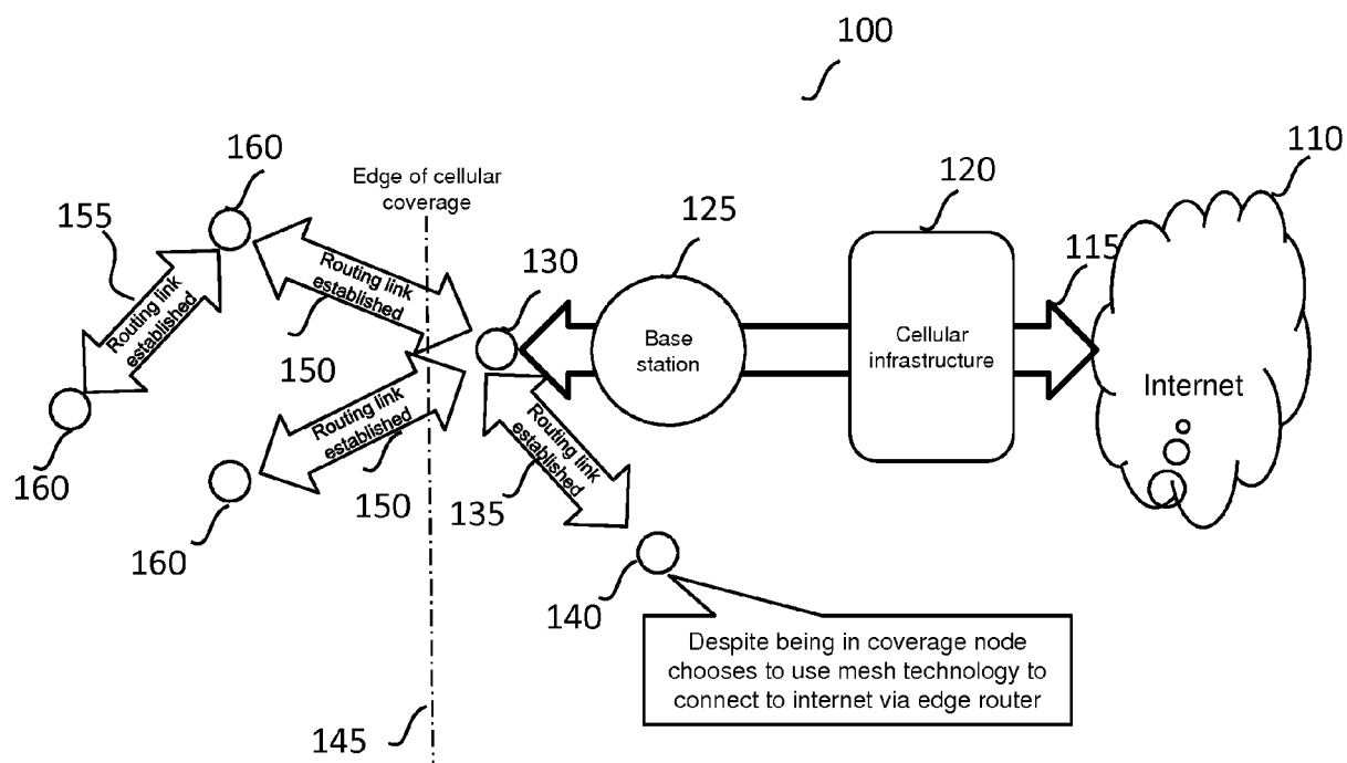
FIG. 1 - Prior Art
