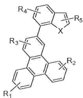
Compound 12G
