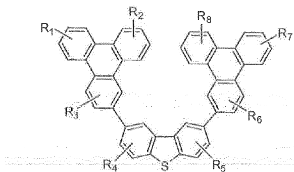
Compound 5'G
