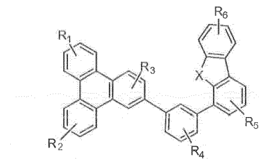
Compound 2G
