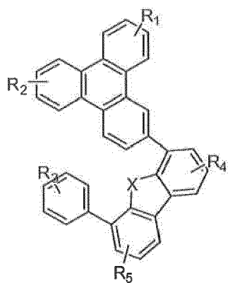
Compound 29G
