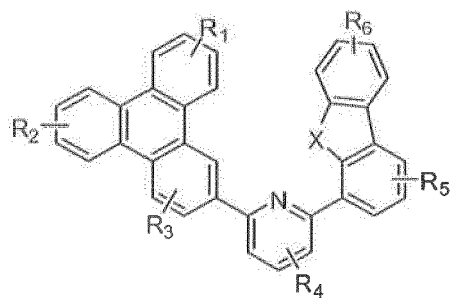
Compound 22 G
