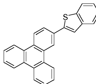
Compound 14'
