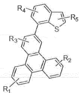
Compound 12'G
