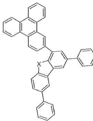
Compound 31
