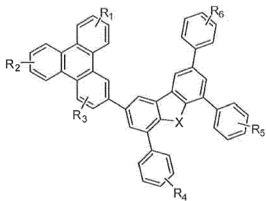
Compound 35G
