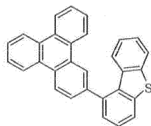
Compound 7'
