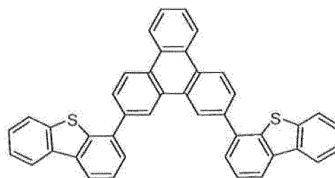
Compound 10'
