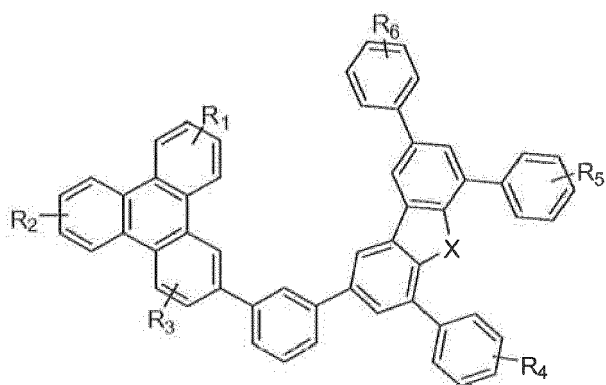
Compound 35G
