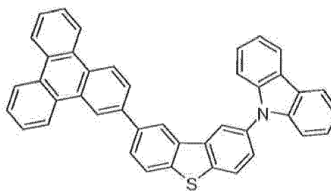
Compound 15'
