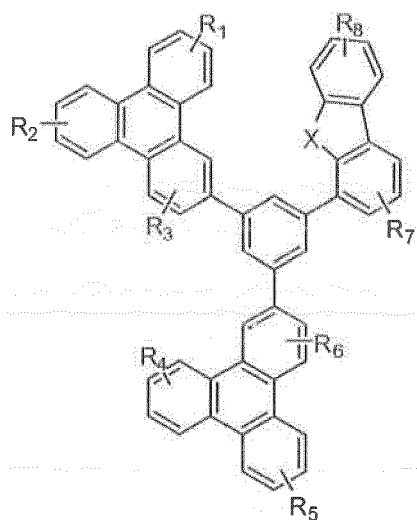
Compound 38G
