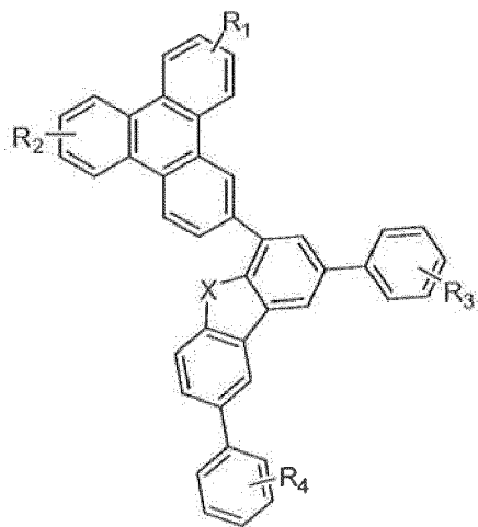
Compound 31G
