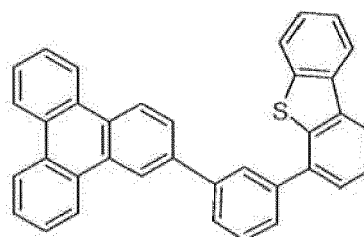
Compound 2'
