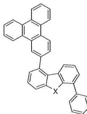
Compound 30
