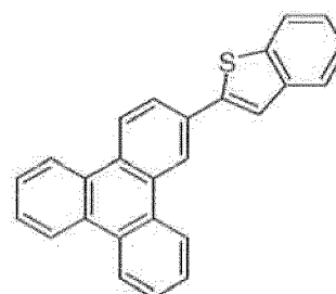
Compound 14'
