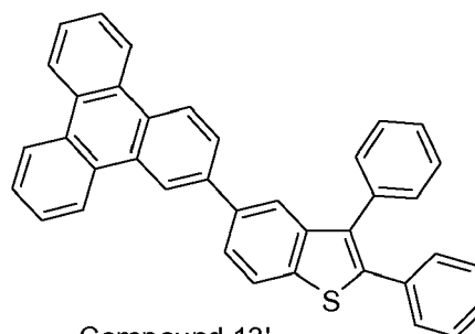
Compound 13'
