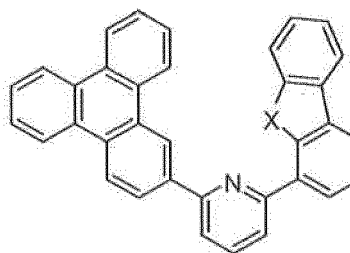
Compound 22
