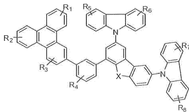
Compound 27G
