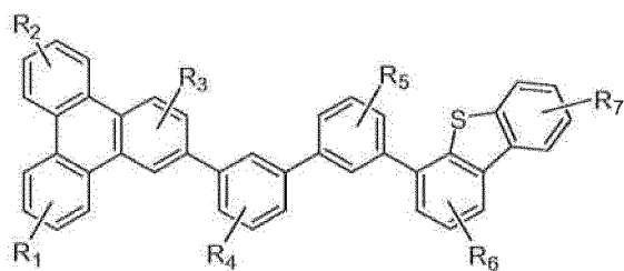
Compound 9'G
