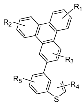
Compound 16'G
