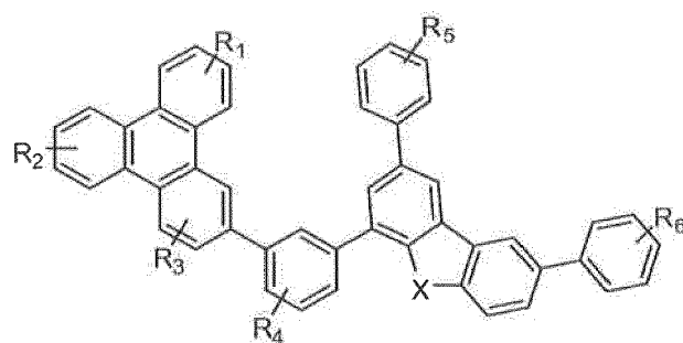
Compound 24 G
