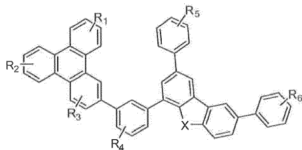
Compound 24 G
