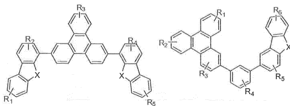
Compound 19 G
