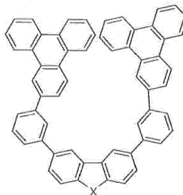
Compound 39
