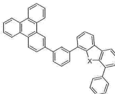
Compound 23
