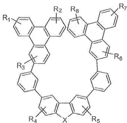
Compound 39G
