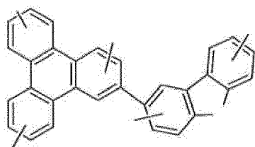
Compound 40G
