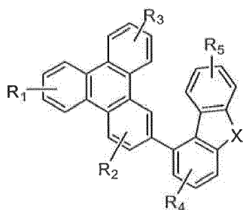
Compound 7G
