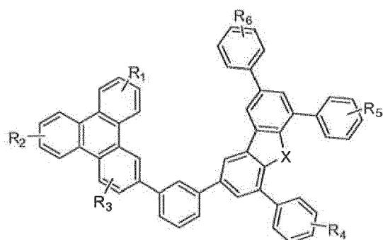
Compound 36G
