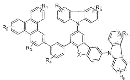
Compound 27 G
