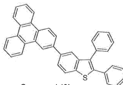
Compound 13'
