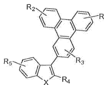
Compound 18G
