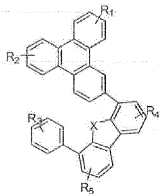
Compound 29G
