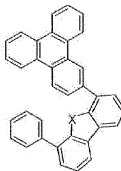
Compound 29
