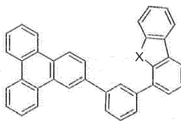
Compound 2
