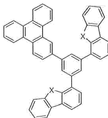
Compound 36
