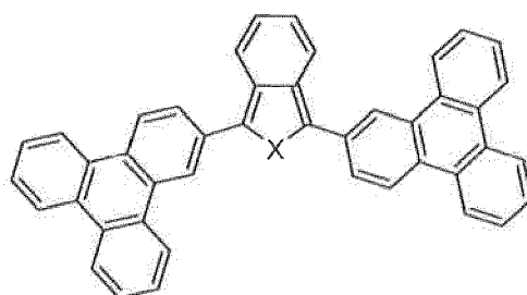
Compound 11
