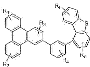
Compound 3'G
