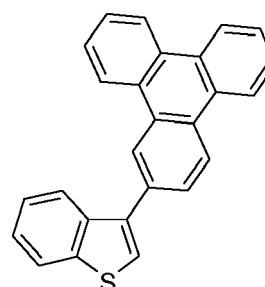
Compound 18'
