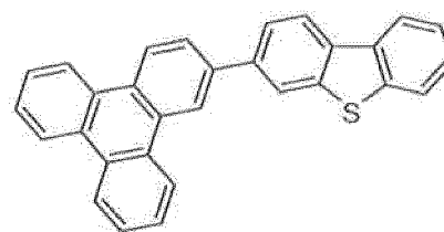
Compound 8'
