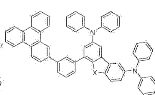
Compound 28
