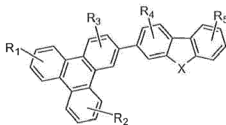
Compound 8G
