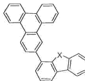
Compound 1
