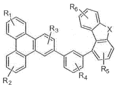
Compound 3G
