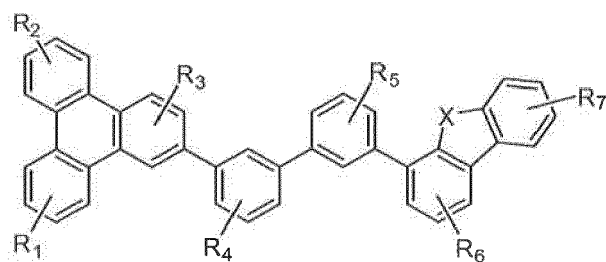
Compound 9G
