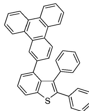
Compound 16'
