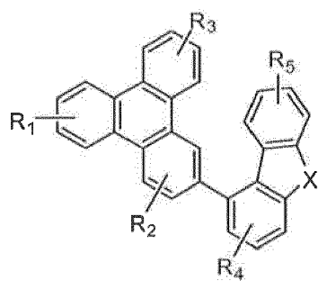
Compound 7G
