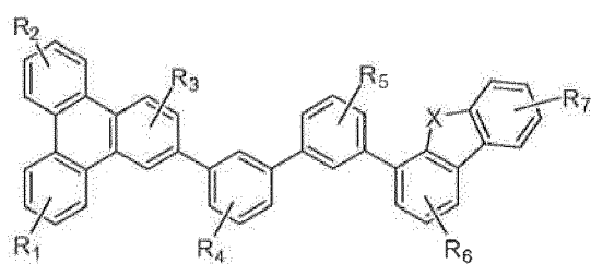
Compound 9G
