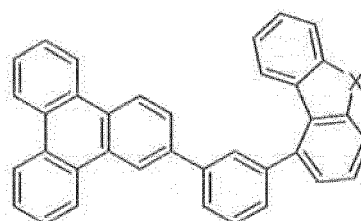
Compound 3
