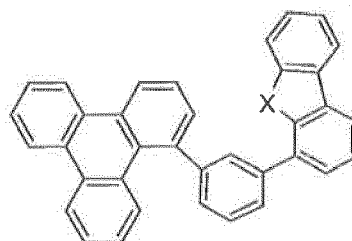
Compound 33
