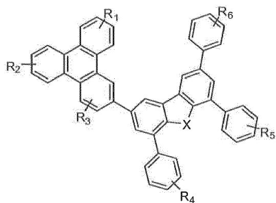
Compound 35G
