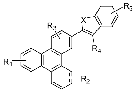
Compound 14G
