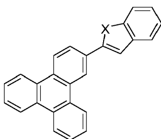
Compound 14
