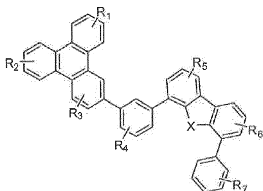
Compound 23 G
