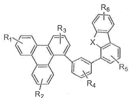
Compound 33G
