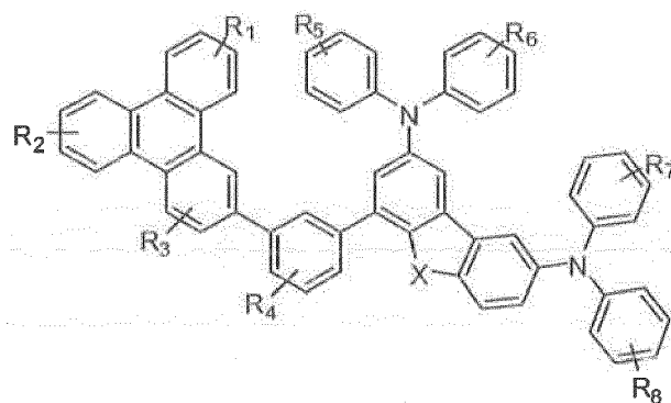
Compound 28G
