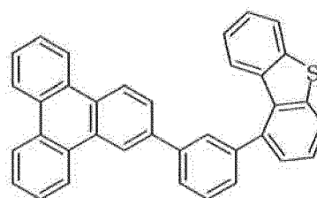
Compound 3'
