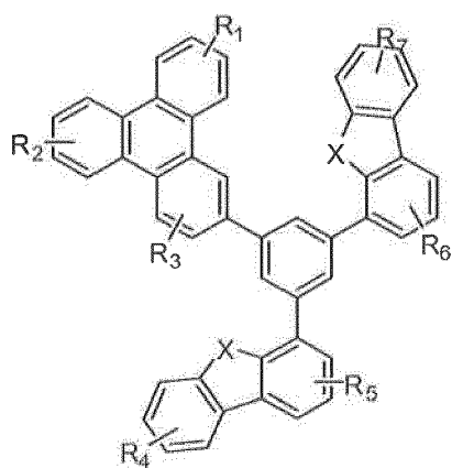
Compound 36G
