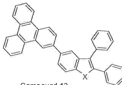
Compound 13
