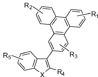
Compound 18G
