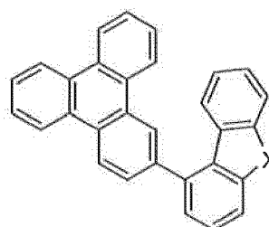
Compound 7
