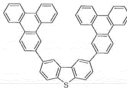
Compound 5'
