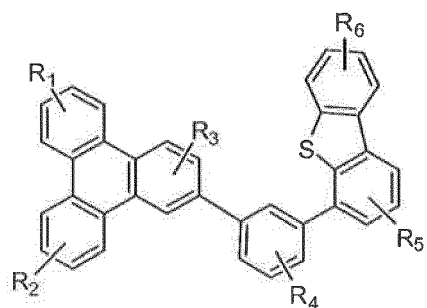
Compound 2'G
