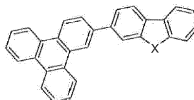
Compound 8
