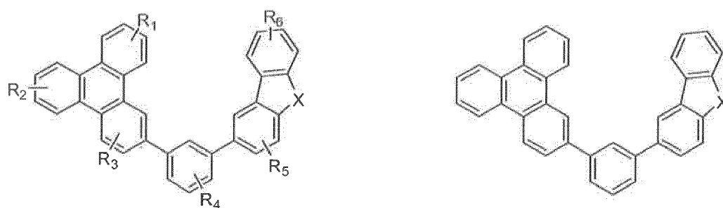
Compound 20
