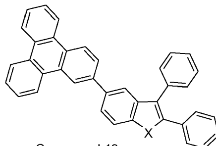
Compound 13
