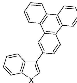
Compound 18
