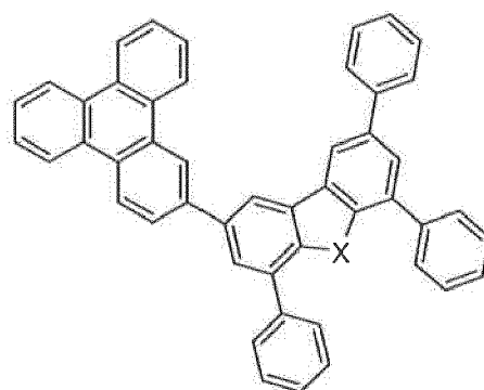
Compound 35
