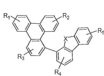
Compound 34G
