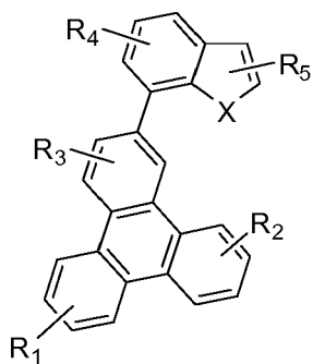
Compound 12G
