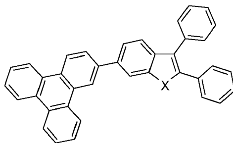
Compound 17
