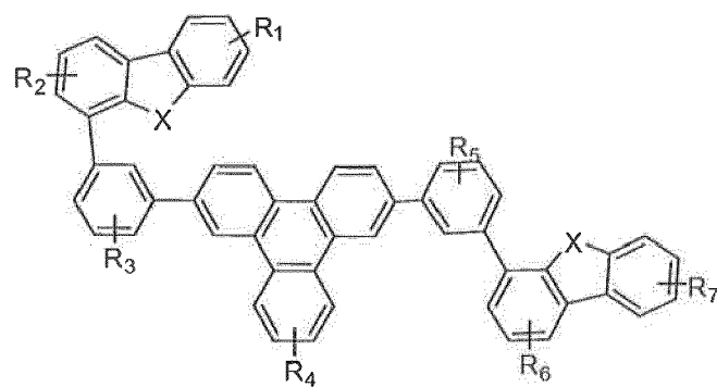
Compound 26G
