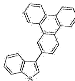
Compound 18'
