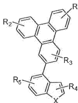
Compound 16G
