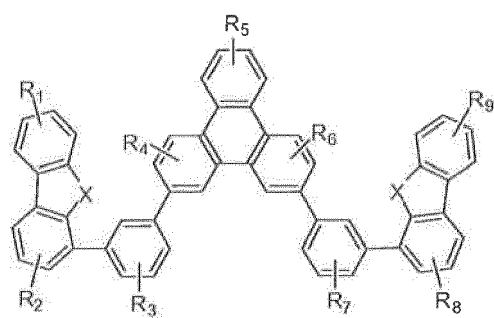
Compound 4G
