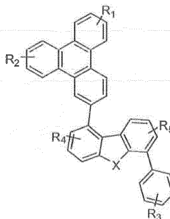
Compound 30G
