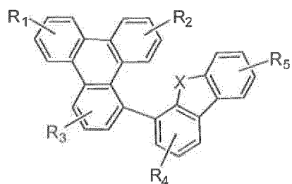
Compound 34G
