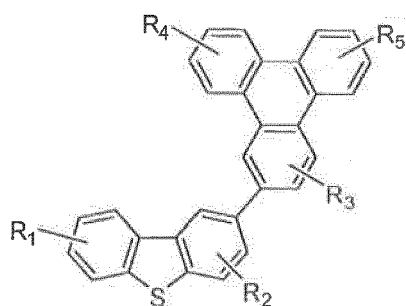
Compound 6'G
