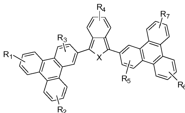
Compound 11G
