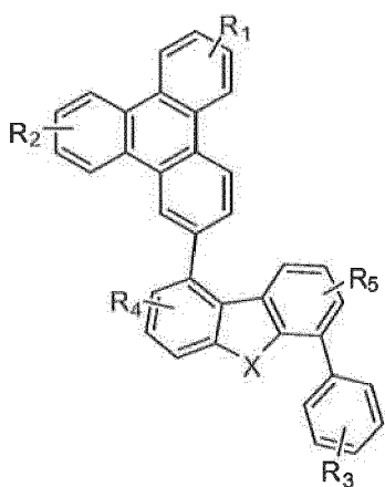
Compound 30G
