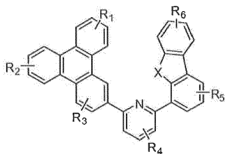
Compound 22 G
