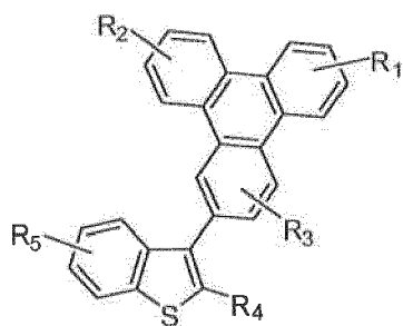
Compound 18'G
