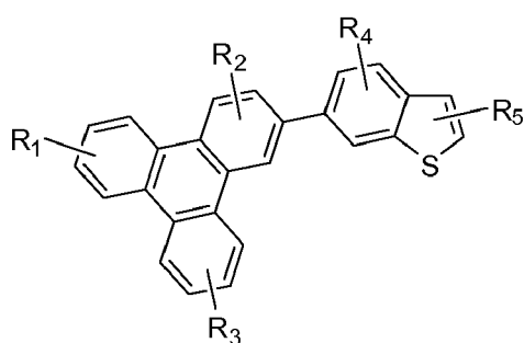
Compound 17'G
