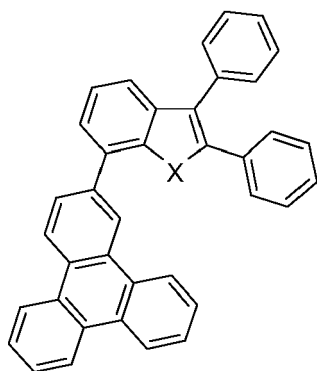
Compound 12
