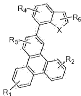
Compound 12G
