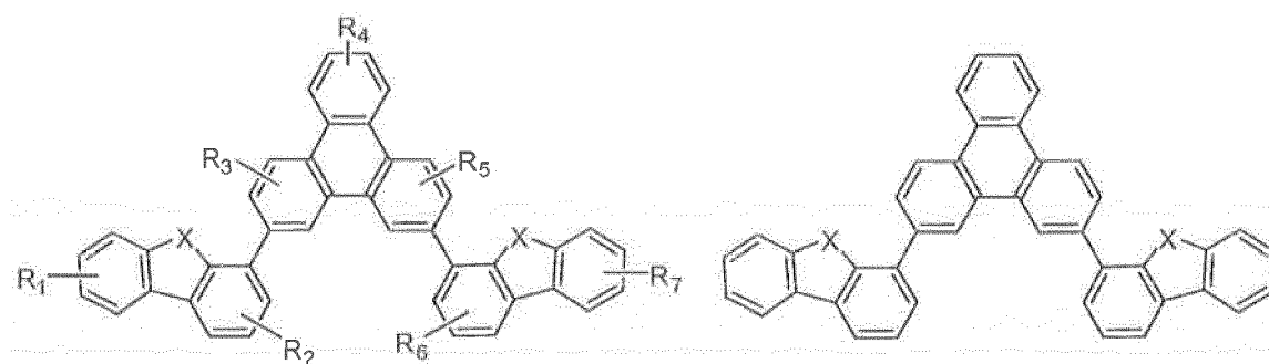
Compound 10G
