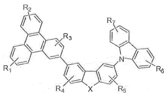
Compound 15G
