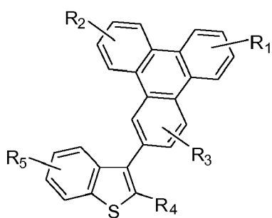
Compound 18'G
