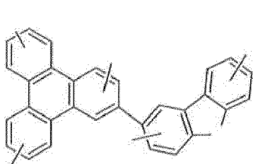
Compound 39G
