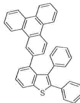
Compound 16'
