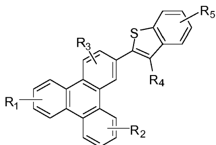
Compound 14'G
