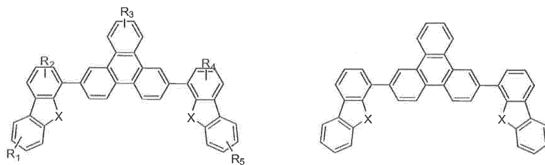
Compound 19 G
