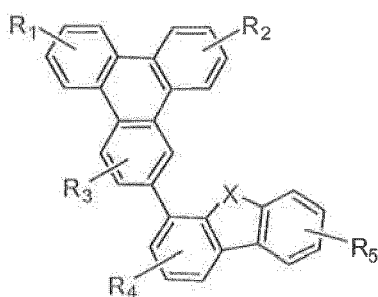
Compound 1G
