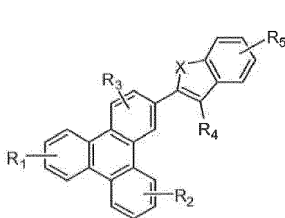
Compound 14G
