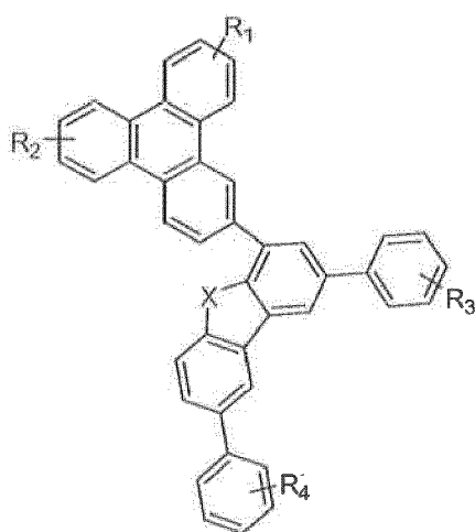
Compound 31G
