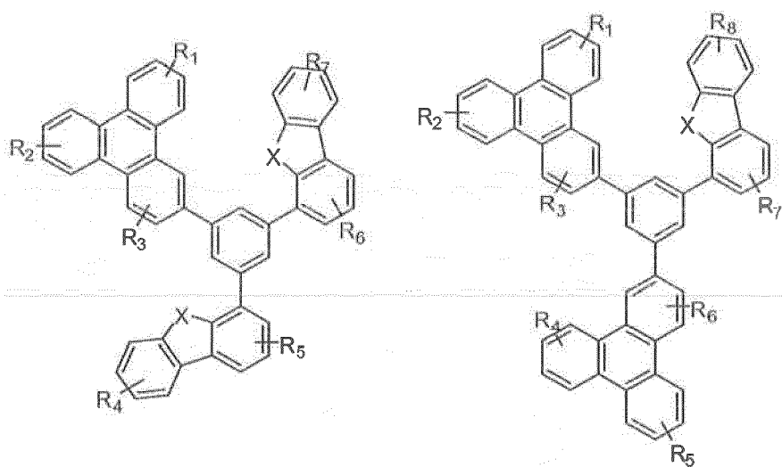
Compound 37G
