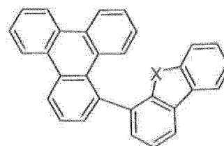
Compound 34
