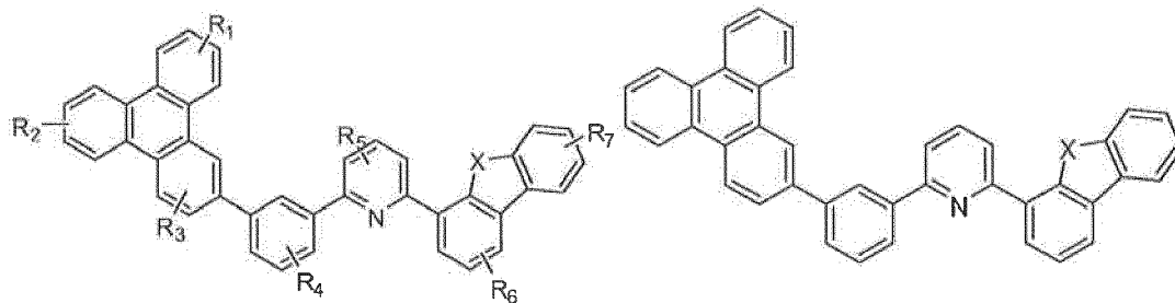
Compound 21
