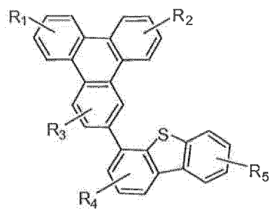
Compound 1'G
