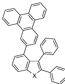
Compound 16
