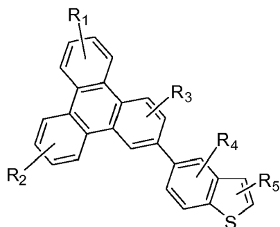
Compound 13'G
