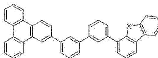
Compound 9
