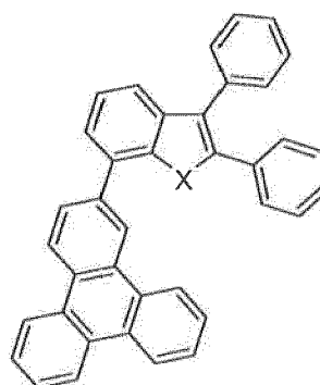
Compound 12
