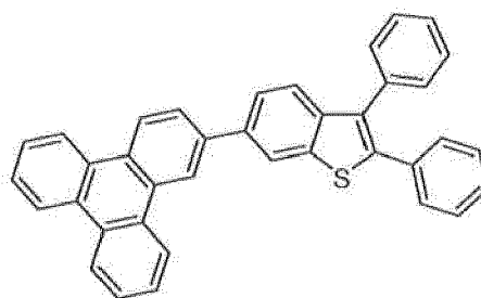
Compound 17'
