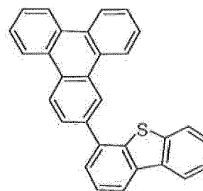
Compound 1'
