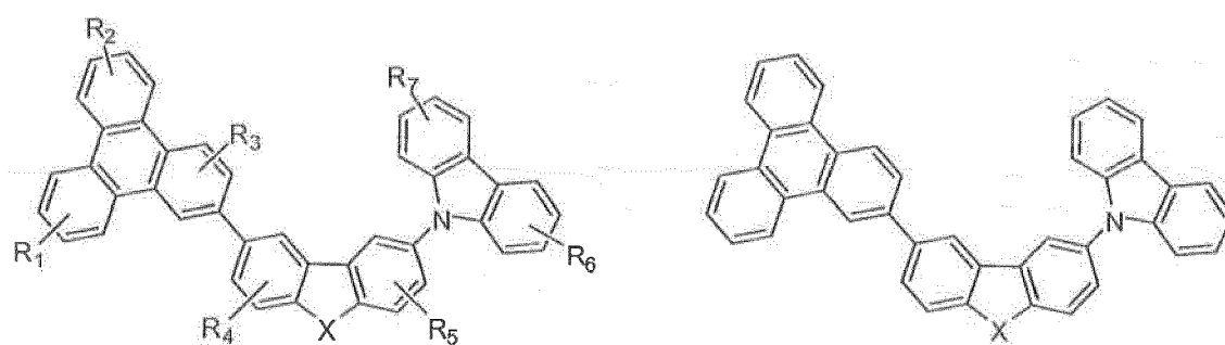
Compound 15G
