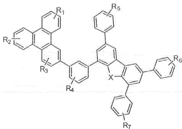
Compound 25 G
