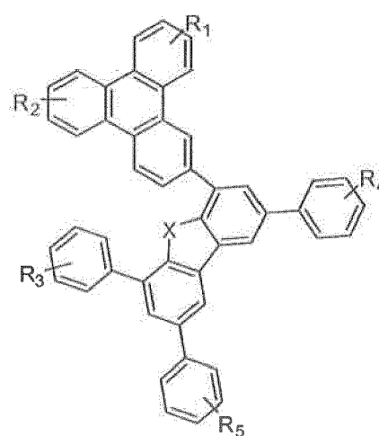
Compound 32G
