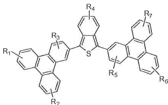
Compound 11'G
