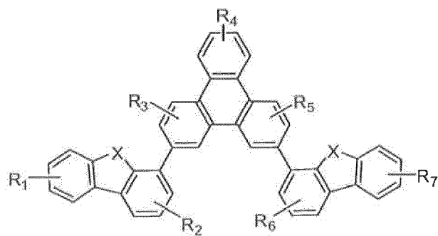
Compound 10G
