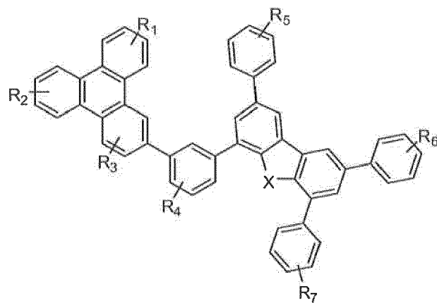
Compound 25 G
