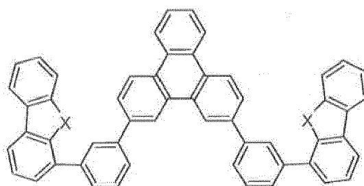
Compound 4
