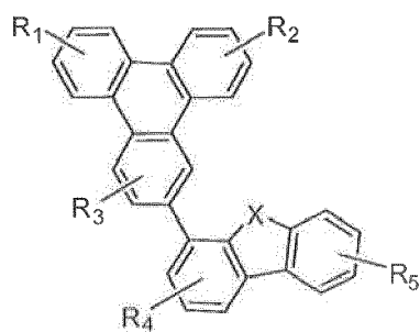
Compound 1G
