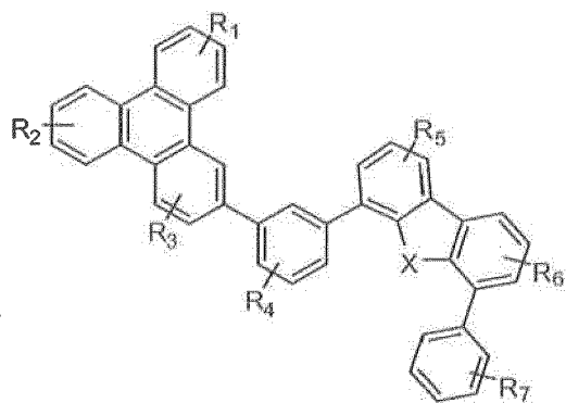
Compound 23 G
