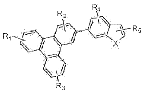
Compound 17G
