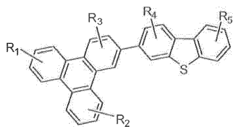
Compound 8'G
