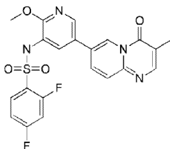
compound 81
