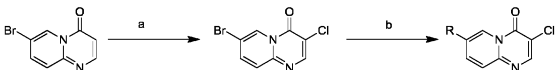
Scheme 13:
