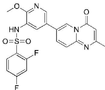
compound 221
