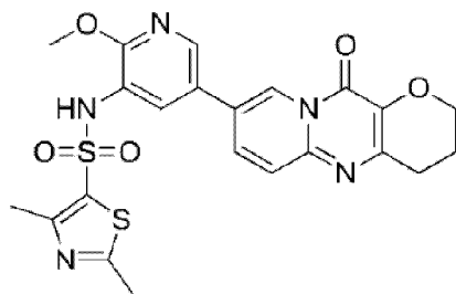
compound 240
