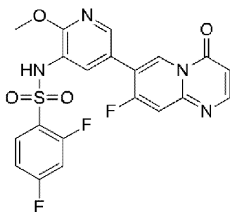
compound 112
