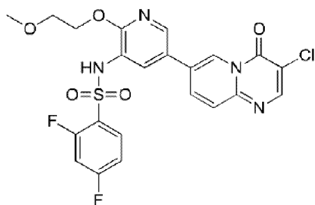
compound 231
