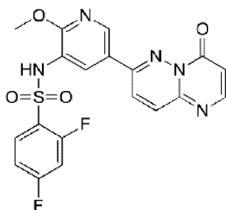
compound 71
