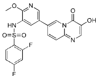
compound 101
