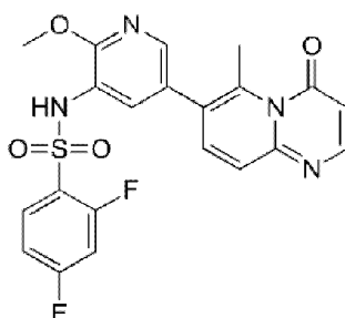
compound 52
