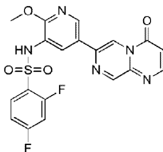
compound 39
