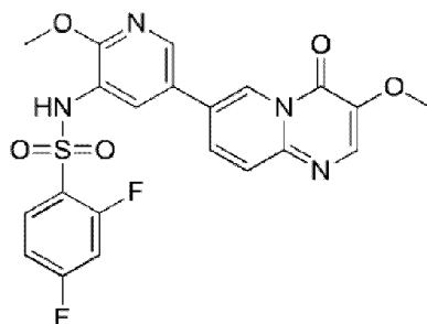
compound 103
