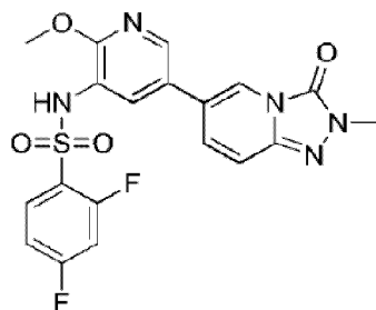
compound 234
