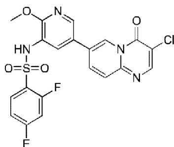
compound 132
