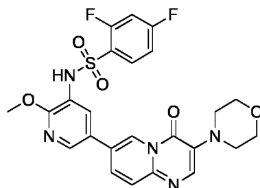
compound 241
