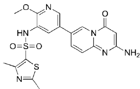
compound 236
