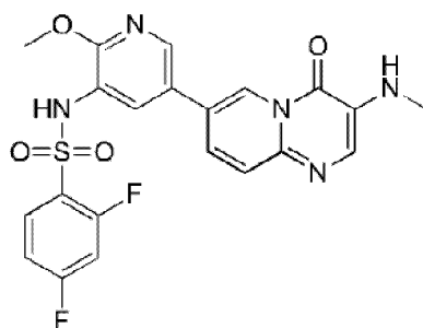
compound 95
