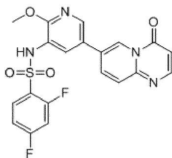
compound 1
