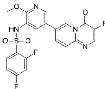
compound 61
