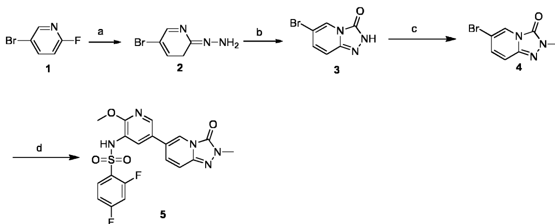
Scheme 19:
