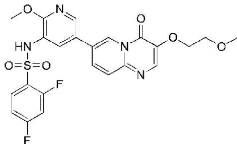
compound 175
