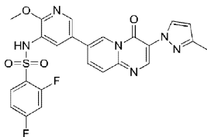
compound 216
