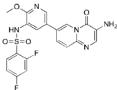
compound 87
