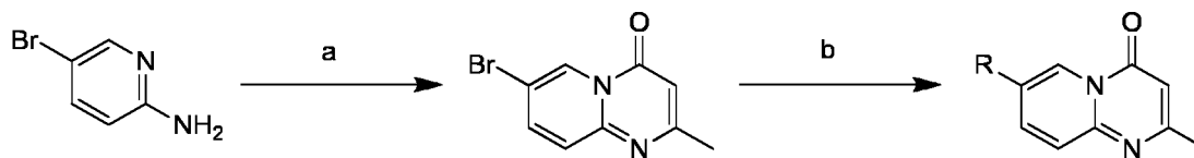
Scheme 17:
