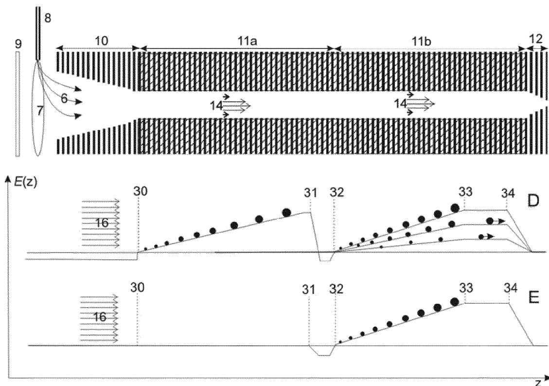
FIGURE 4 (PRIOR ART)
