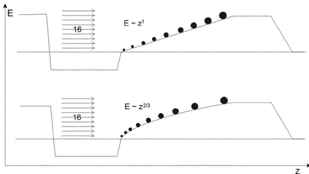
FIGURE 3 (PRIOR ART)
